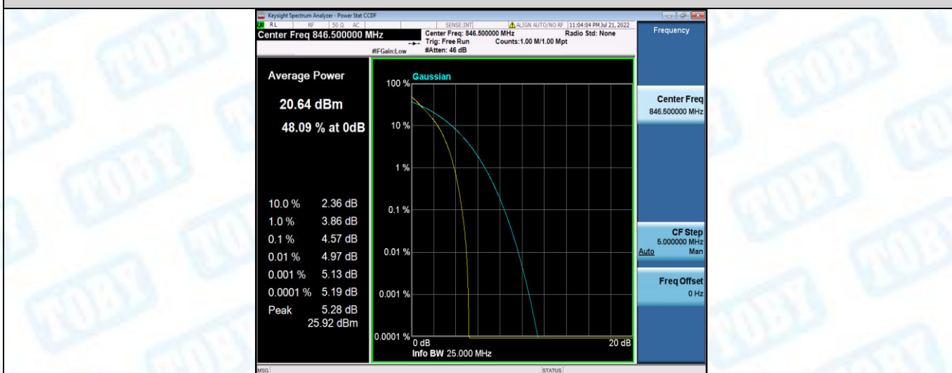
Band5-5MHz-16QAM-20425-1RB#0
