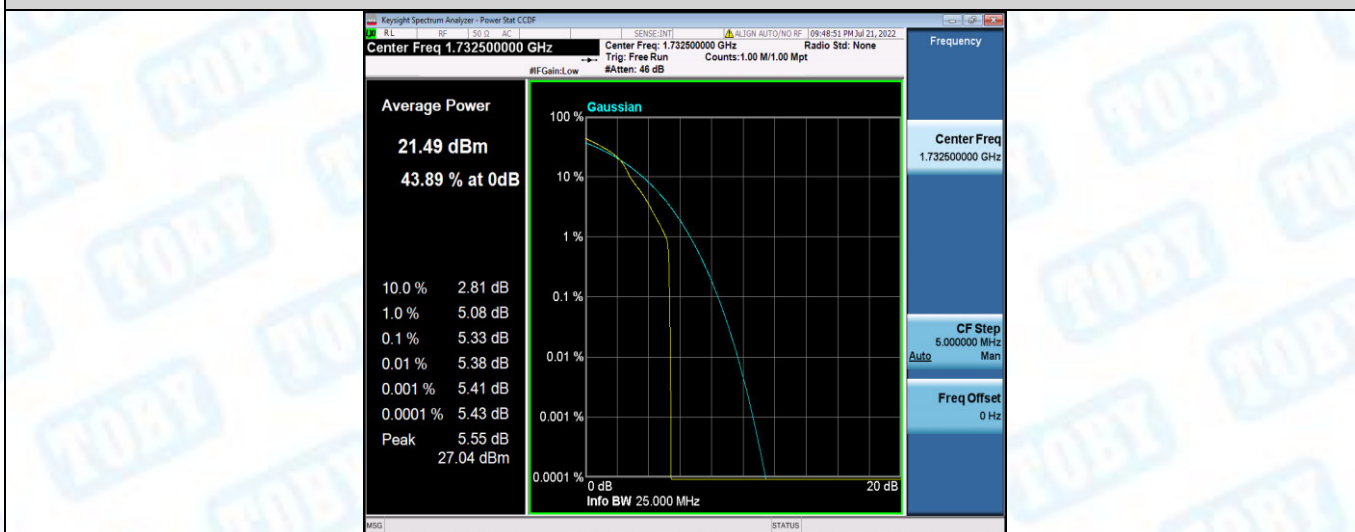
Band4-20MHz-16QAM-20175-100RB#0
