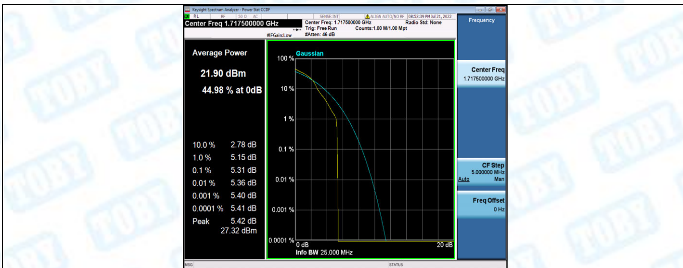
Band4-15MHz-16QAM-20025-75RB#0
