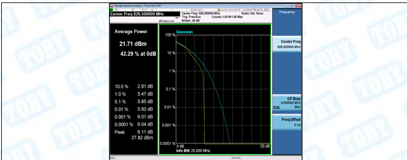
Band5-5MHz-16QAM-20425-25RB#0
