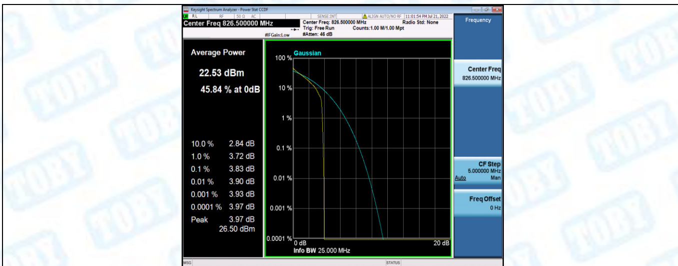
Band5-5MHz-QPSK-20425-25RB#0
