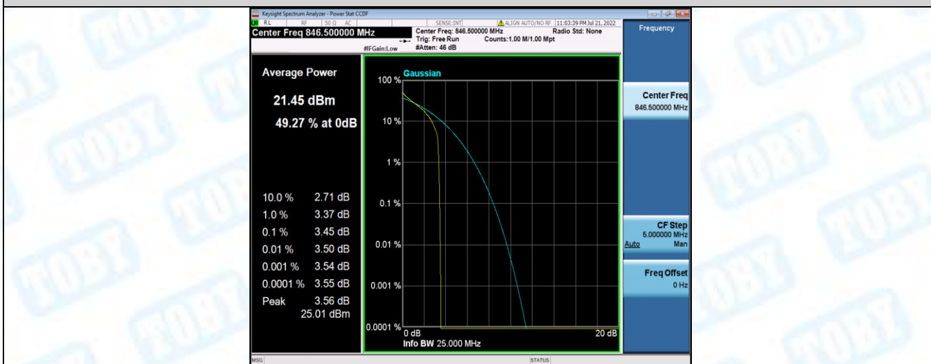
Band5-5MHz-QPSK-20625-25RB#0
