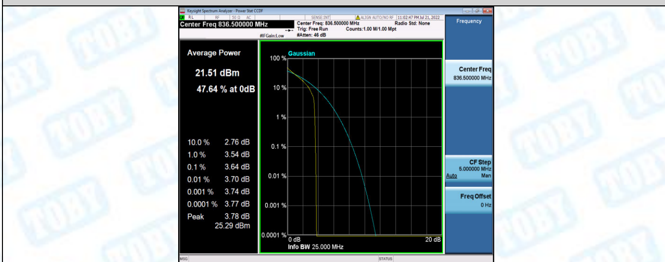
Band5-5MHz-QPSK-20525-25RB#0
