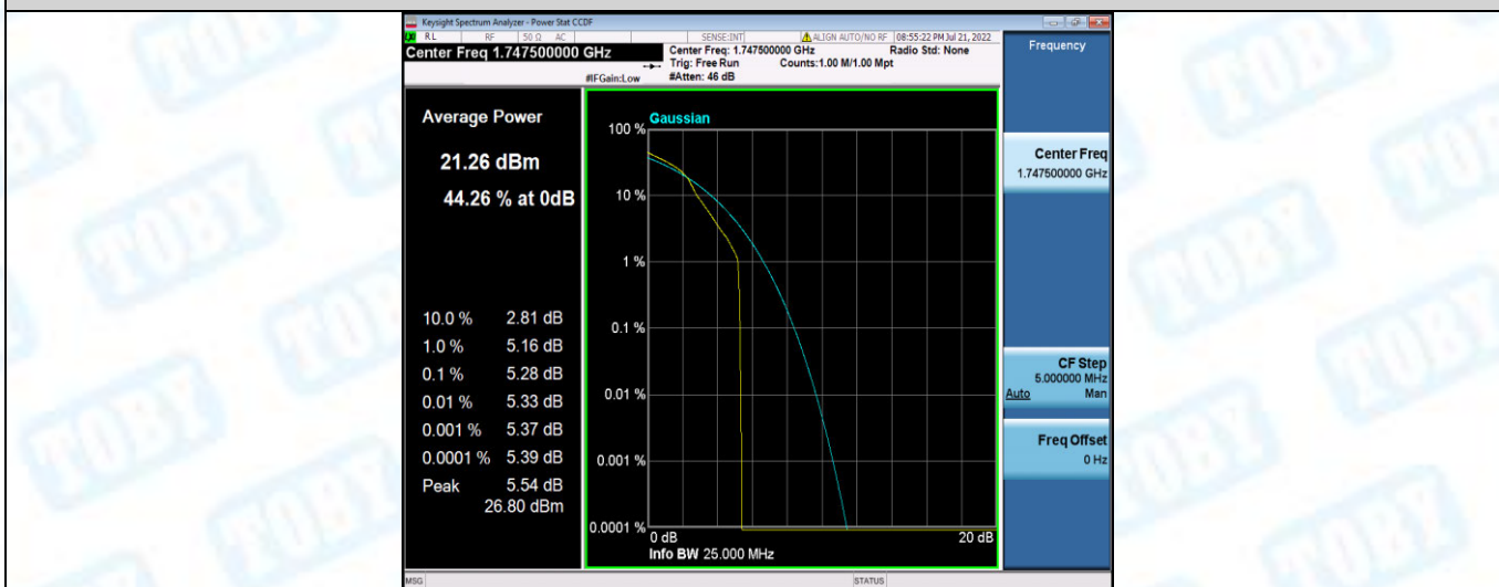
Band4-15MHz-16QAM-20325-75RB#0
