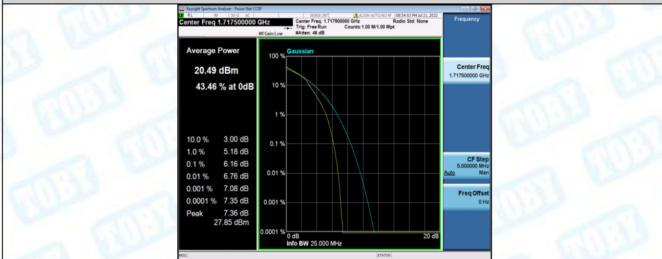
Band4-15MHz-16QAM-20175-1RB#0
