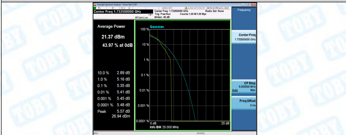
Band4-15MHz-16QAM-20175-75RB#0
