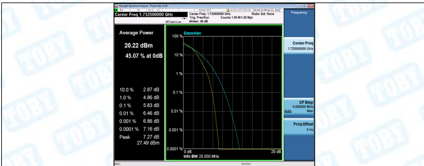
Band4-20MHz-16QAM-20300-1RB#0
