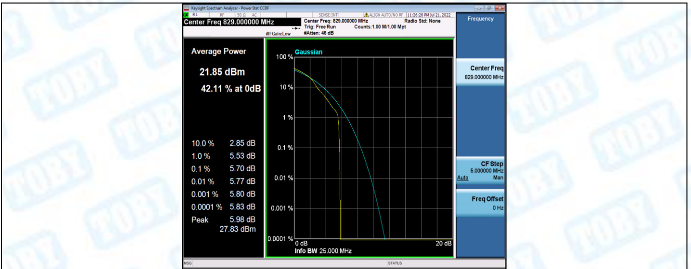
Band5-10MHz-16QAM-20450-50RB#0
