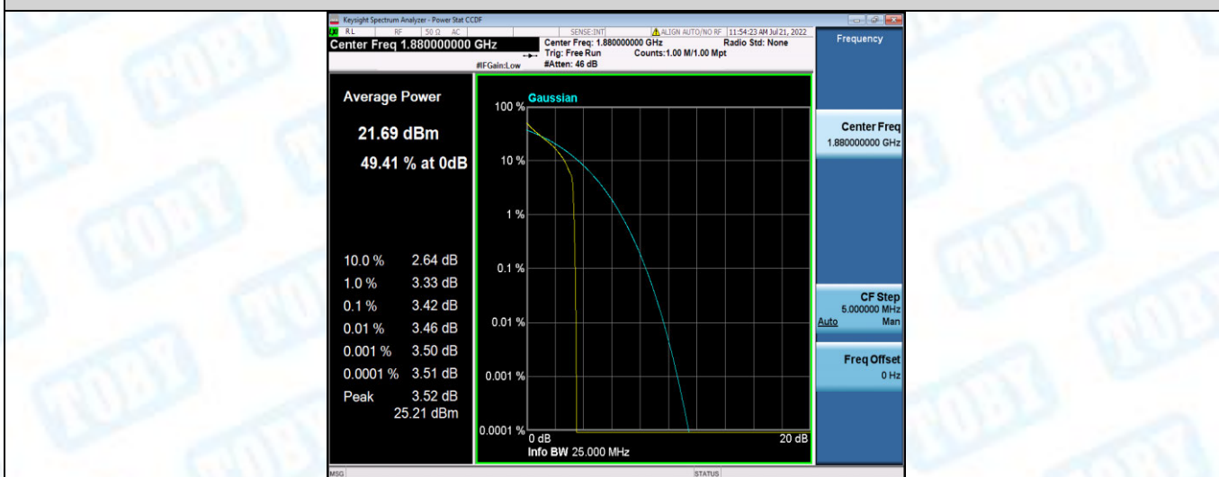
Band2-15MHz-QPSK-18900-75RB#0
