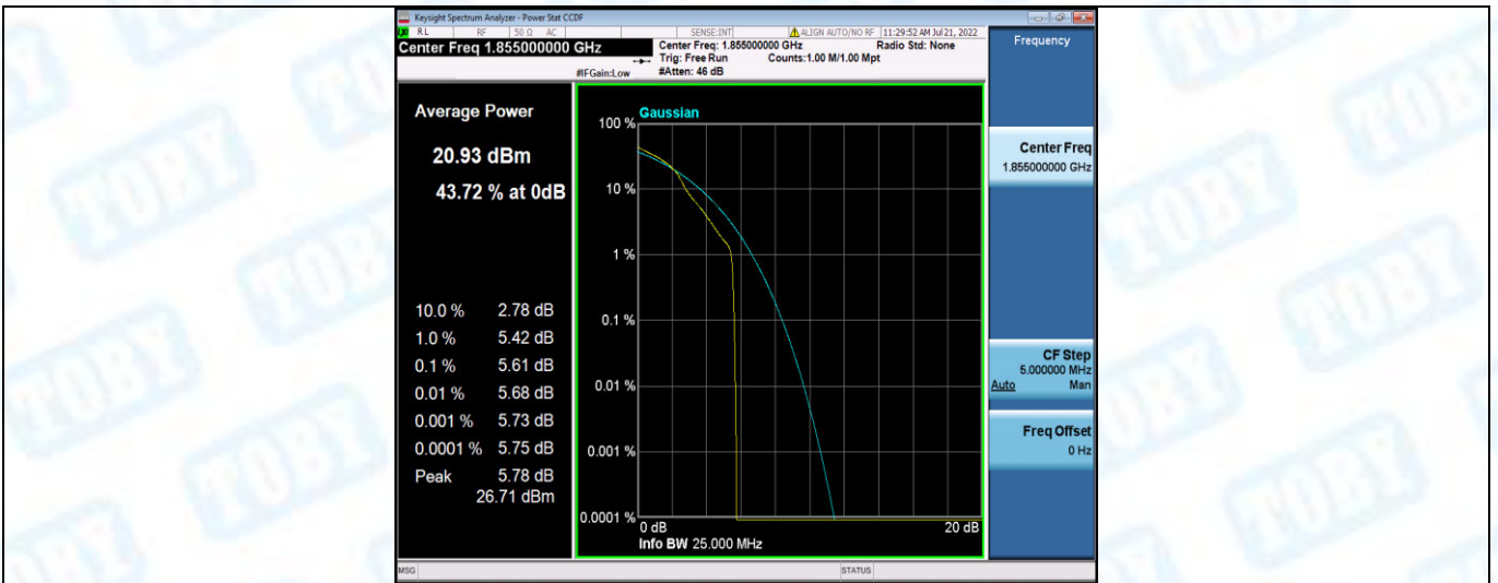
Band2-10MHz-16QAM-18650-50RB#0
