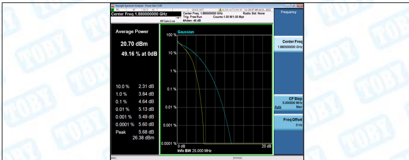
Band2-10MHz-QPSK-19150-1RB#0
