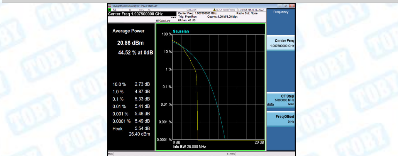
Band2-5MHz-16QAM-19175-25RB#0
