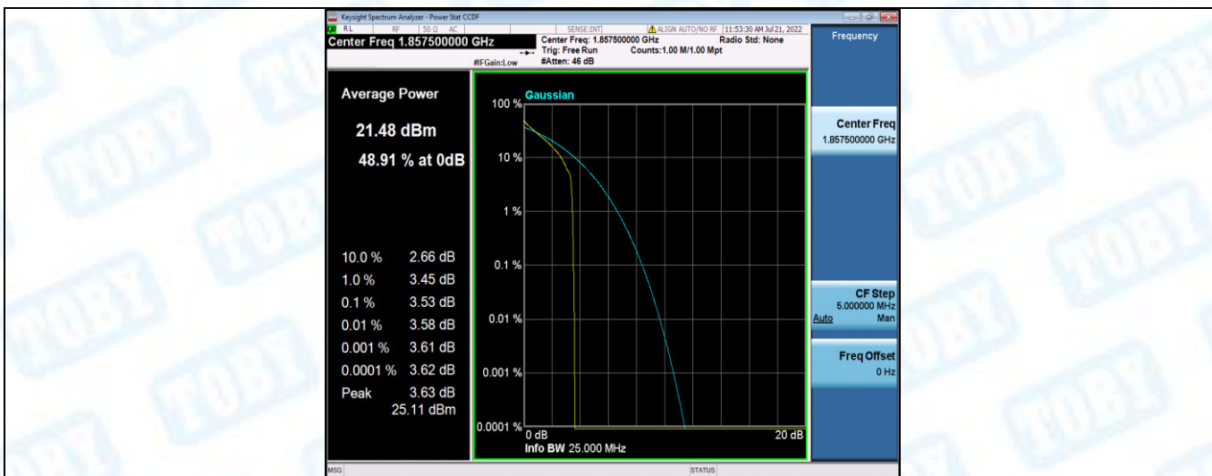
Band2-15MHz-QPSK-18675-75RB#0
