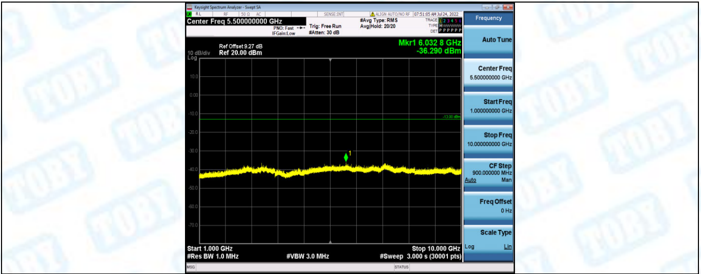
Band5-4183-3-1000~10000MHz
