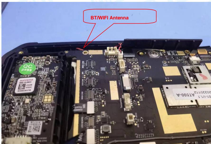
Photo 13 Internal of EUT (SINGLE)
