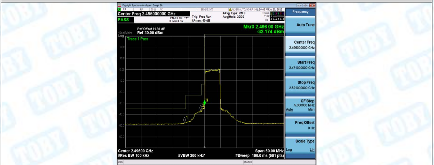
Band41-5MHz-16QAM-41565-1RB#0
