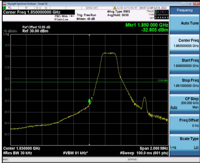
Band25-1.4MHz-16QAM-26047-1RB#5
