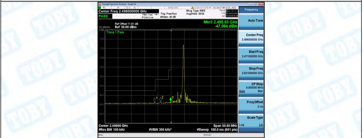
Band41-5MHz-16QAM-39675-25RB#0
