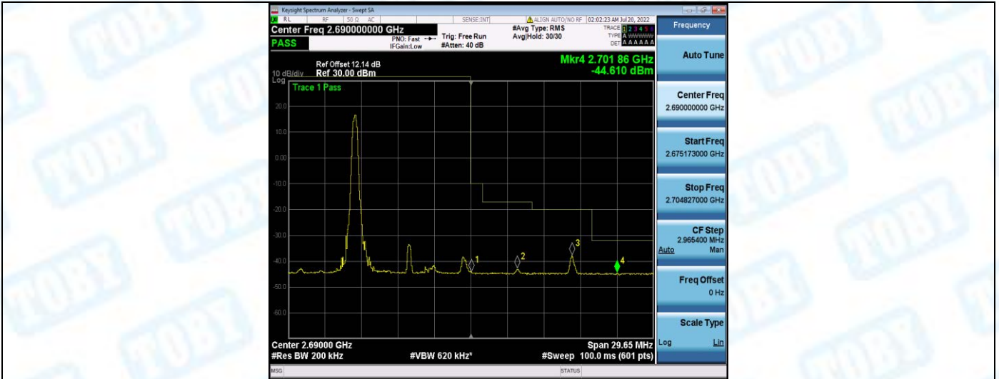
Band41-10MHz-QPSK-41540-1RB#49
