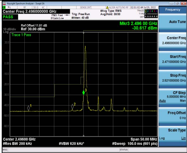
Band41-10MHz-QPSK-39700-1RB#49
