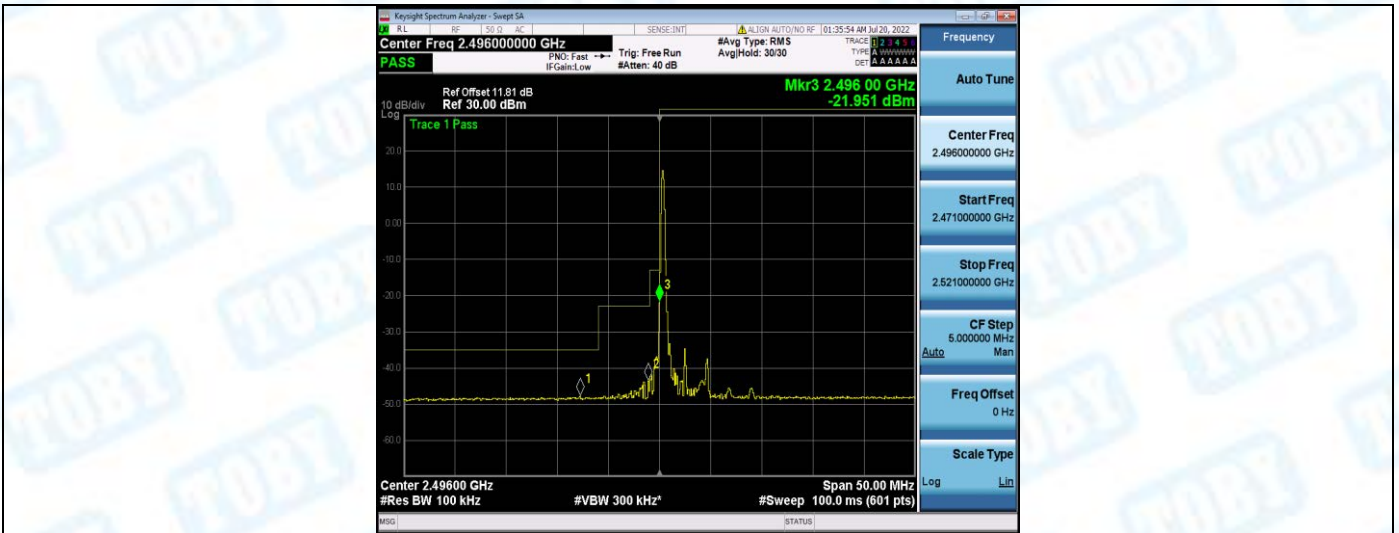
Band41-5MHz-QPSK-39675-1RB#24
