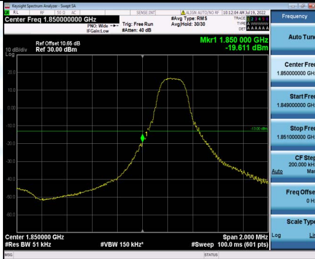
Band25-3MHz-QPSK-26055-1RB#14
