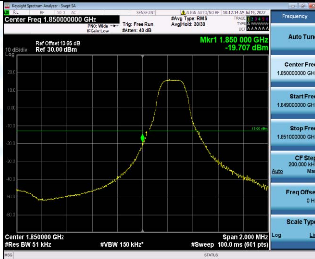
Band25-3MHz-16QAM-26055-1RB#14
