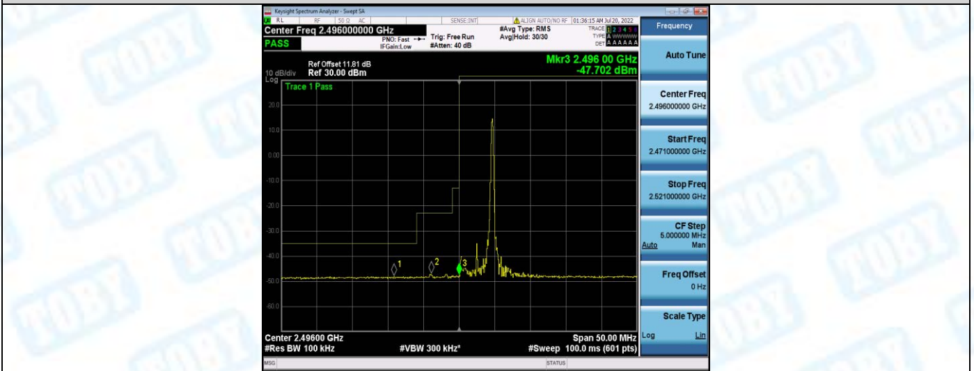
Band41-5MHz-QPSK-39675-25RB#0
