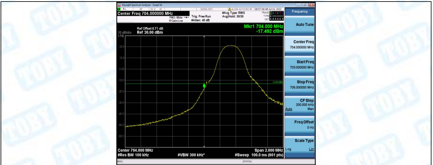
Band17-5MHz-QPSK-23755-1RB#24
