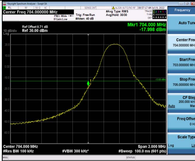
Band17-5MHz-16QAM-23755-1RB#24
