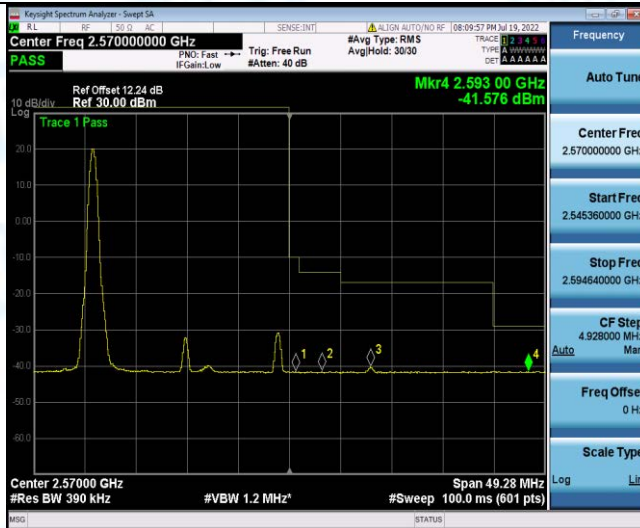
Band7-20MHz-16QAM-21350-1RB#99
