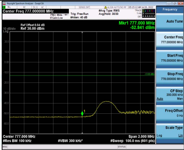
Band13-5MHz-16QAM-23205-25RB#0
