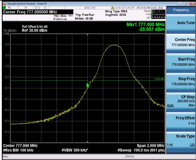
Band13-5MHz-16QAM-23205-1RB#24
