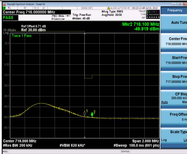
Band17-10MHz-QPSK-23800-1RB#49
