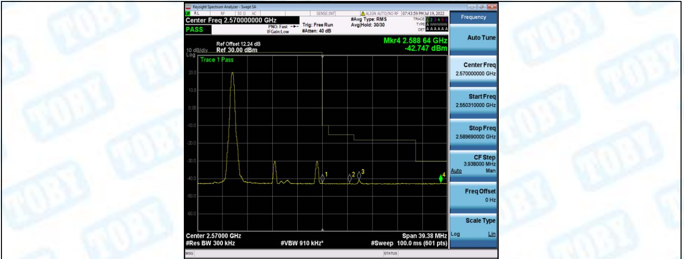
Band7-15MHz-16QAM-21375-1RB#74
