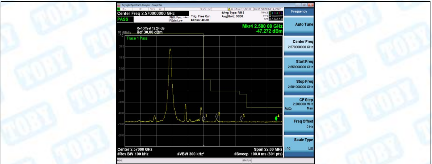
Band7-5MHz-16QAM-21425-1RB#24
