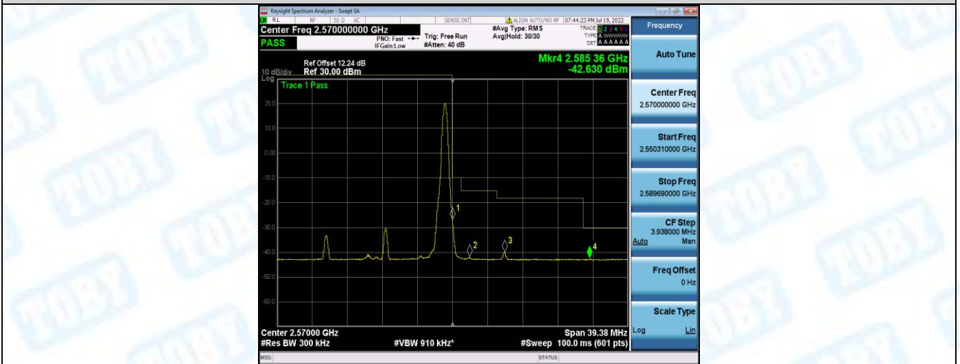
Band7-15MHz-16QAM-21375-75RB#0
