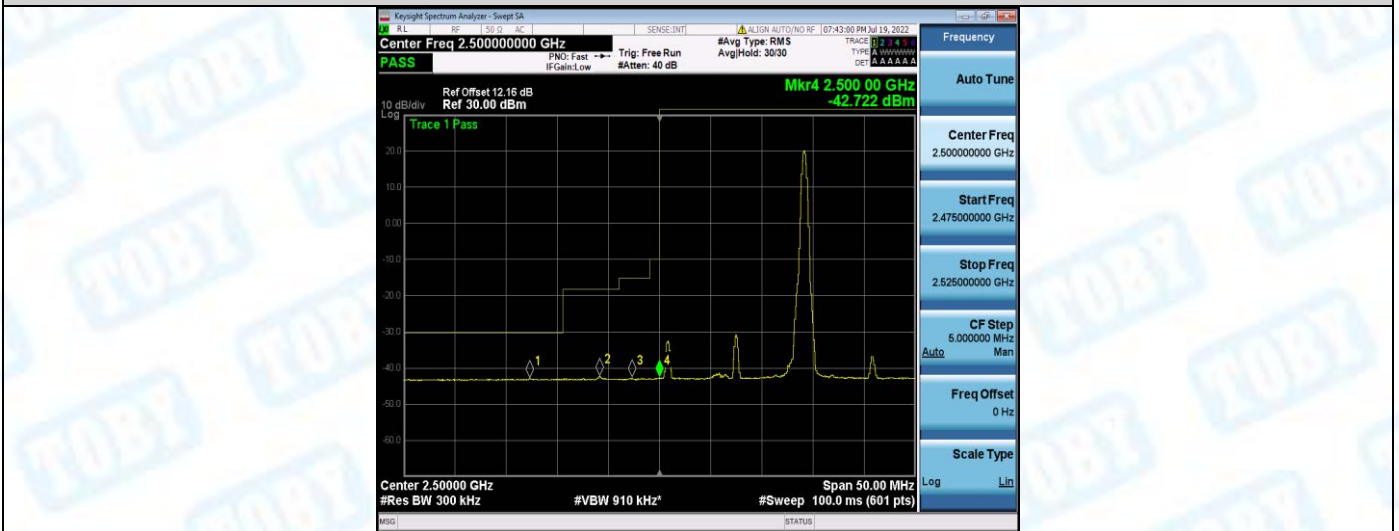
Band7-15MHz-16QAM-20825-75RB#0
