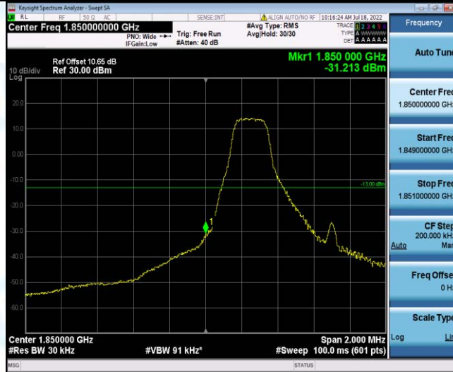
Band2-1.4MHz-QPSK-18607-1RB#5
