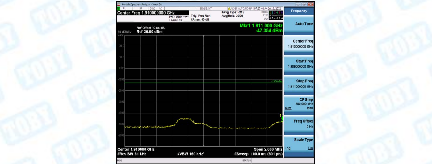
Band2-3MHz-16QAM-19185-1RB#14
