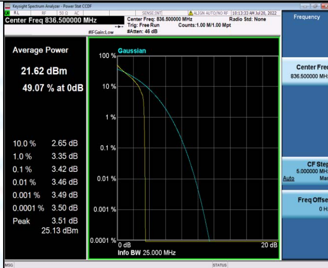
Band26-10MHz-QPSK-26915-50RB#0
