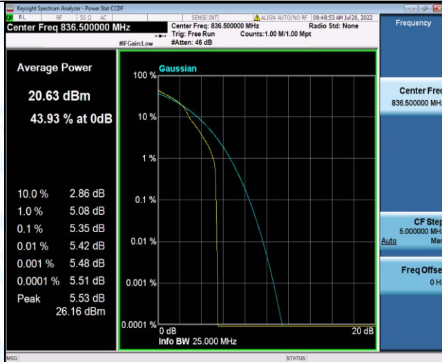
Band26-5MHz-16QAM-26915-25RB#0
