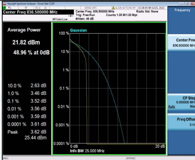
Band26-15MHz-QPSK-26915-75RB#0
