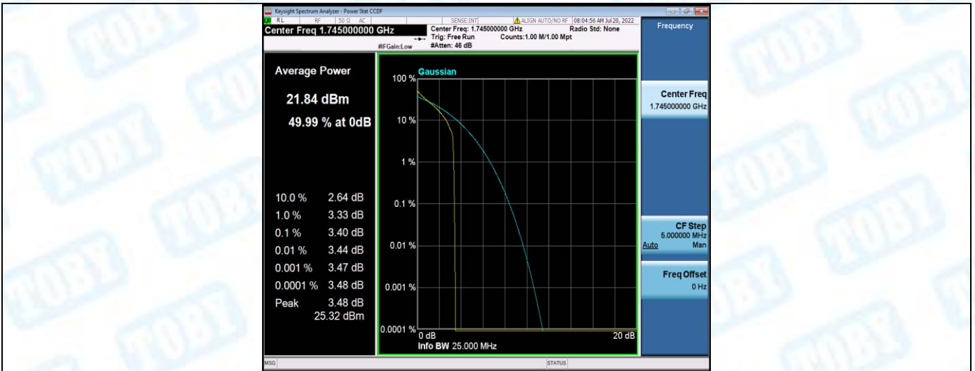
Band66-10MHz-QPSK-132322-50RB#0
