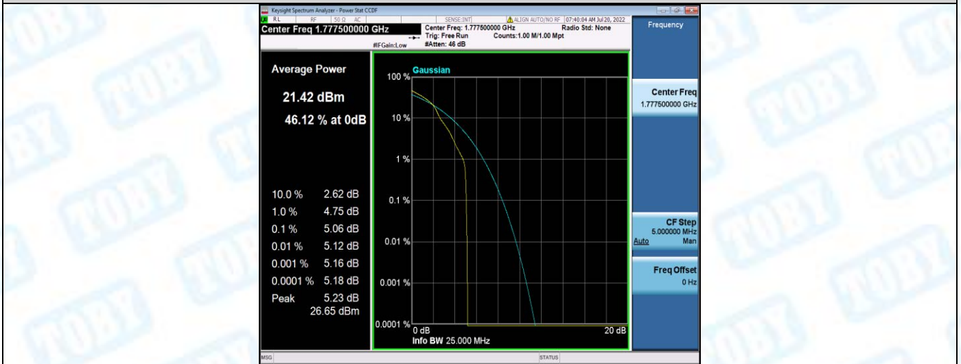
Band66-5MHz-16QAM-132647-25RB#0
