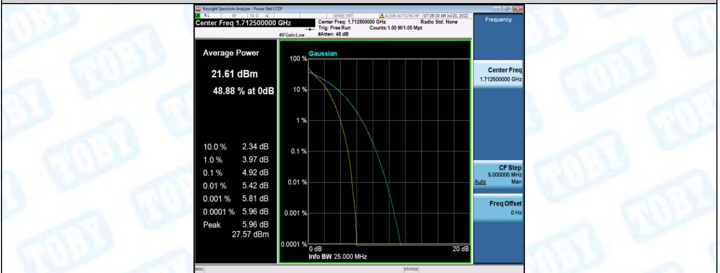
Band66-5MHz-QPSK-132322-1RB#0
