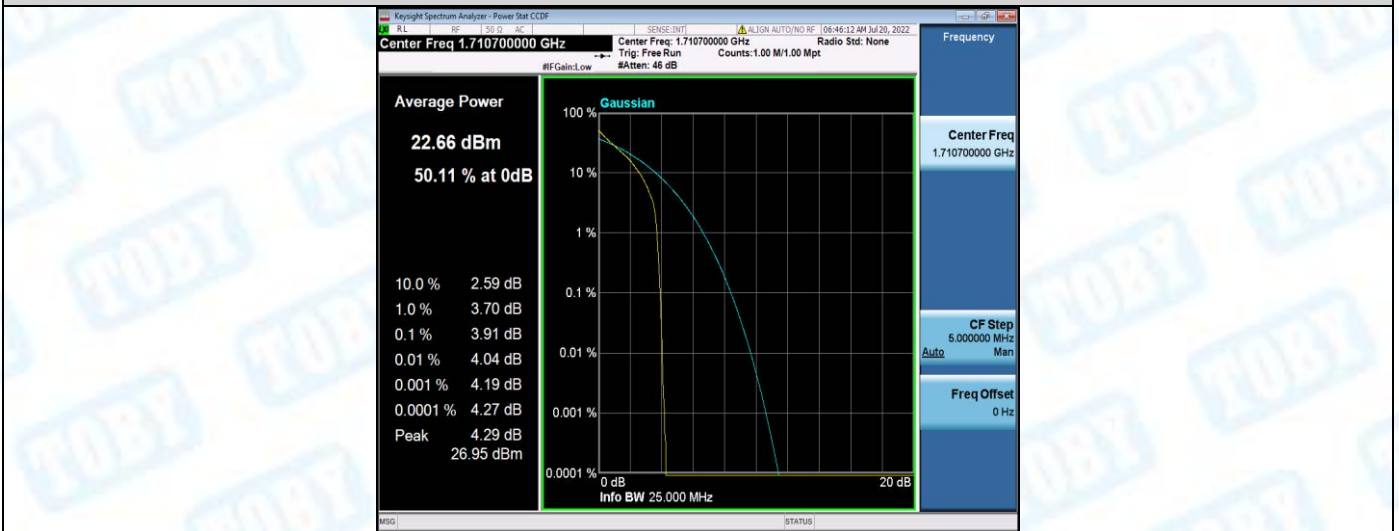
Band66-1.4MHz-QPSK-131979-6RB#0
