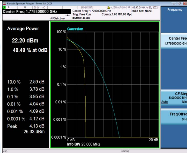
Band66-1.4MHz-QPSK-132665-6RB#0
