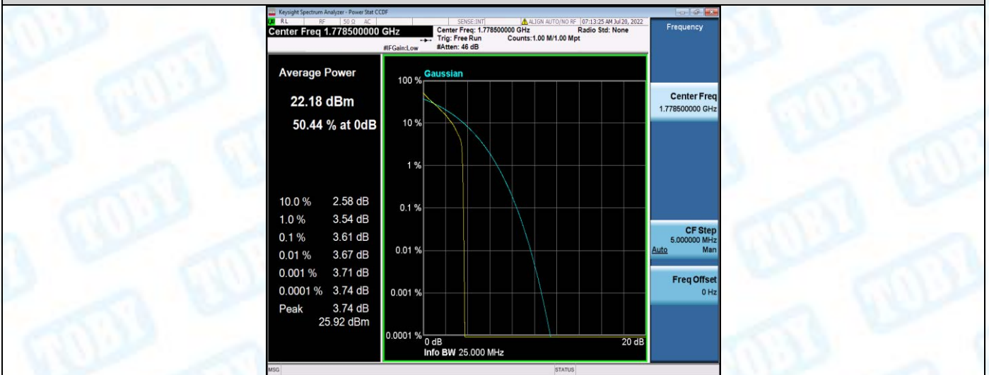
Band66-3MHz-QPSK-132657-15RB#0
