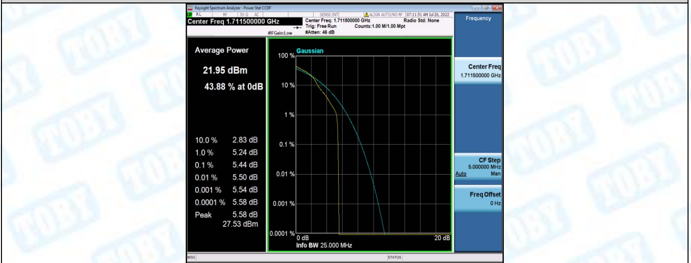
Band66-3MHz-16QAM-131987-15RB#0
