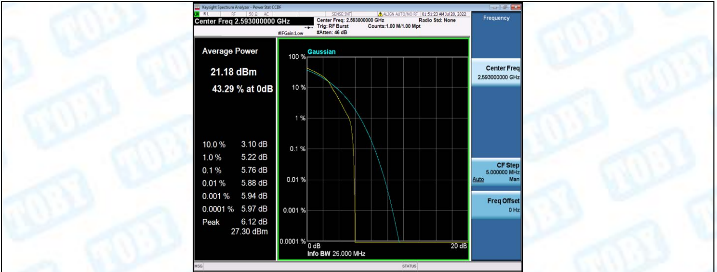
Band41-5MHz-16QAM-40620-25RB#0
