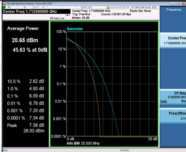
Band66-5MHz-16QAM-132322-1RB#0
