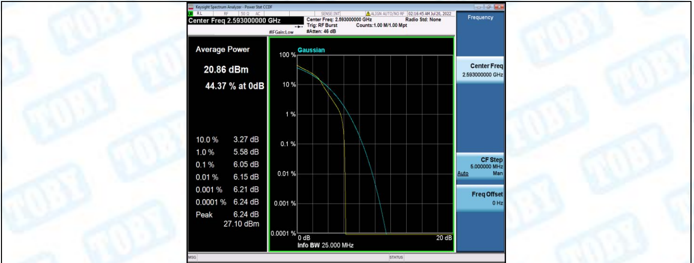
Band41-10MHz-16QAM-40620-50RB#0
