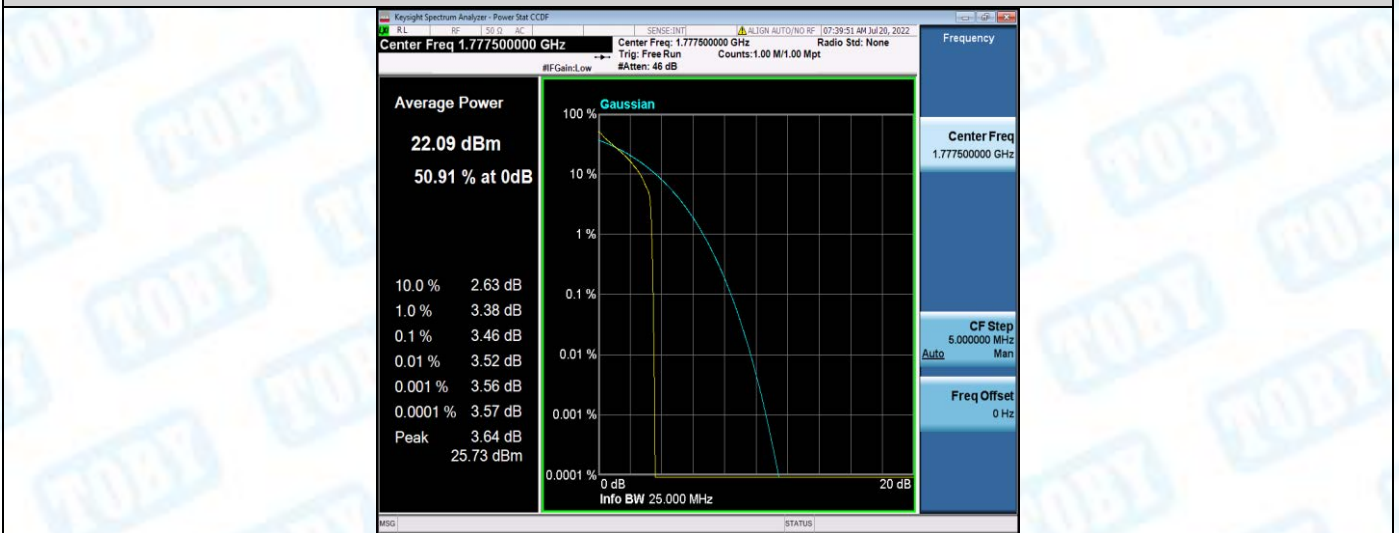
Band66-5MHz-QPSK-132647-25RB#0
