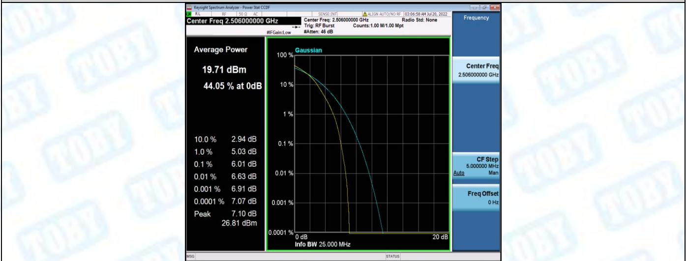
Band41-20MHz-16QAM-40620-1RB#0
