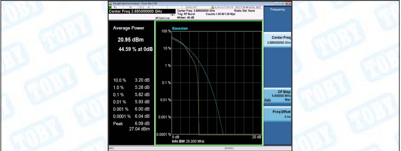
Band41-10MHz-16QAM-41540-50RB#0
