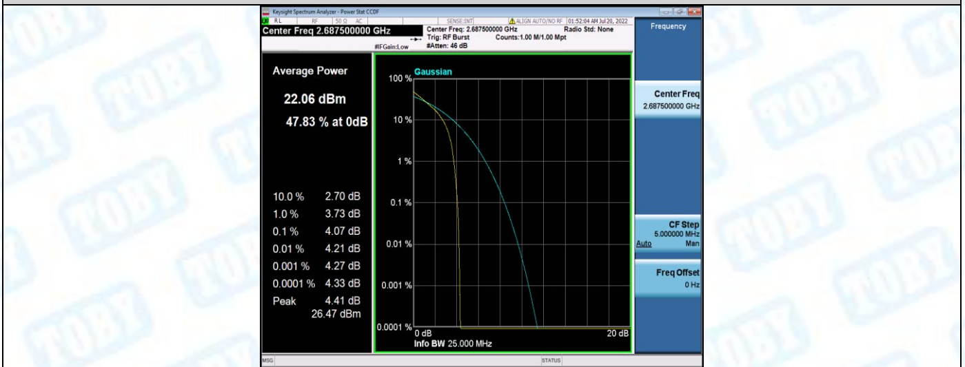
Band41-5MHz-QPSK-41565-25RB#0
