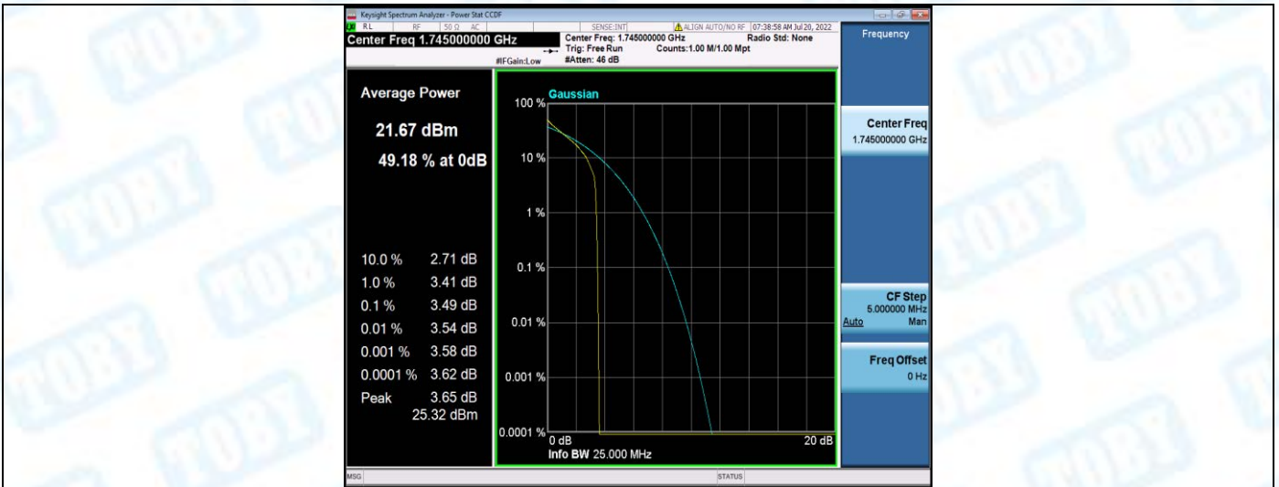
Band66-5MHz-QPSK-132322-25RB#0
