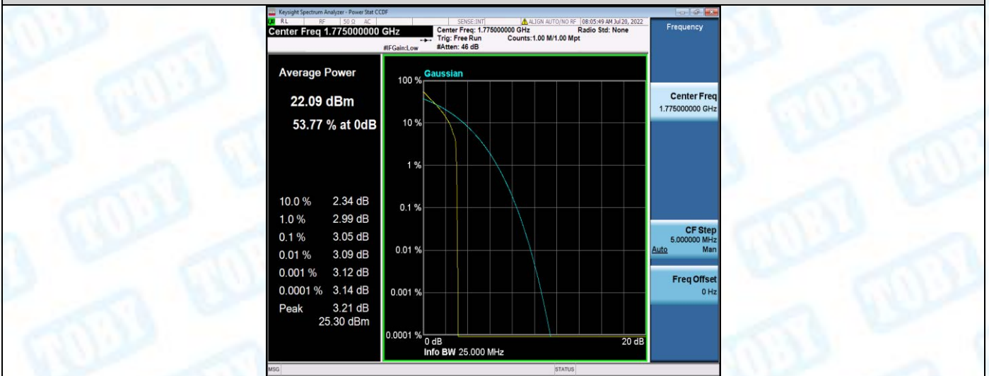
Band66-10MHz-QPSK-132622-50RB#0
