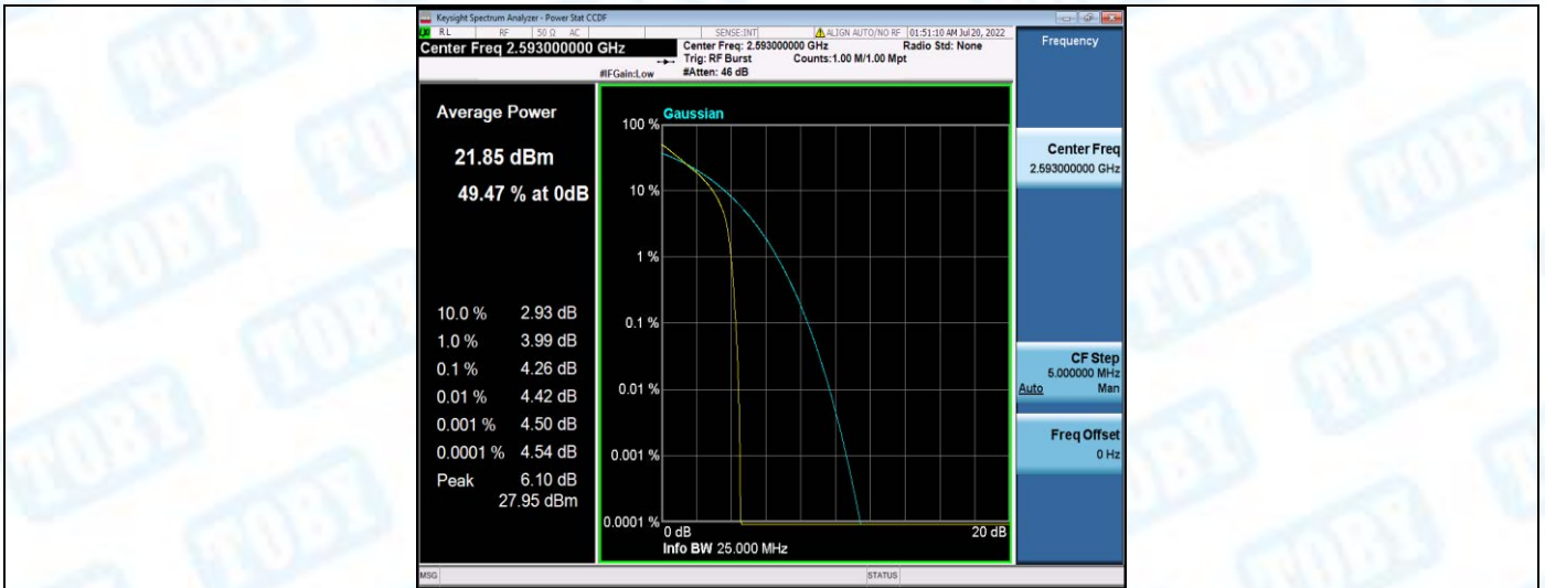
Band41-5MHz-QPSK-40620-25RB#0
