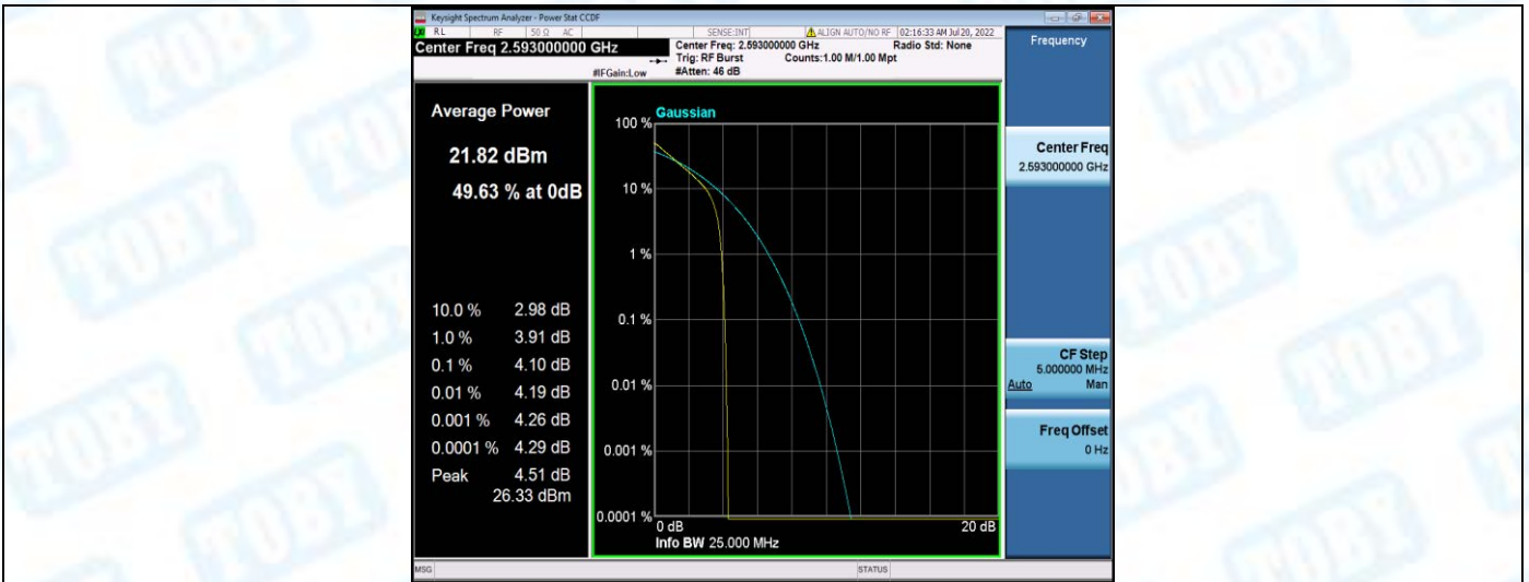
Band41-10MHz-QPSK-40620-50RB#0
