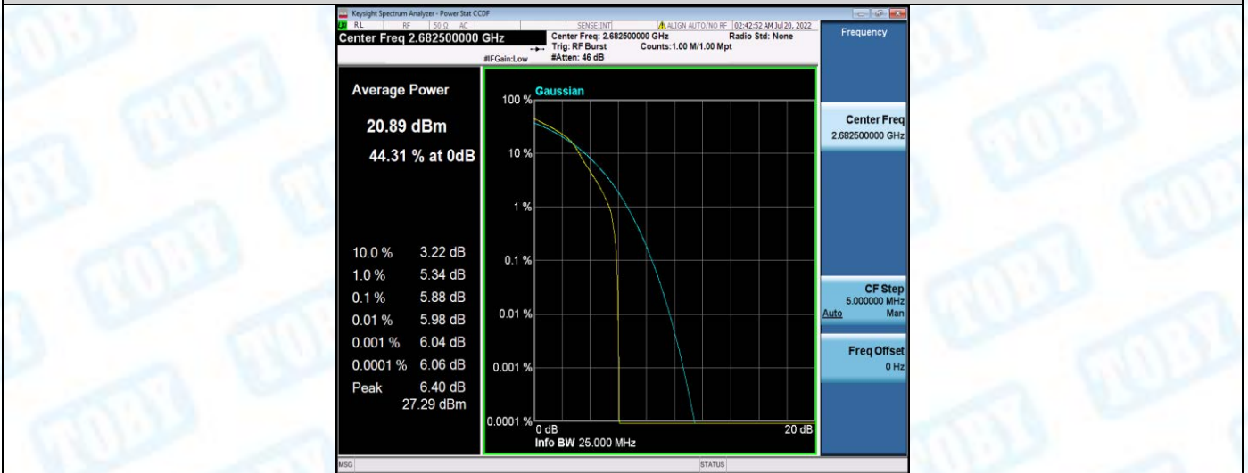
Band41-15MHz-16QAM-41515-75RB#0
