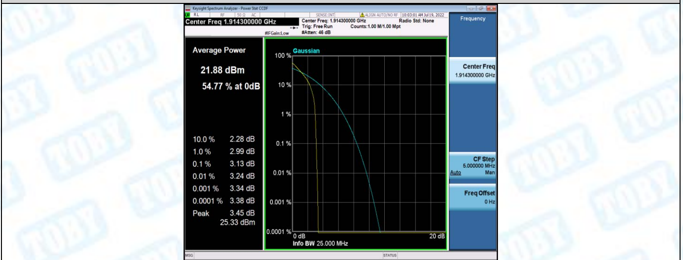
Band25-1.4MHz-QPSK-26683-6RB#0
