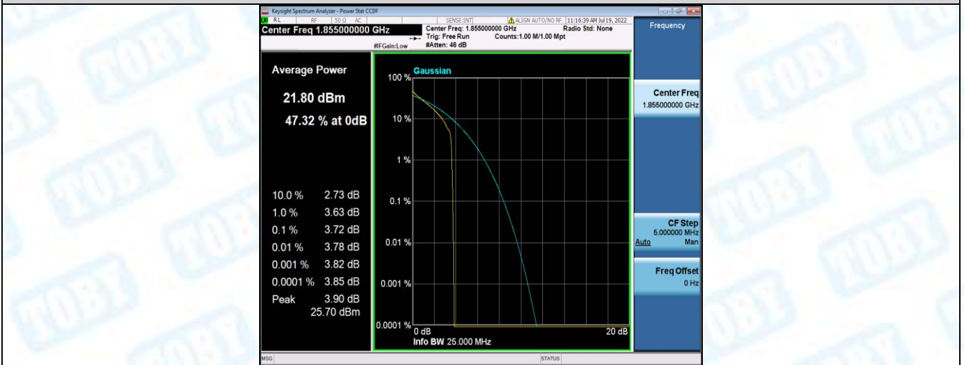
Band25-10MHz-QPSK-26090-50RB#0
