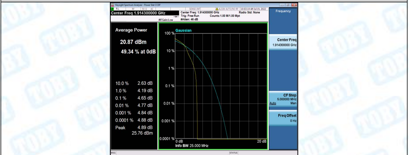
Band25-1.4MHz-16QAM-26683-6RB#0
