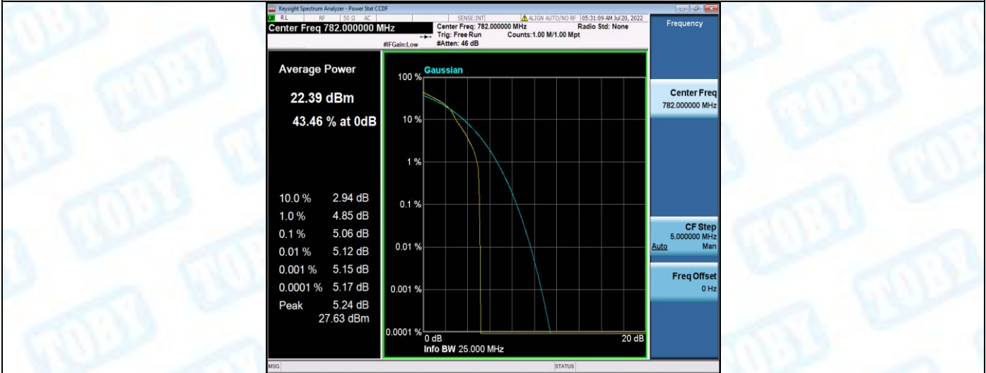
Band13-5MHz-16QAM-23230-25RB#0
