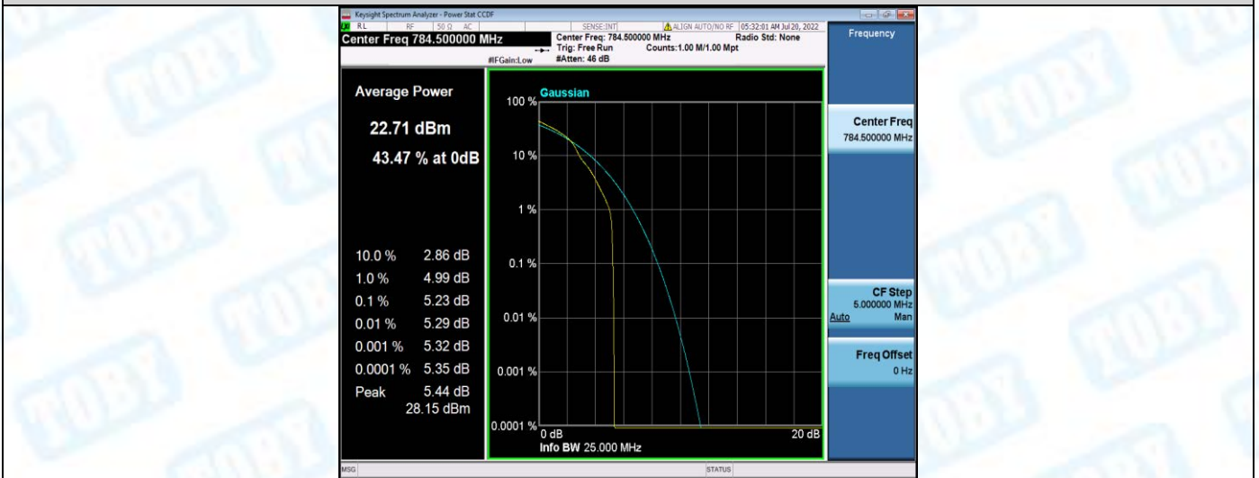
Band13-5MHz-16QAM-23255-25RB#0
