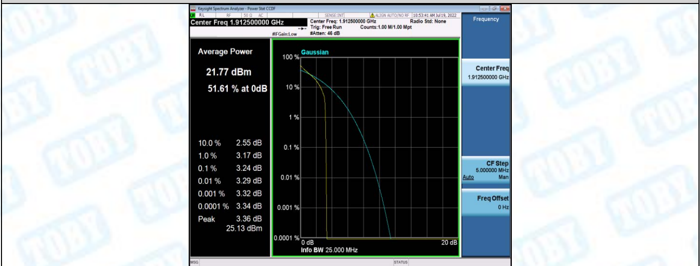
Band25-5MHz-QPSK-26665-25RB#0
