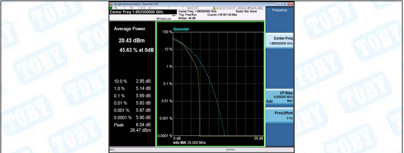
Band25-1.4MHz-16QAM-26365-6RB#0
