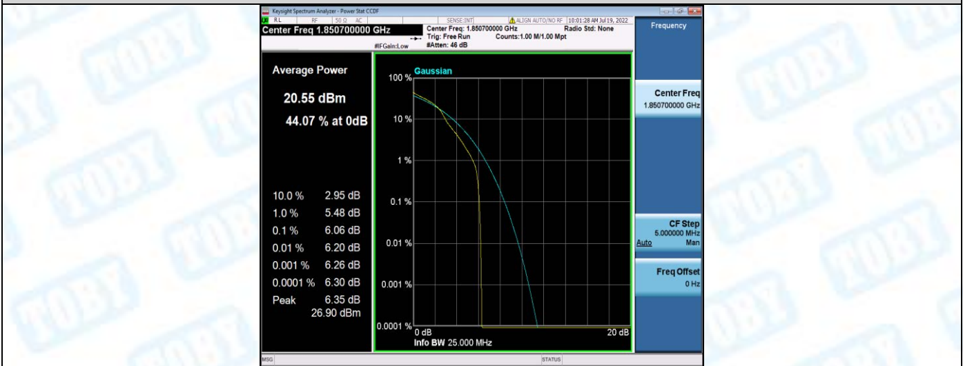
Band25-1.4MHz-16QAM-26047-6RB#0
