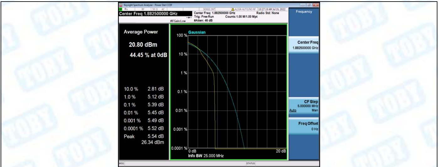
Band25-3MHz-16QAM-26365-15RB#0
