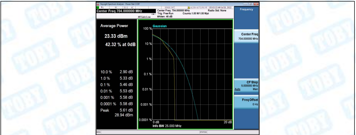
Band12-10MHz-16QAM-23060-50RB#0
