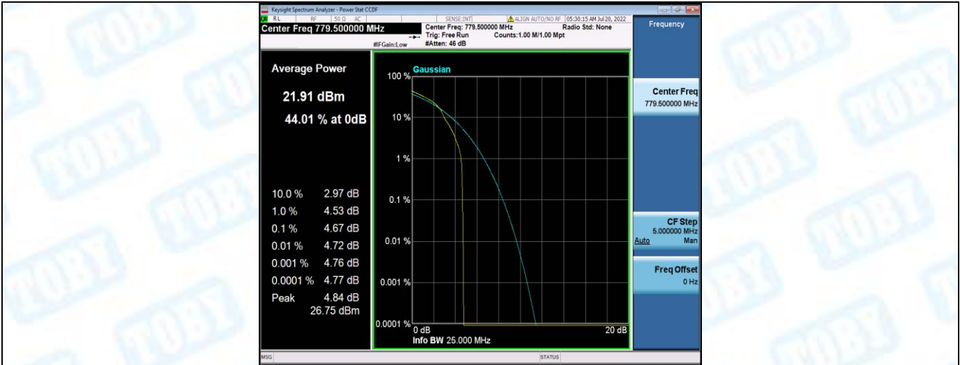
Band13-5MHz-16QAM-23205-25RB#0
