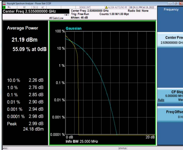
Band7-20MHz-QPSK-21100-100RB#0
