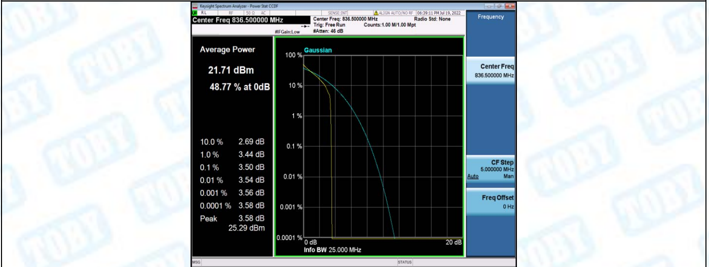
Band5-10MHz-QPSK-20525-50RB#0
