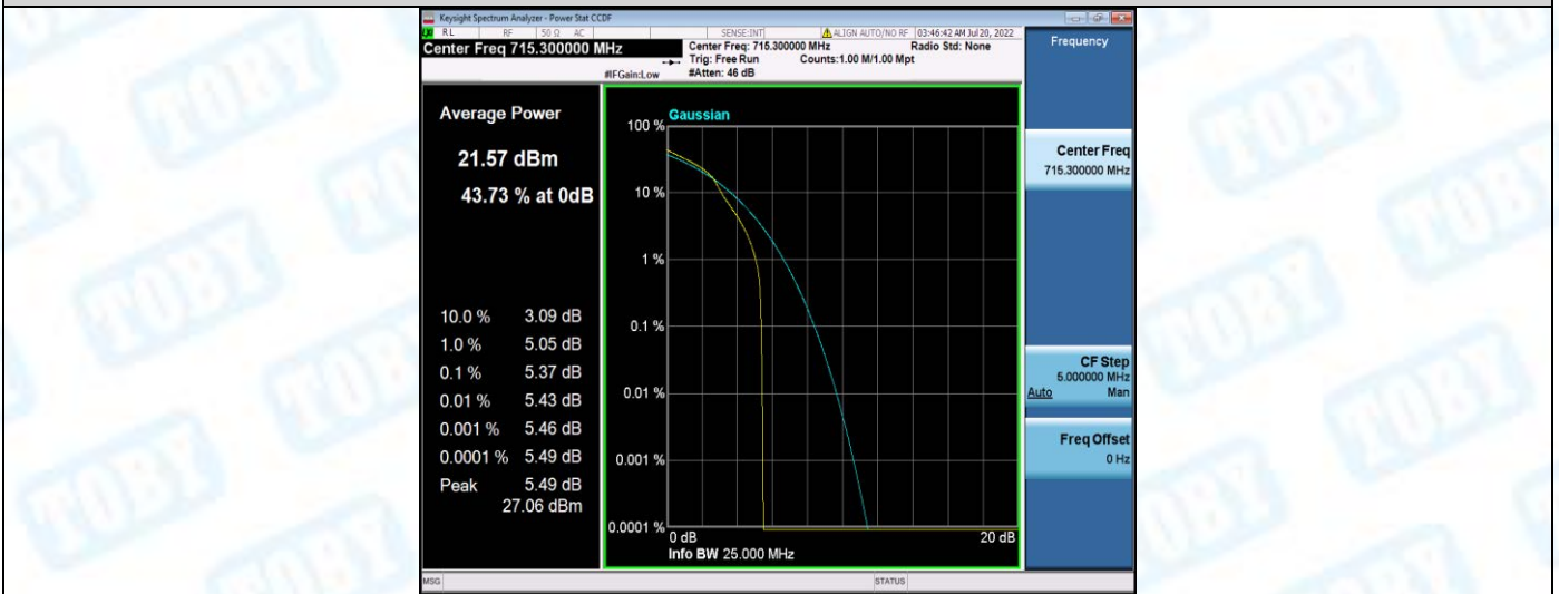
Band12-1.4MHz-16QAM-23173-6RB#0
