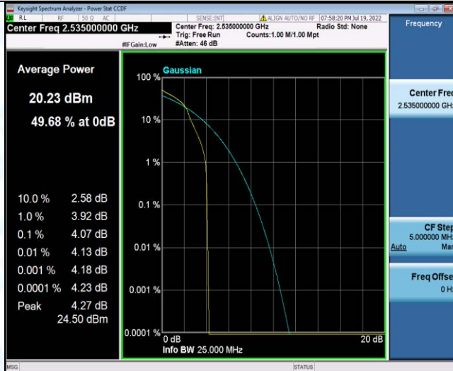
Band7-15MHz-16QAM-21100-75RB#0
