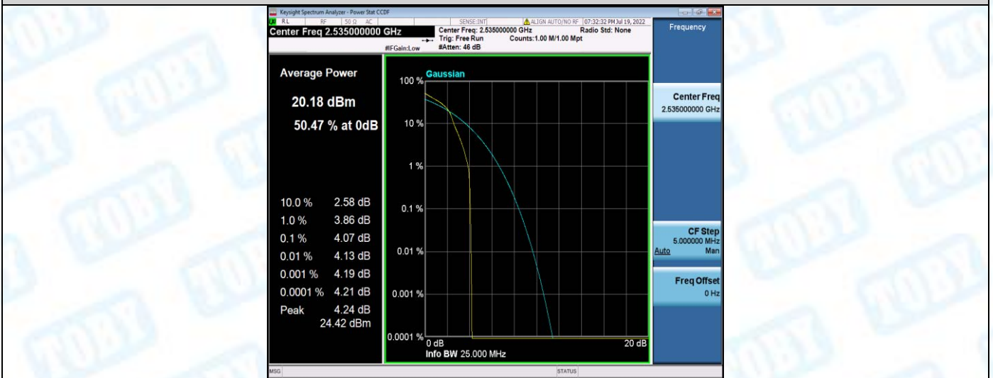
Band7-10MHz-16QAM-21100-50RB#0
