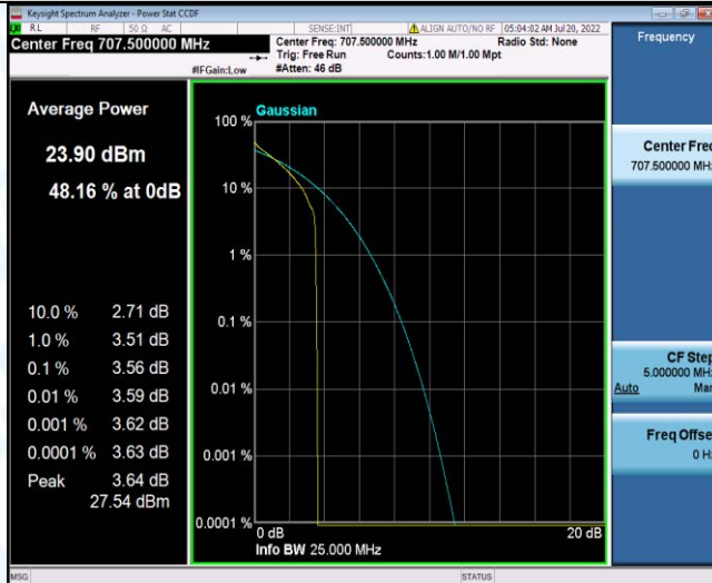
Band12-10MHz-QPSK-23095-50RB#0
