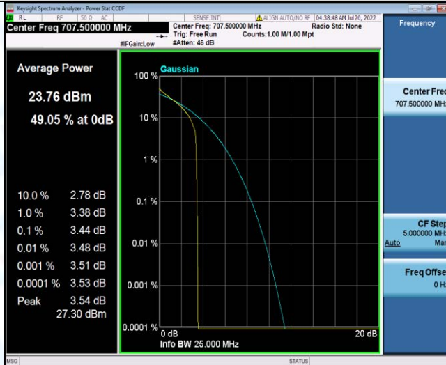
Band12-5MHz-QPSK-23095-25RB#0
