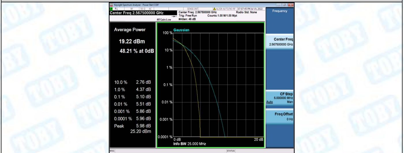
Band7-10MHz-QPSK-20800-1RB#0
