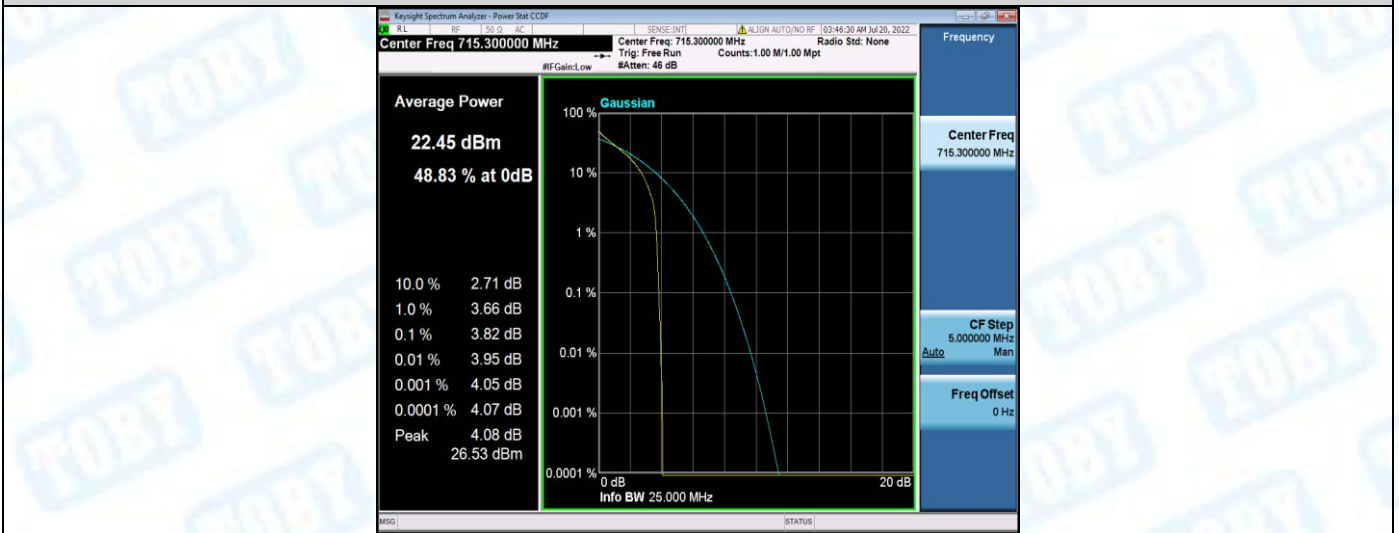
Band12-1.4MHz-QPSK-23173-6RB#0
