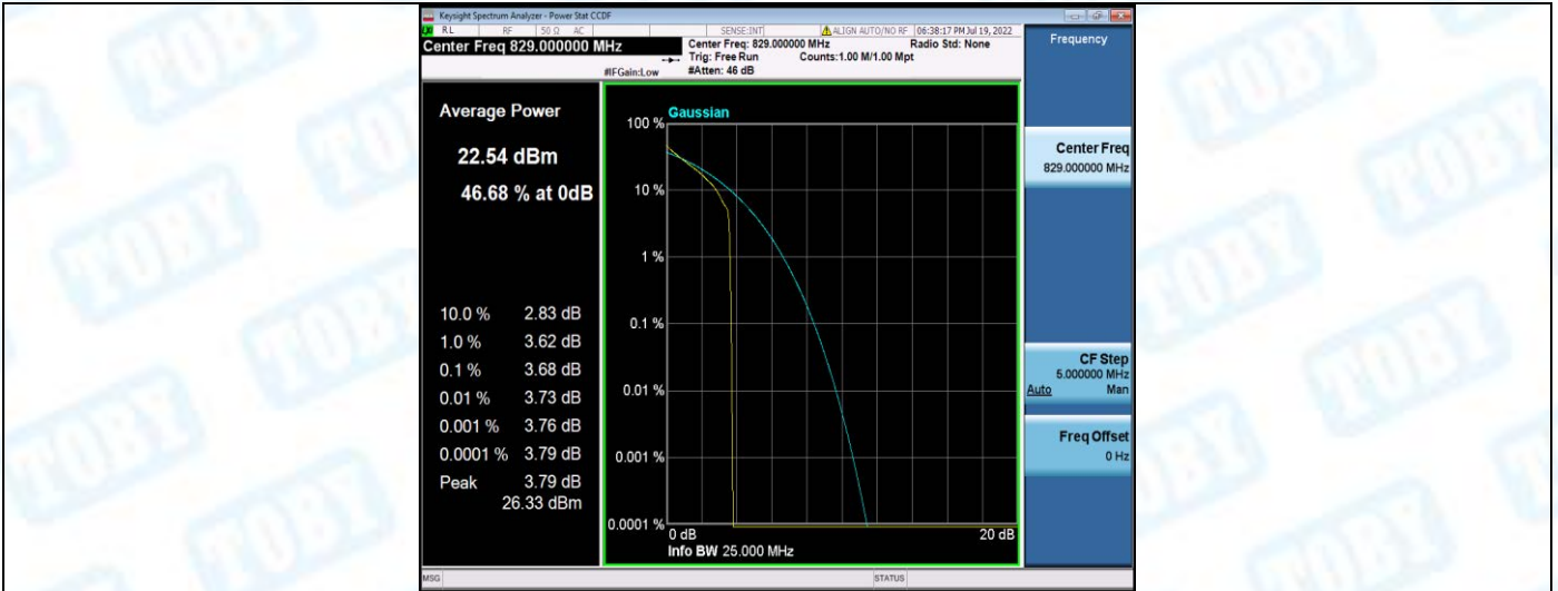
Band5-10MHz-QPSK-20450-50RB#0
