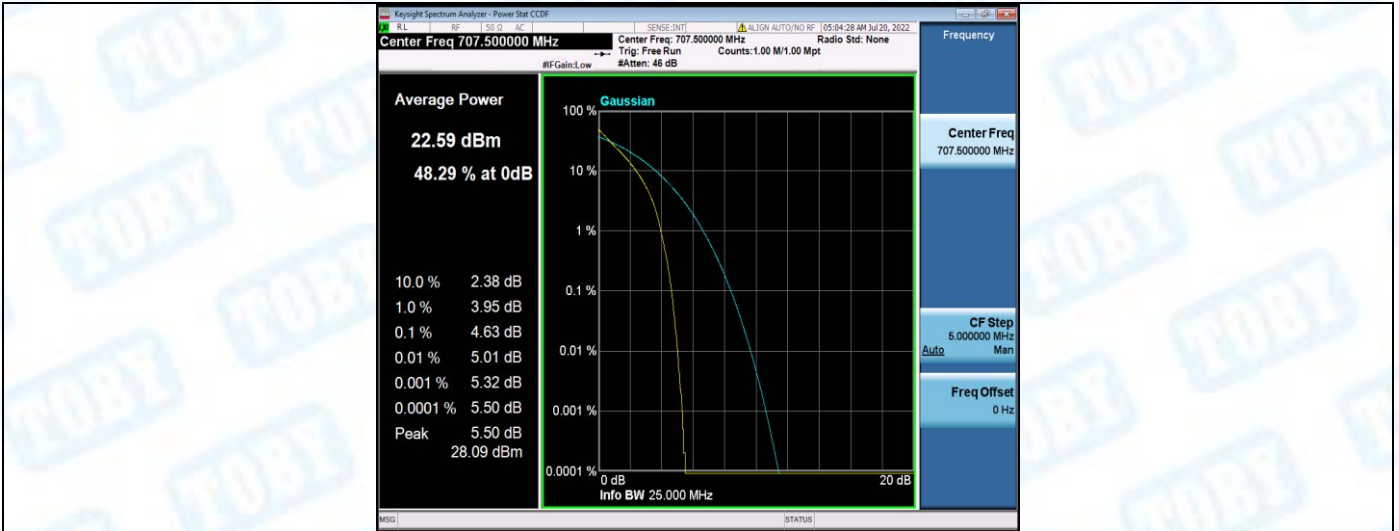
Band12-10MHz-QPSK-23130-1RB#0
