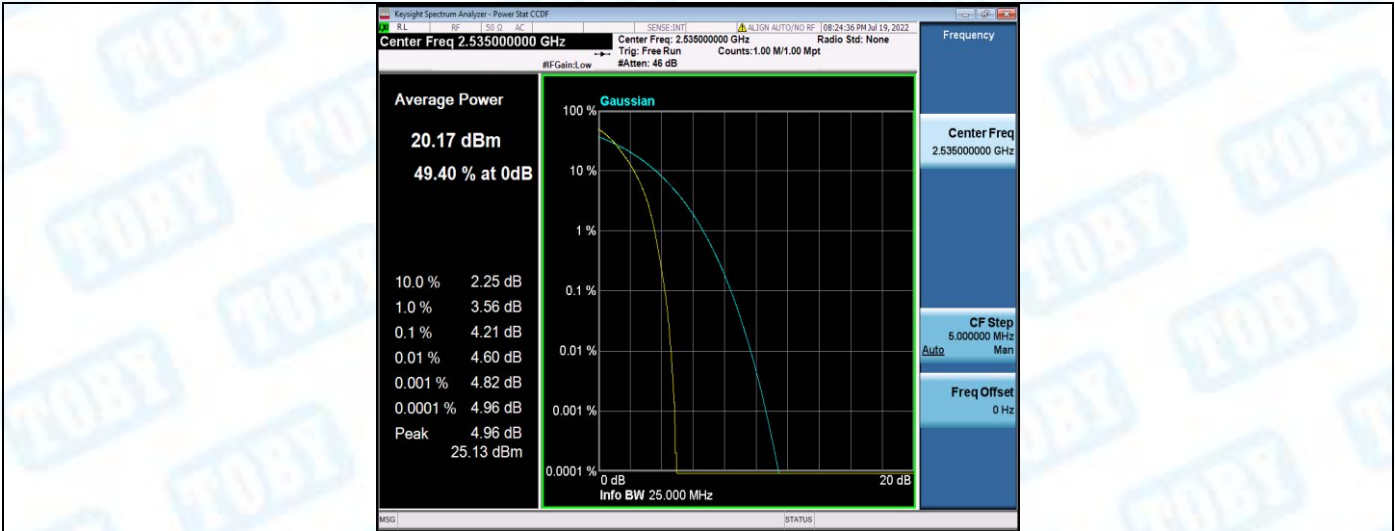
Band7-20MHz-QPSK-21350-1RB#0
