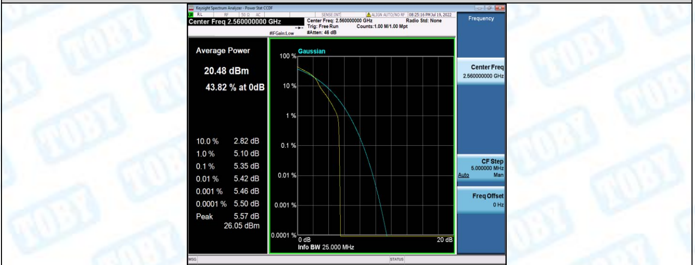
Band7-20MHz-16QAM-21350-100RB#0
