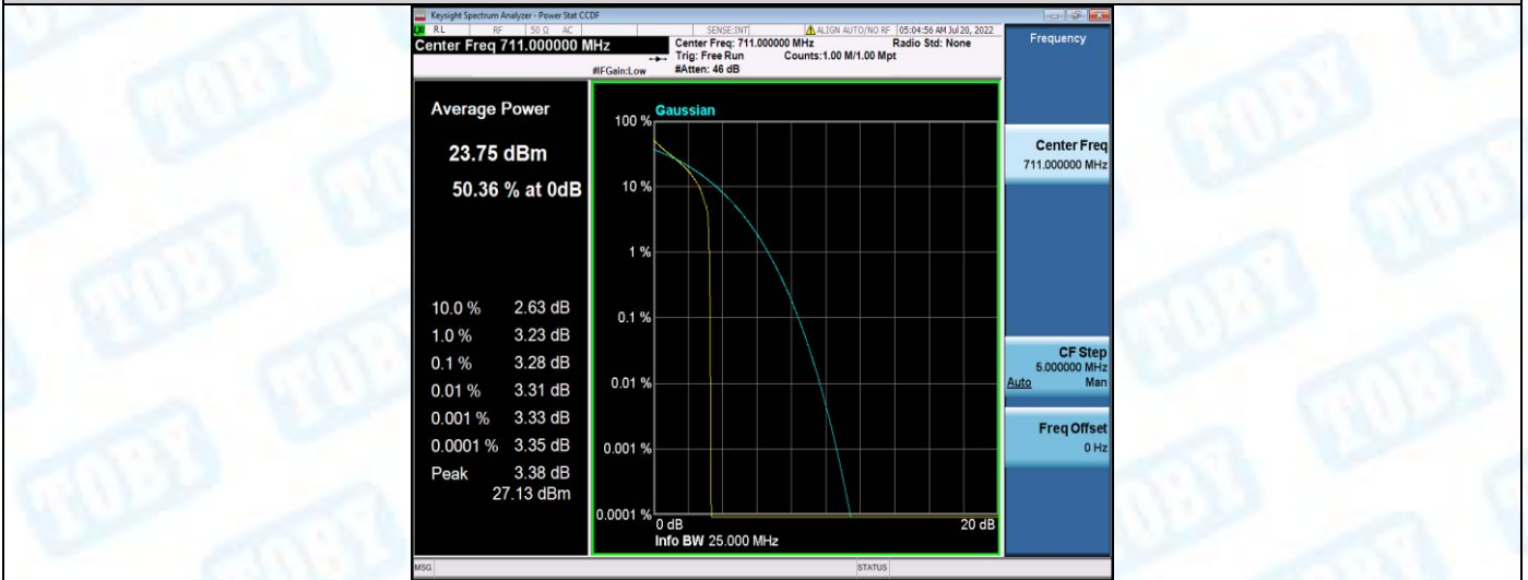
Band12-10MHz-QPSK-23130-50RB#0
