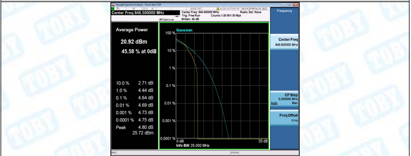
Band5-5MHz-16QAM-20625-25RB#0
