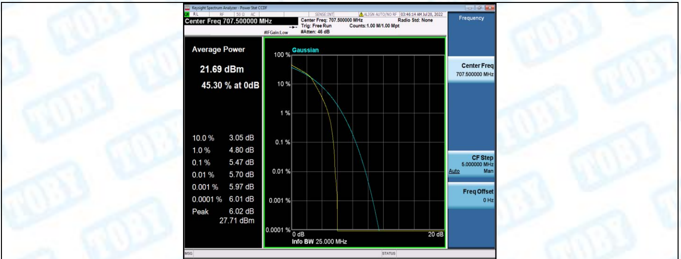
Band12-1.4MHz-16QAM-23173-1RB#0
