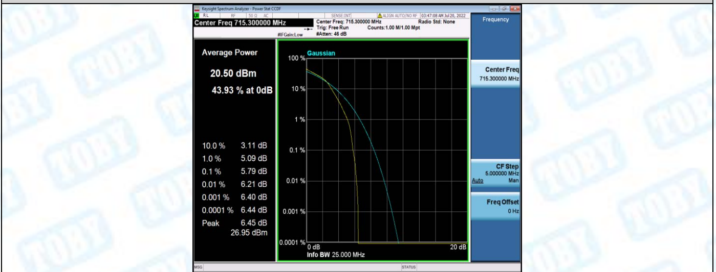
Band12-3MHz-QPSK-23025-1RB#0
