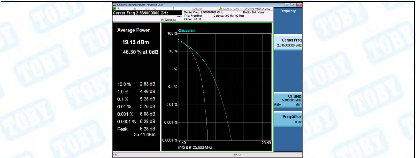
Band7-20MHz-16QAM-21350-1RB#0
