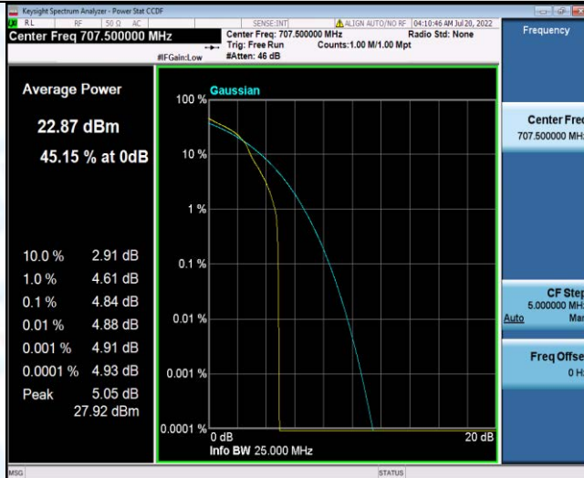
Band12-3MHz-16QAM-23095-15RB#0
