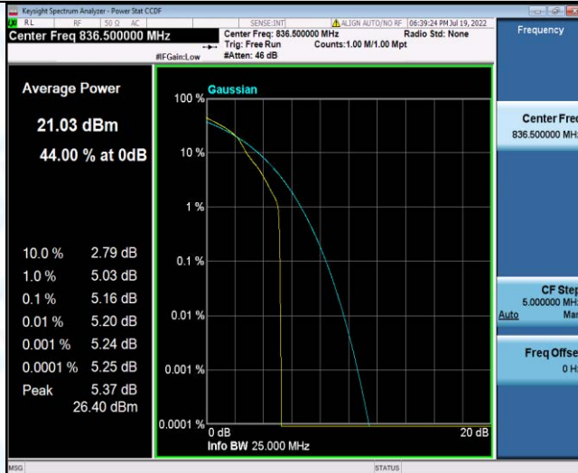
Band5-10MHz-16QAM-20525-50RB#0
