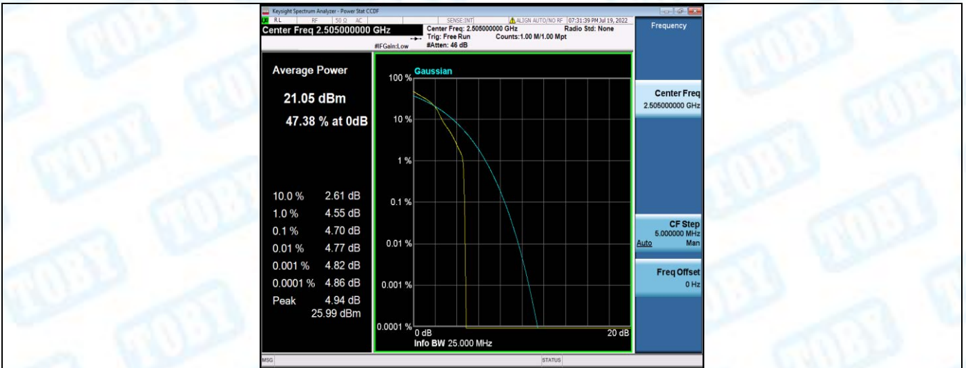
Band7-10MHz-16QAM-20800-50RB#0
