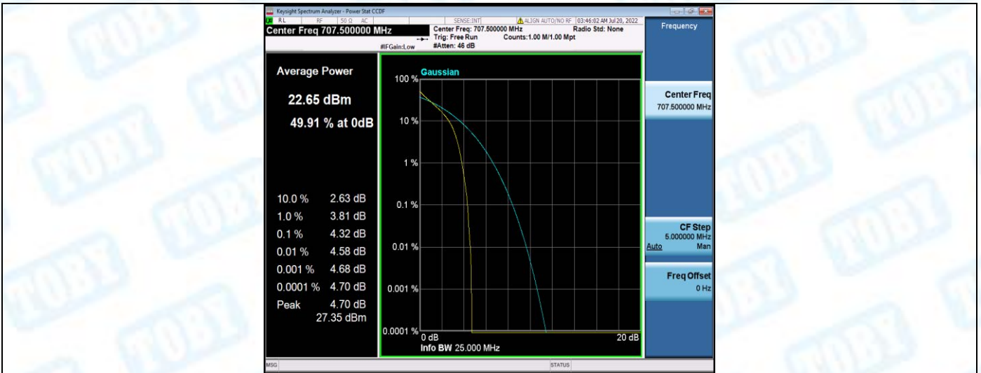
Band12-1.4MHz-QPSK-23173-1RB#0
