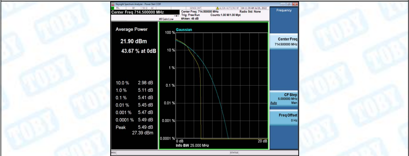
Band12-3MHz-16QAM-23165-15RB#0
