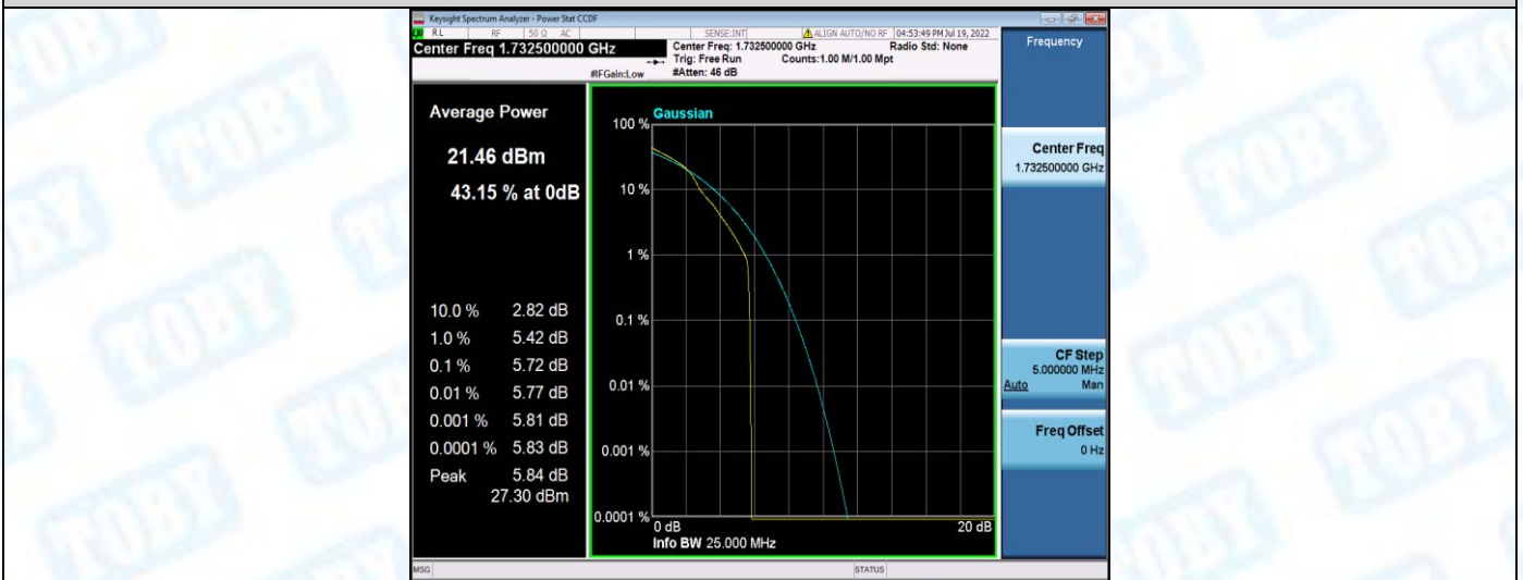
Band4-20MHz-16QAM-20175-100RB#0
