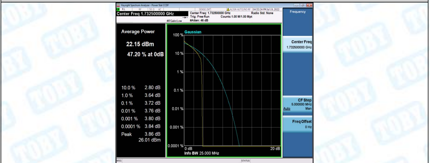
Band4-20MHz-QPSK-20175-100RB#0
