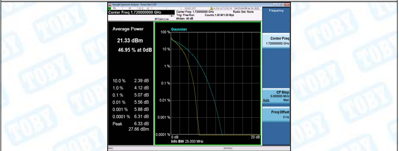
Band4-20MHz-QPSK-20175-1RB#0
