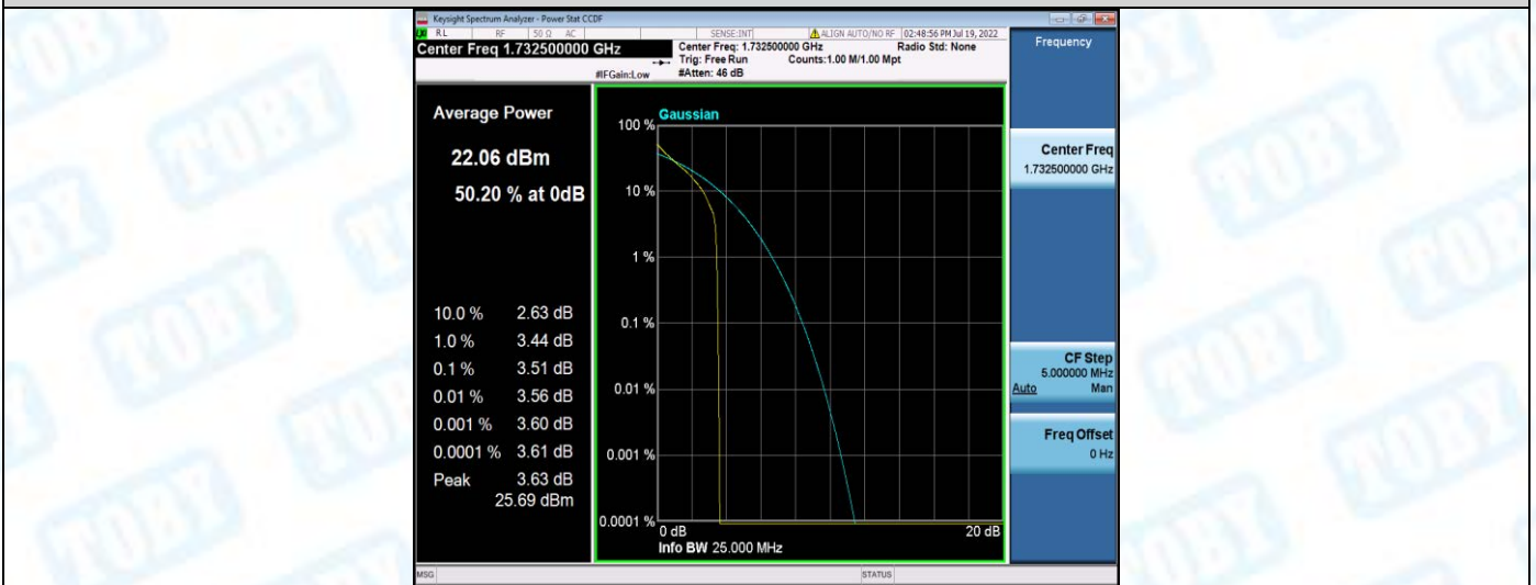
Band4-3MHz-QPSK-20175-15RB#0
