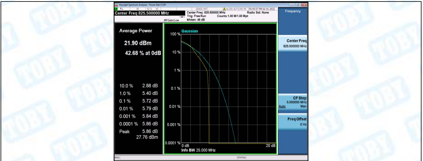
Band5-3MHz-16QAM-20415-15RB#0
