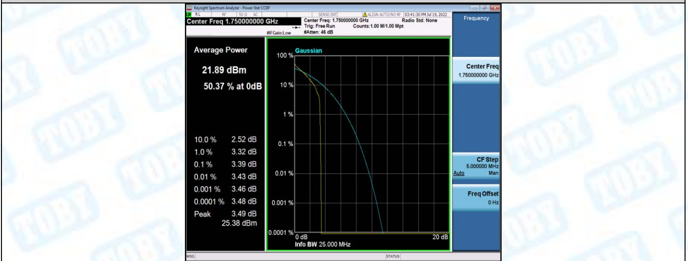
Band4-10MHz-QPSK-20350-50RB#0
