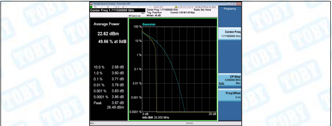
Band4-3MHz-QPSK-19965-15RB#0
