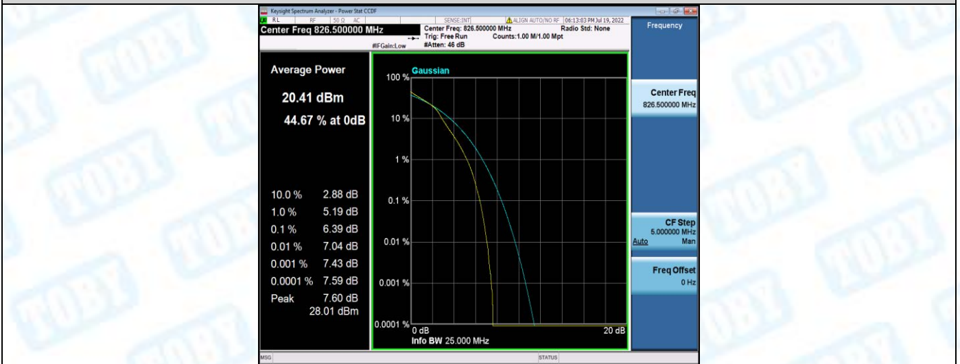
Band5-5MHz-16QAM-20525-1RB#0
