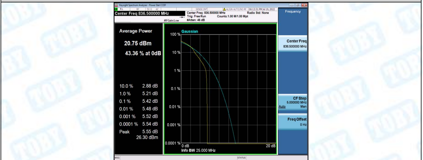
Band5-5MHz-16QAM-20525-25RB#0
