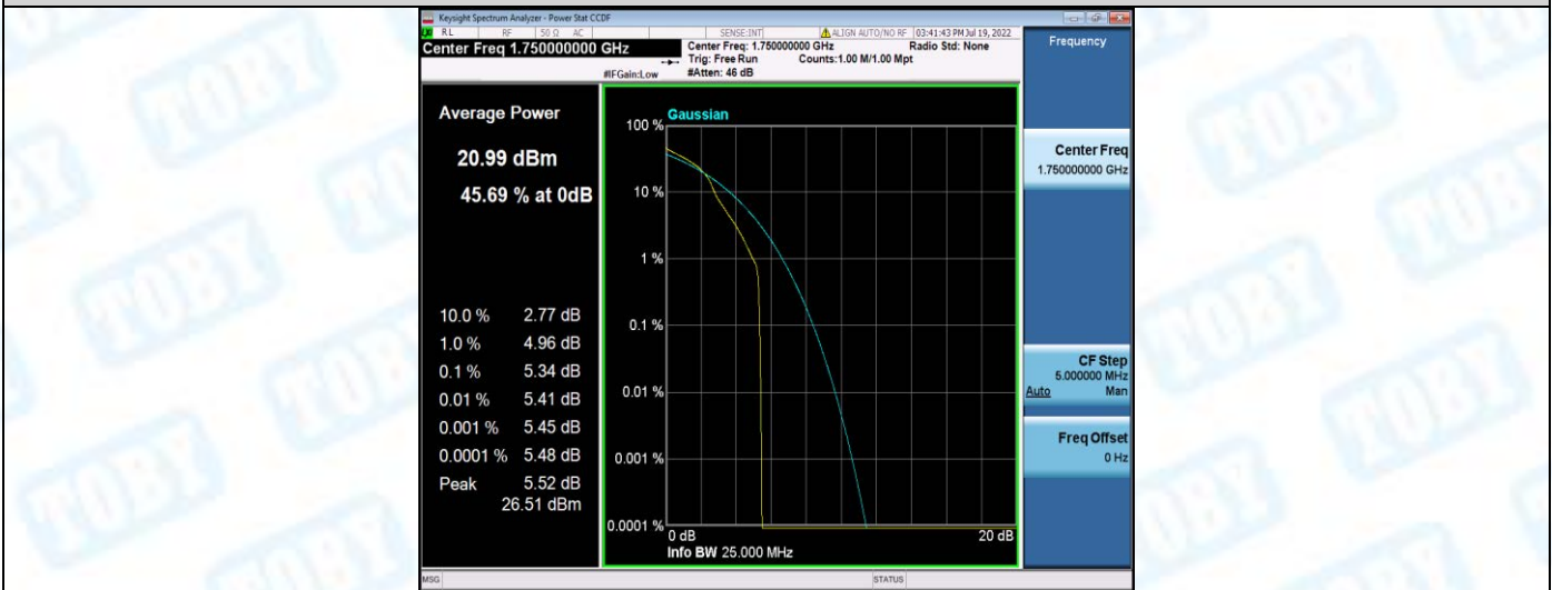
Band4-10MHz-16QAM-20350-50RB#0
