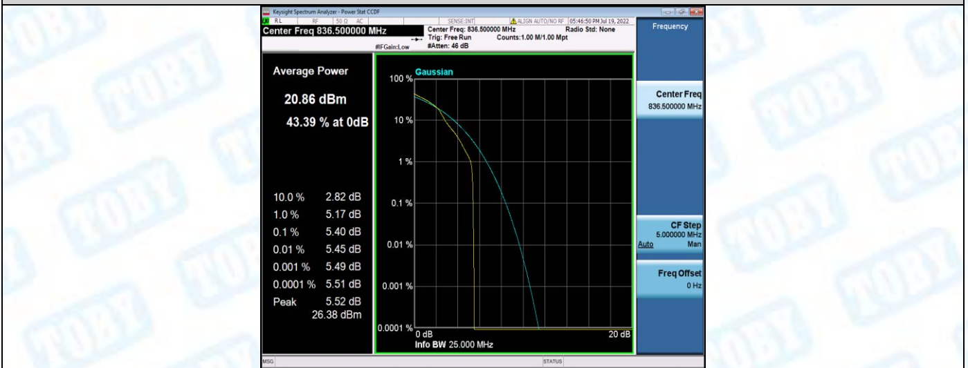
Band5-3MHz-16QAM-20525-15RB#0
