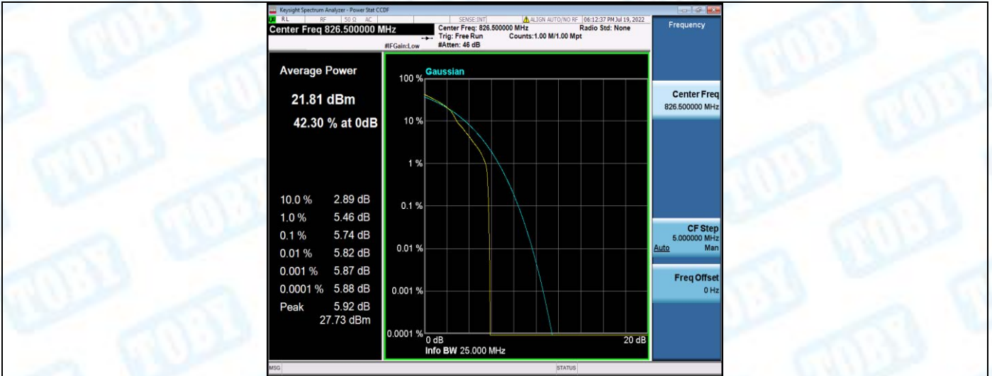
Band5-5MHz-16QAM-20425-25RB#0
