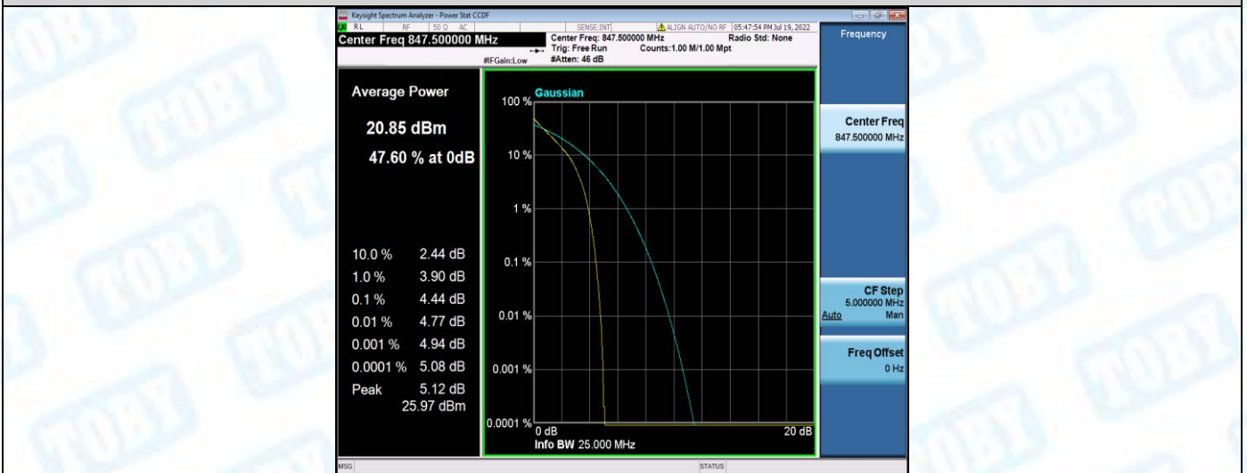
Band5-3MHz-16QAM-20415-1RB#0
