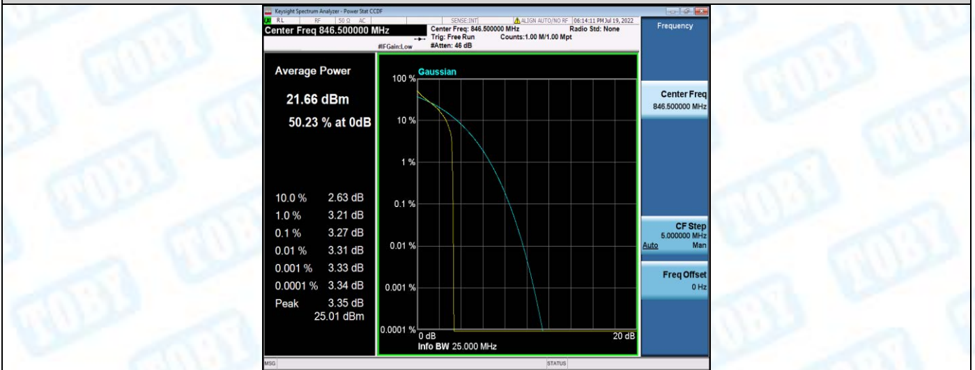
Band5-5MHz-QPSK-20625-25RB#0
