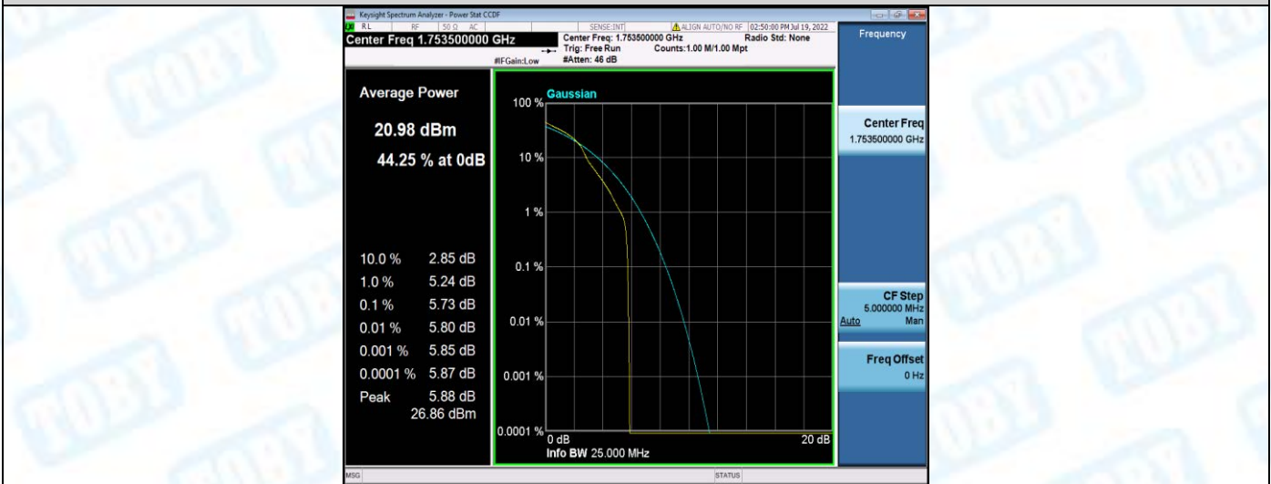
Band4-3MHz-16QAM-20385-15RB#0
