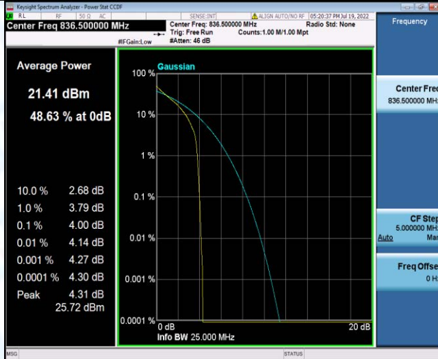
Band5-1.4MHz-QPSK-20525-6RB#0
