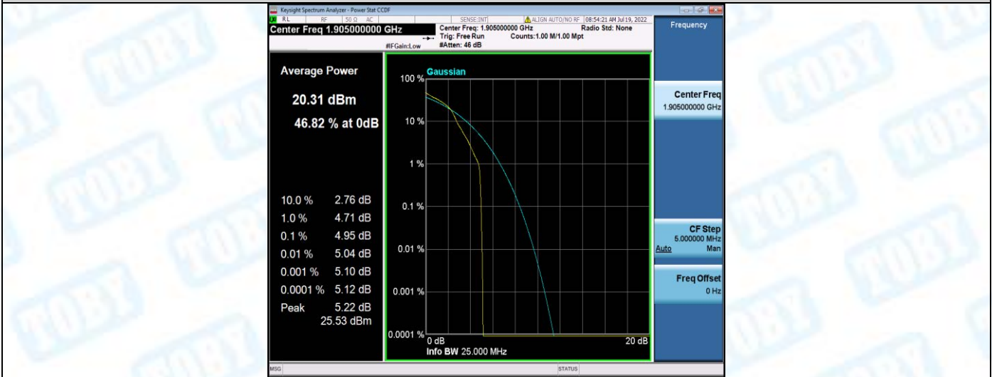
Band2-10MHz-16QAM-19150-50RB#0
