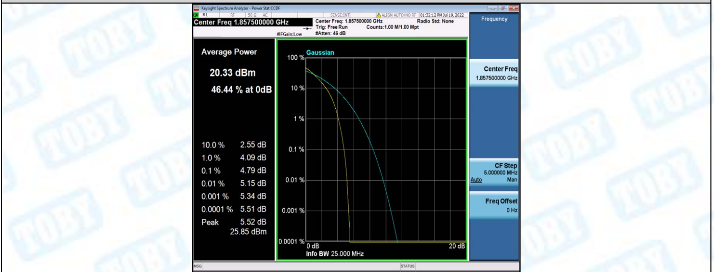
Band2-15MHz-QPSK-18900-1RB#0
