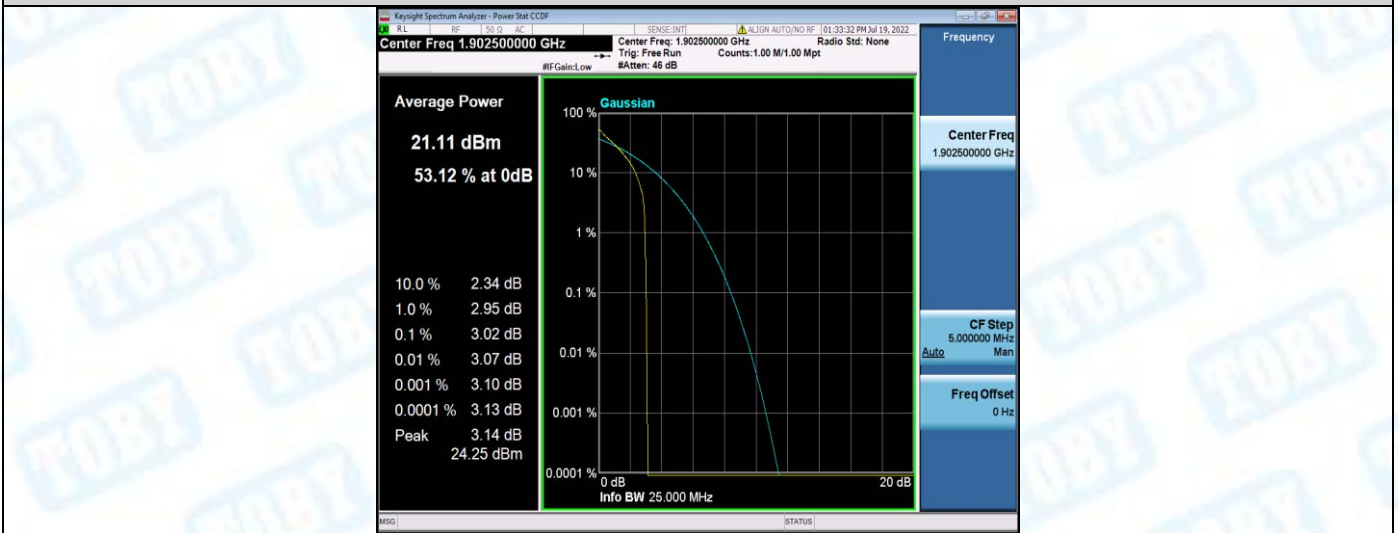
Band2-15MHz-QPSK-19125-75RB#0
