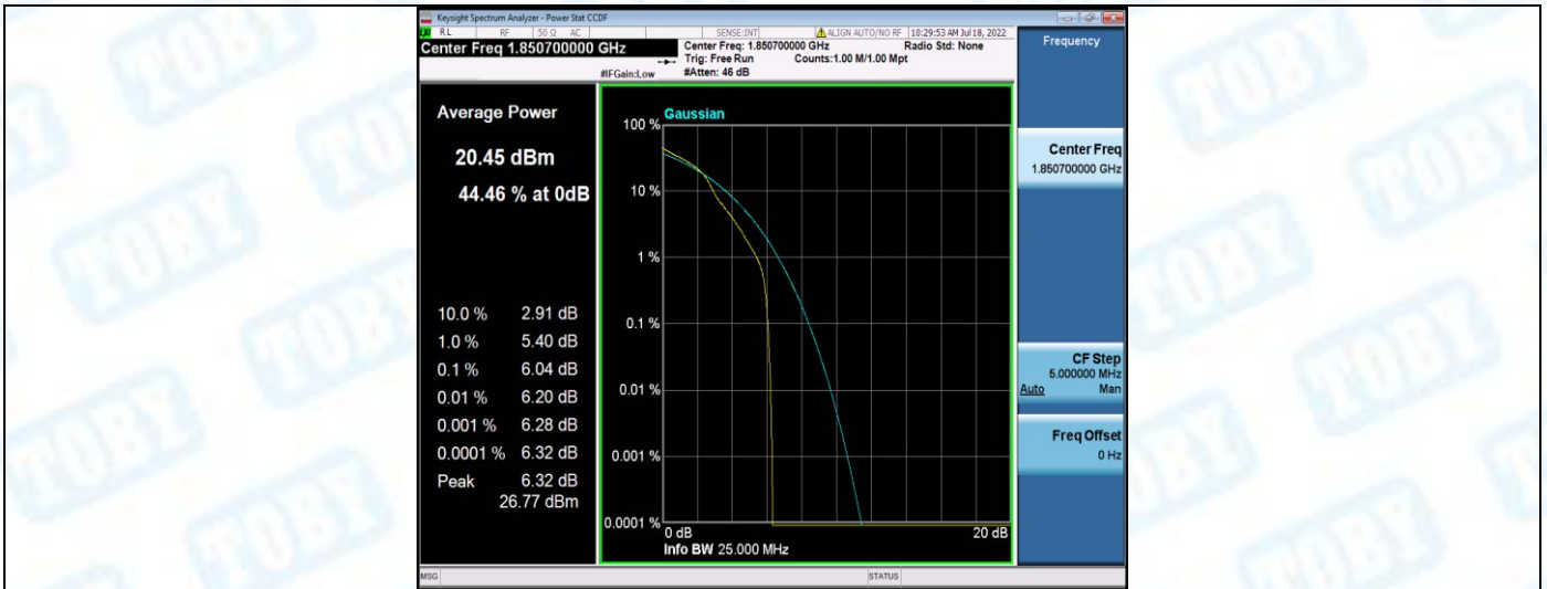
Band2-1.4MHz-16QAM-18607-6RB#0
