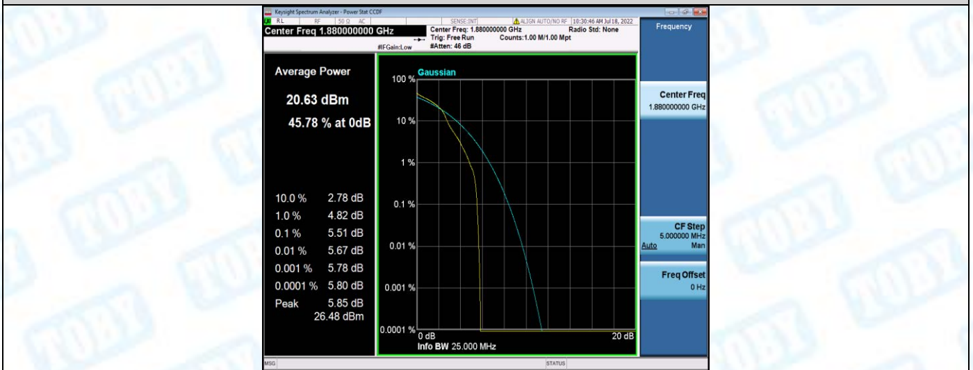
Band2-1.4MHz-16QAM-18900-6RB#0
