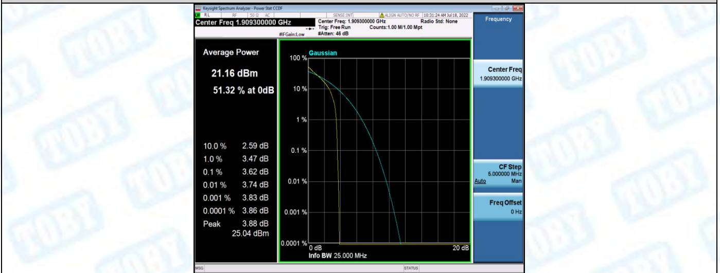
Band2-1.4MHz-QPSK-19193-6RB#0
