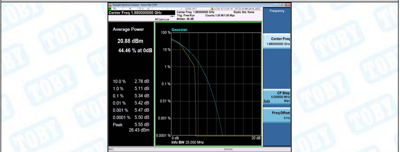
Band2-3MHz-16QAM-18900-15RB#0
