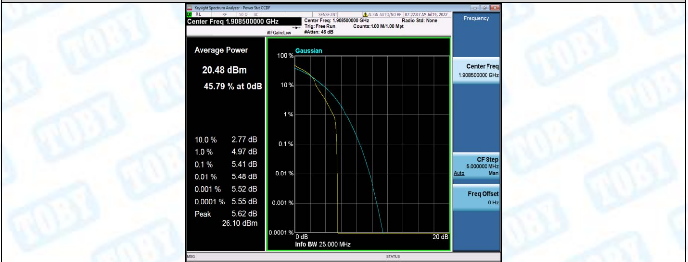
Band2-3MHz-16QAM-19185-15RB#0
