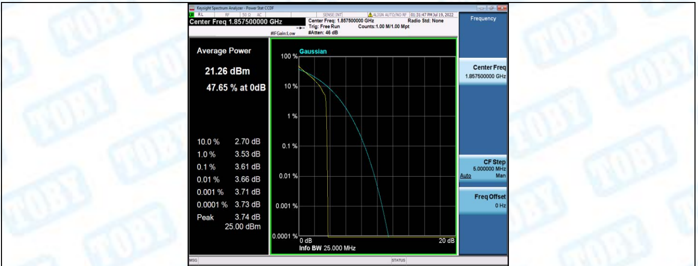
Band2-15MHz-QPSK-18675-75RB#0
