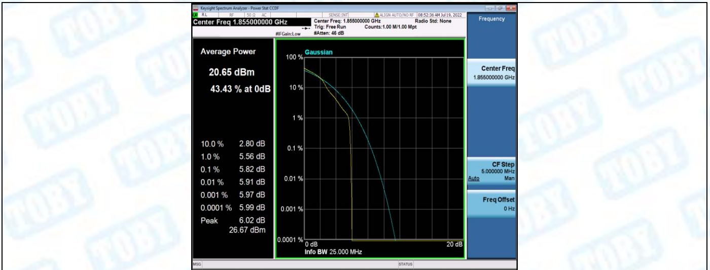
Band2-10MHz-16QAM-18650-50RB#0
