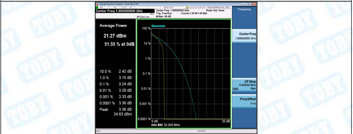
Band2-10MHz-QPSK-19150-50RB#0
