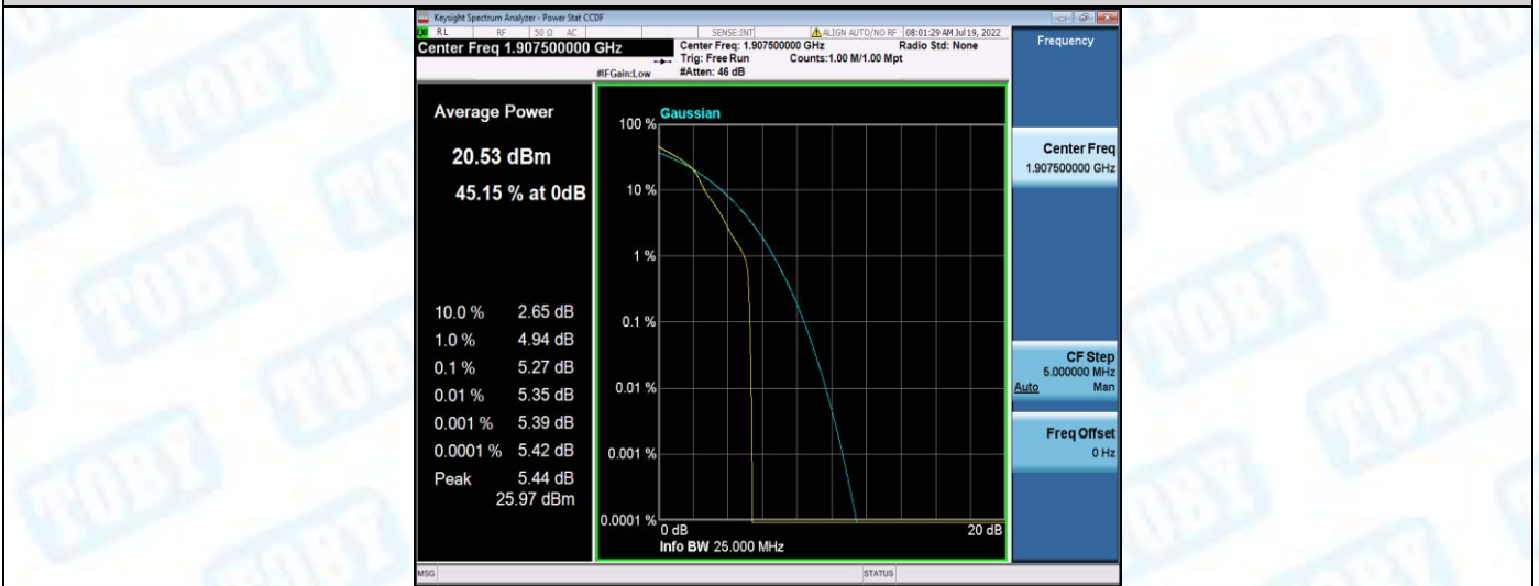
Band2-5MHz-16QAM-19175-25RB#0
