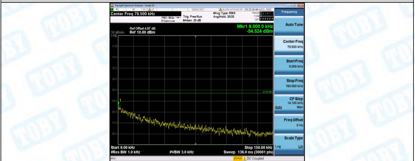
Band4-1413-2-0.009~0.15MHz
