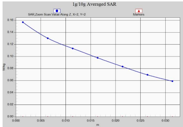
Fig.A.1- 37 Z-Scan at power reference point (LTE band71)
