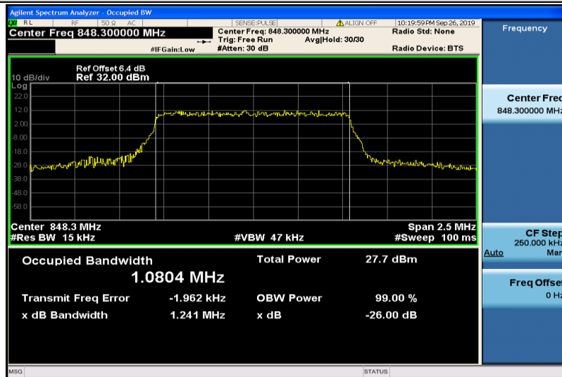
Band5-1.4MHz-QPSK-20643-6RB#0-1.0804
