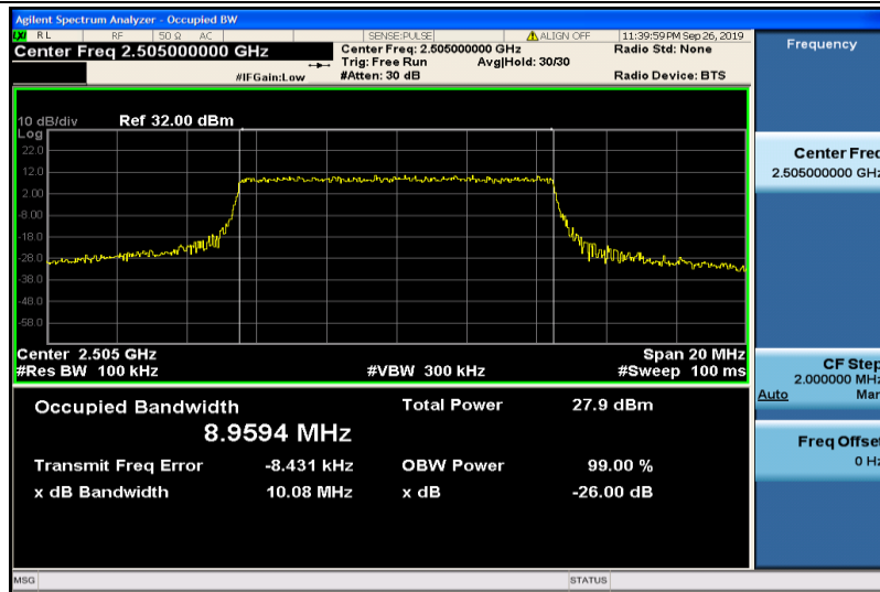
Band7-10MHz-16QAM-20800-50RB#0-8.9594
