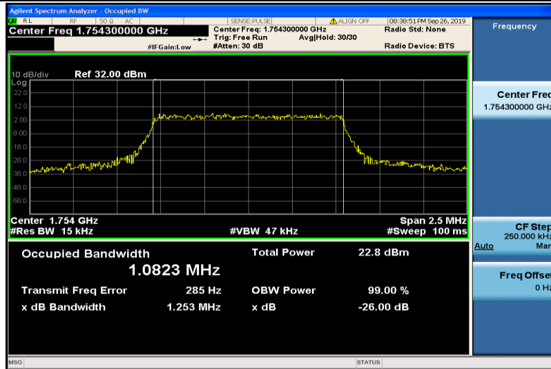
Band4-1.4MHz-16QAM-20393-6RB#0-1.0823
