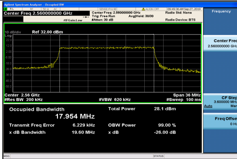
Band7-20MHz-16QAM-21350-100RB#0-17.954
