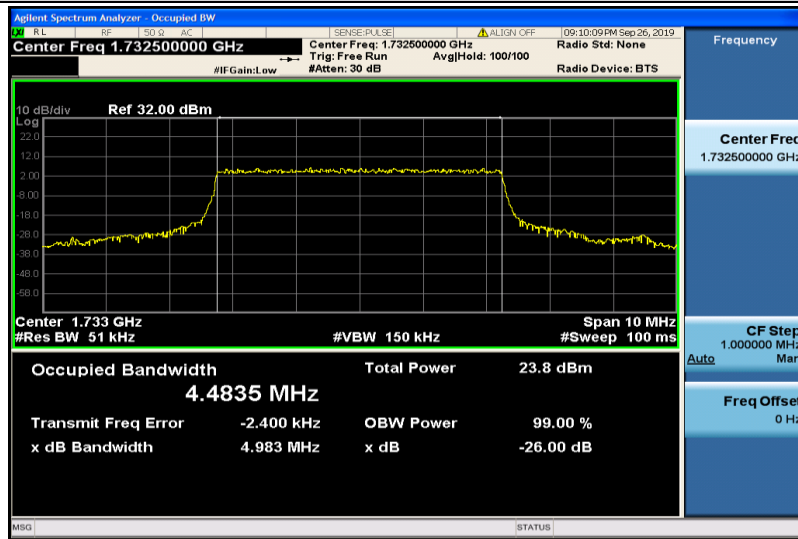
Band4-5MHz-QPSK-20175-25RB#0-4.4835
