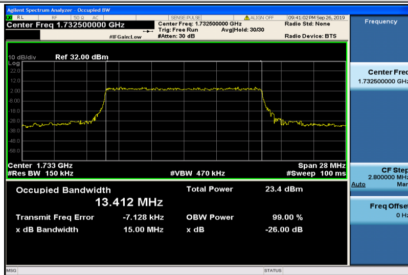
Band4-15MHz-QPSK-20175-75RB#0-13.412
