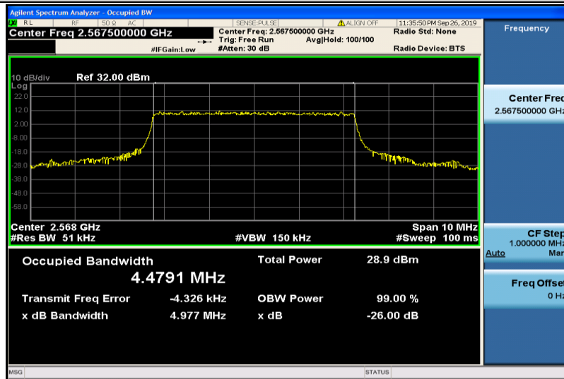
Band7-5MHz-QPSK-21425-25RB#0-4.4791
