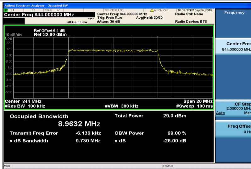
Band5-10MHz-QPSK-20600-50RB#0-8.9632
