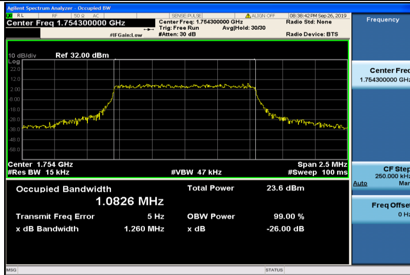
Band4-1.4MHz-QPSK-20393-6RB#0-1.0826
