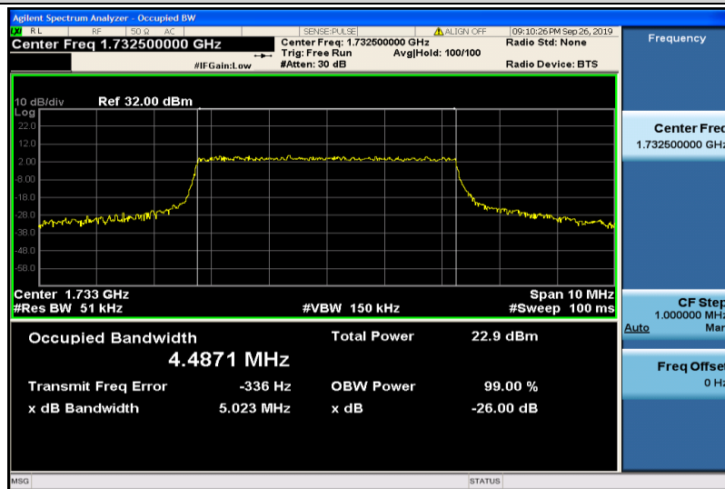
Band4-5MHz-16QAM-20175-25RB#0-4.4871
