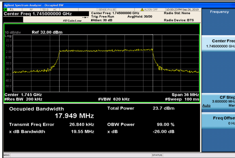
Band4-20MHz-16QAM-20300-100RB#0-17.949
