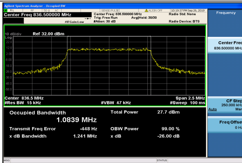
Band5-1.4MHz-QPSK-20525-6RB#0-1.0839
