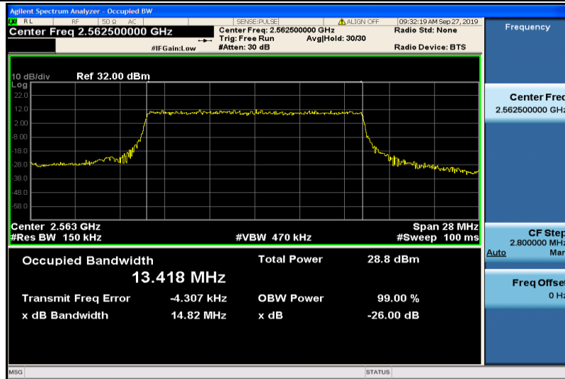
Band7-15MHz-QPSK-21375-75RB#0-13.418
