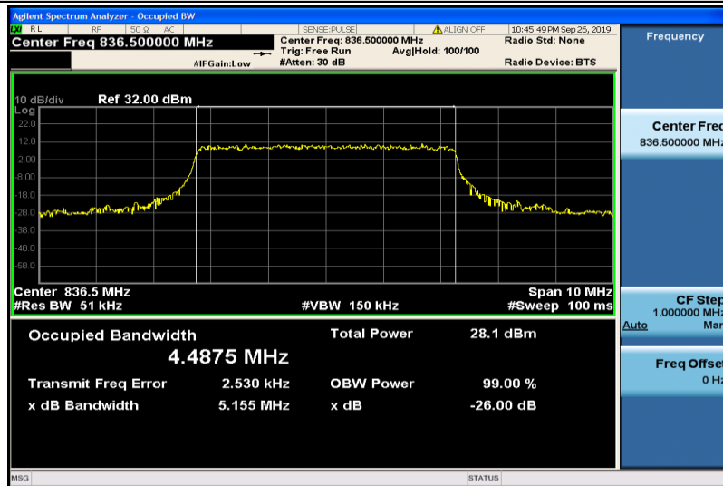
Band5-5MHz-16QAM-20525-25RB#0-4.4875
