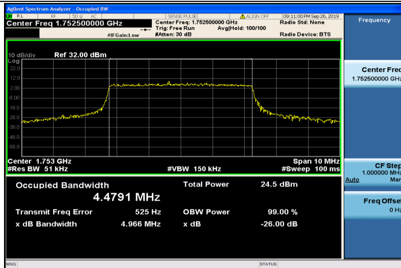
Band4-5MHz-16QAM-20375-25RB#0-4.4791
