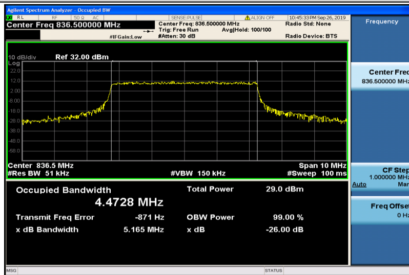
Band5-5MHz-QPSK-20525-25RB#0-4.4728
