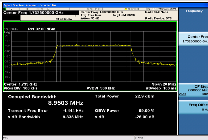
Band4-10MHz-QPSK-20175-50RB#0-8.9503
