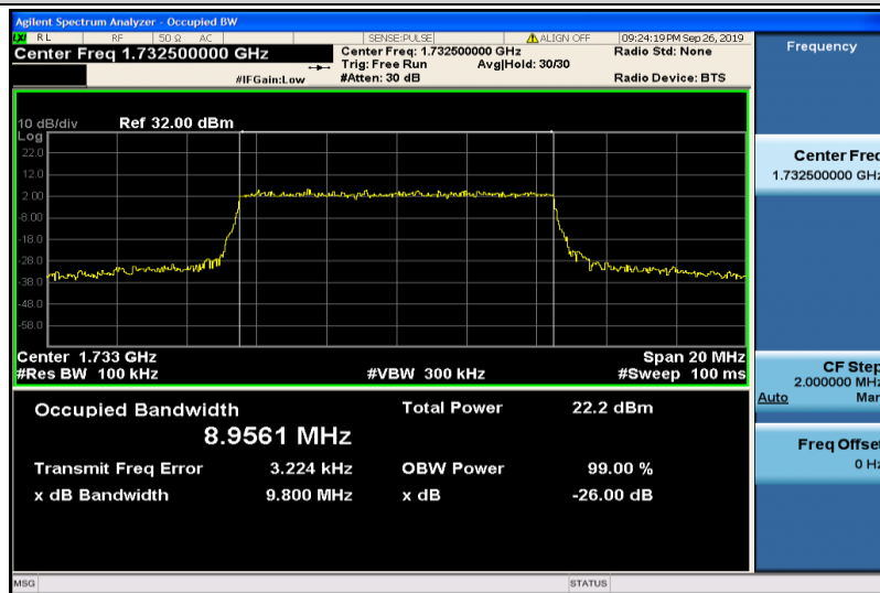
Band4-10MHz-16QAM-20175-50RB#0-8.9561
