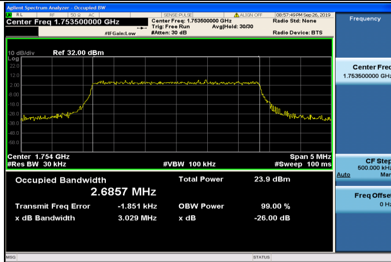
Band4-3MHz-16QAM-20385-15RB#0-2.6857
