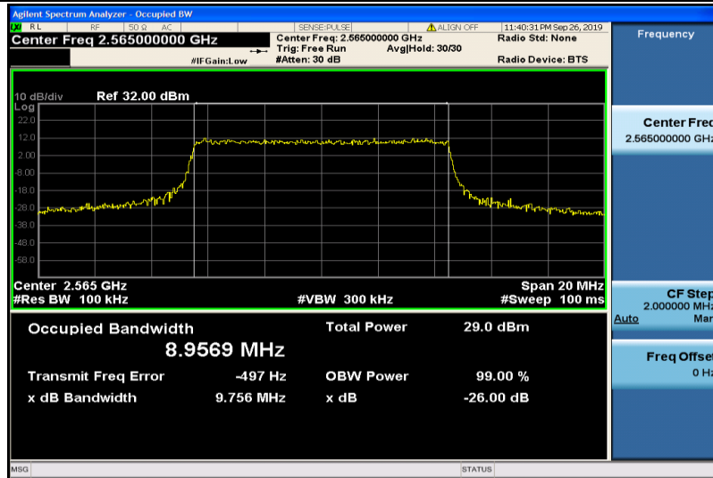
Band7-10MHz-QPSK-21400-50RB#0-8.9569
