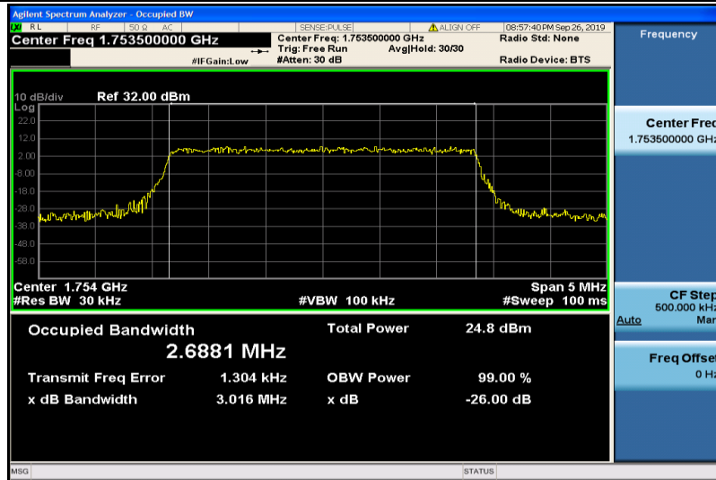
Band4-3MHz-QPSK-20385-15RB#0-2.6881
