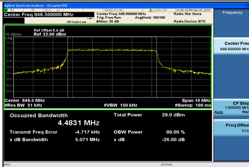
Band5-5MHz-QPSK-20625-25RB#0-4.4831
