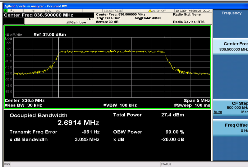
Band5-3MHz-16QAM-20525-15RB#0-2.6914
