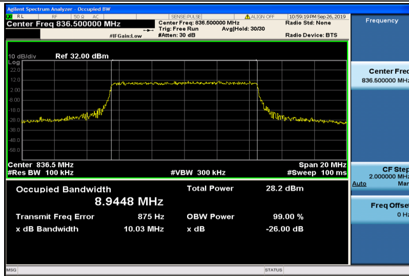
Band5-10MHz-16QAM-20525-50RB#0-8.9448
