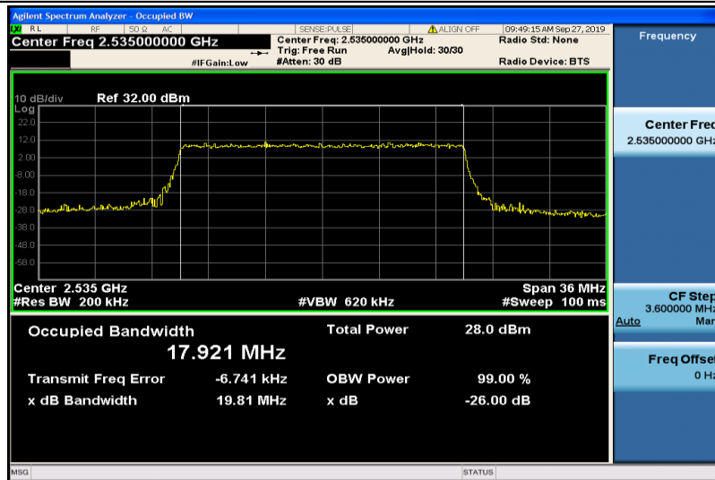
Band7-20MHz-16QAM-21100-100RB#0-17.921
