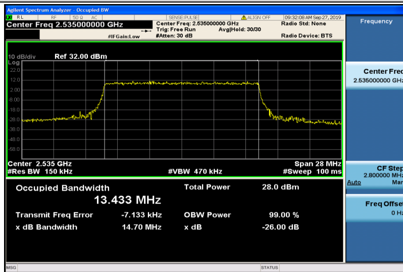
Band7-15MHz-16QAM-21100-75RB#0-13.433
