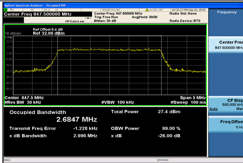
Band5-3MHz-16QAM-20635-15RB#0-2.6847
