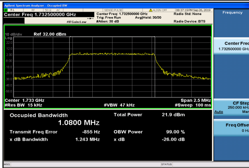
Band4-1.4MHz-QPSK-20175-6RB#0-1.0800
