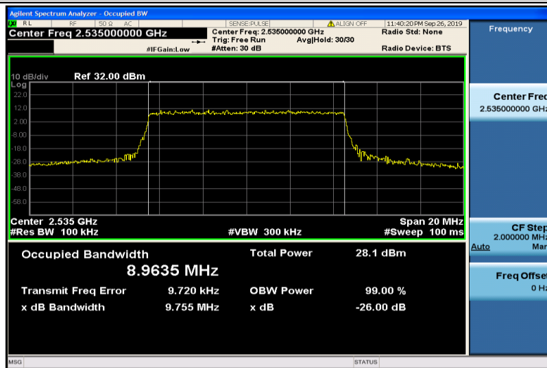
Band7-10MHz-16QAM-21100-50RB#0-8.9635
