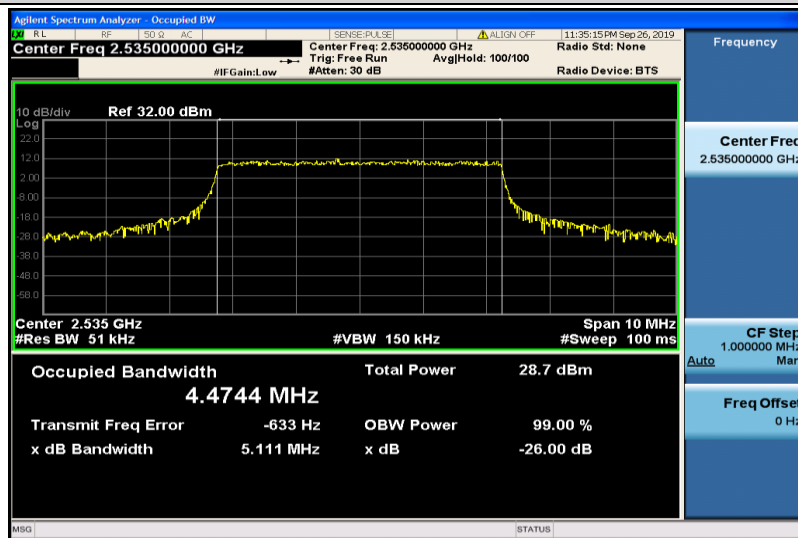
Band7-5MHz-QPSK-21100-25RB#0-4.4744
