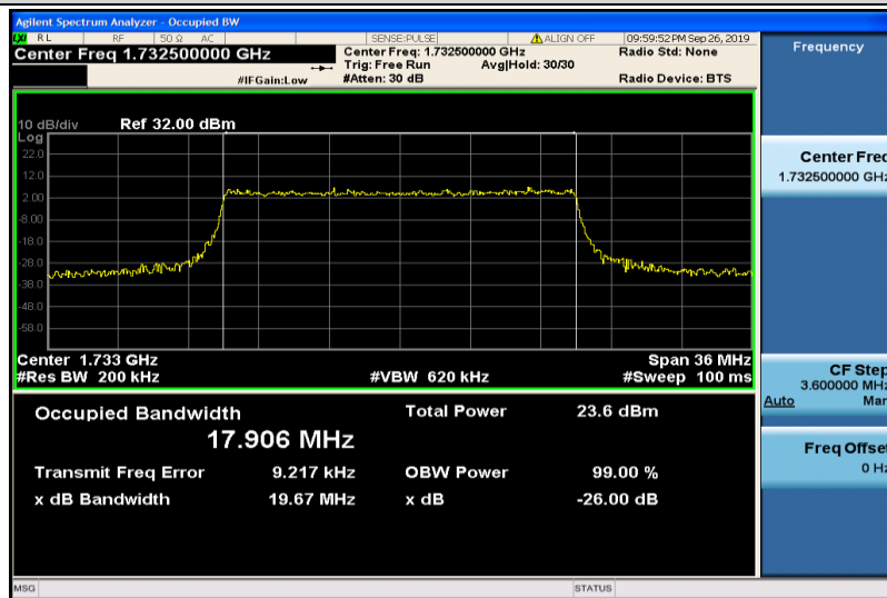
Band4-20MHz-QPSK-20175-100RB#0-17.906
