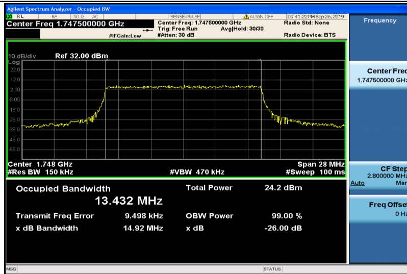
Band4-15MHz-QPSK-20325-75RB#0-13.432
