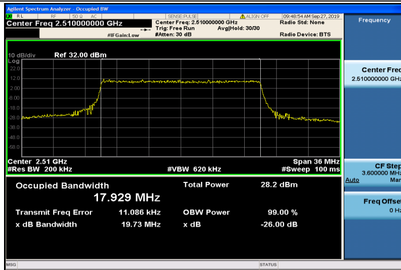
Band7-20MHz-16QAM-20850-100RB#0-17.929
