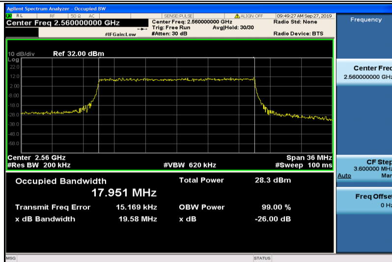
Band7-20MHz-QPSK-21350-100RB#0-17.951
