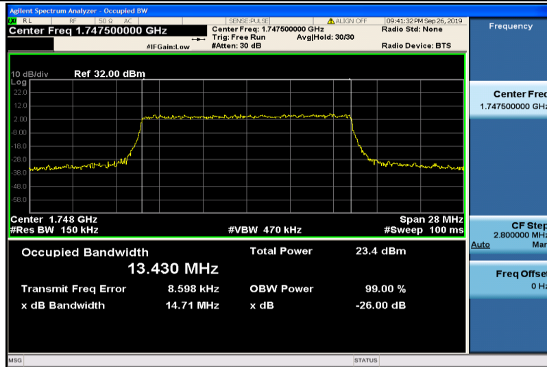
Band4-15MHz-16QAM-20325-75RB#0-13.430
