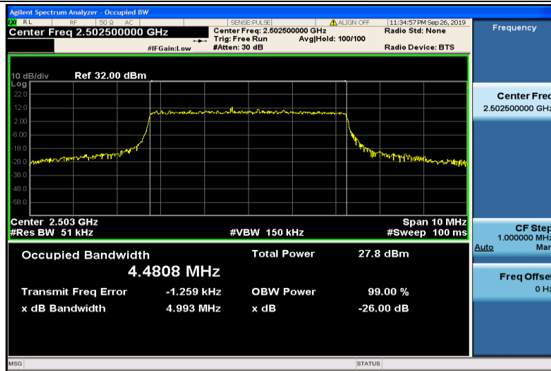
Band7-5MHz-16QAM-20775-25RB#0-4.4808
