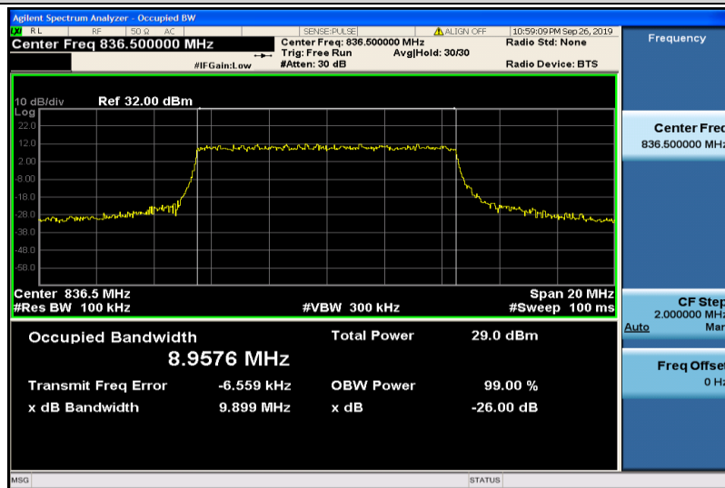
Band5-10MHz-QPSK-20525-50RB#0-8.9576
