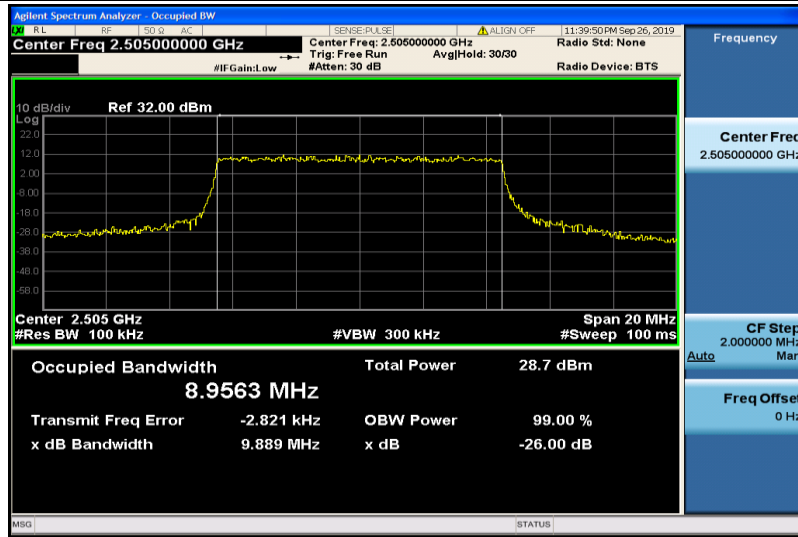
Band7-10MHz-QPSK-20800-50RB#0-8.9563
