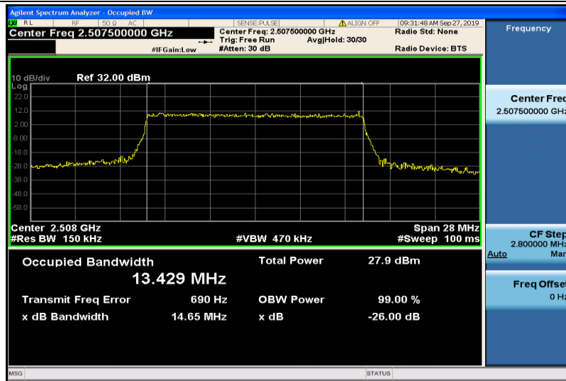
Band7-15MHz-16QAM-20825-75RB#0-13.429
