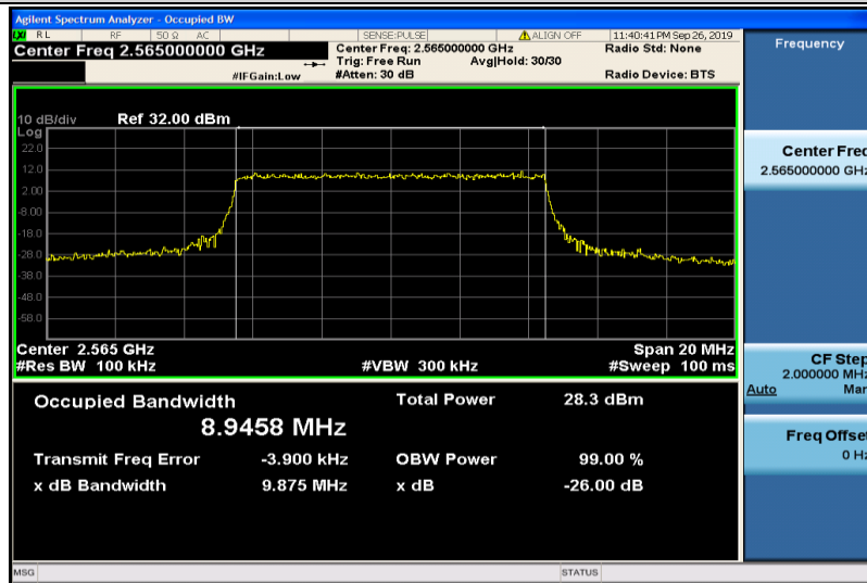
Band7-10MHz-16QAM-21400-50RB#0-8.9458
