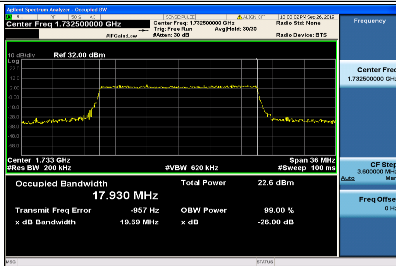
Band4-20MHz-16QAM-20175-100RB#0-17.930
