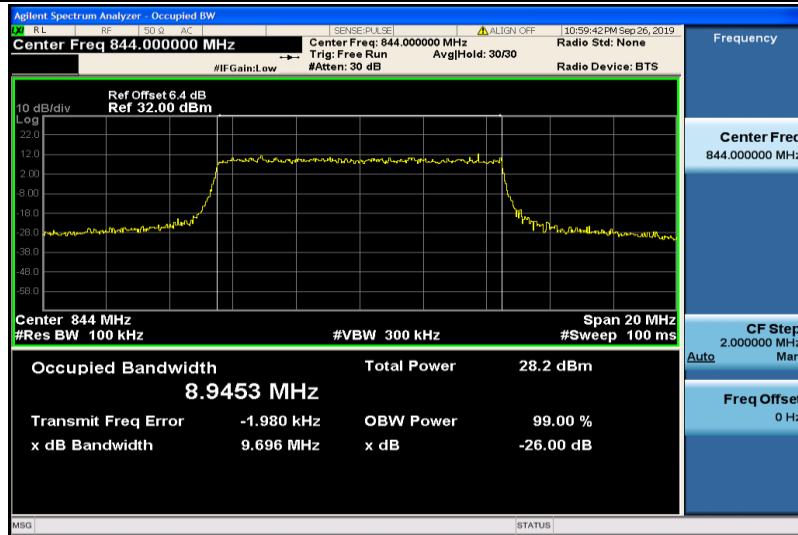
Band5-10MHz-16QAM-20600-50RB#0-8.9453
