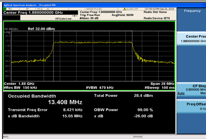
Band2-15MHz-QPSK-18900-75RB#0-13.408
