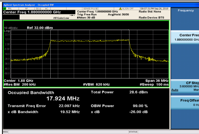
Band2-20MHz-QPSK-18900-100RB#0-17.924
