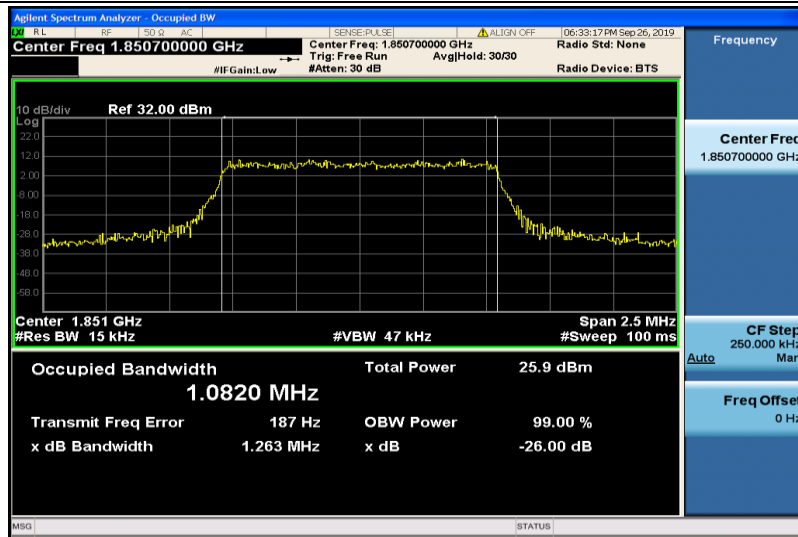
Band2-1.4MHz-16QAM-18607-6RB#0-1.0820
