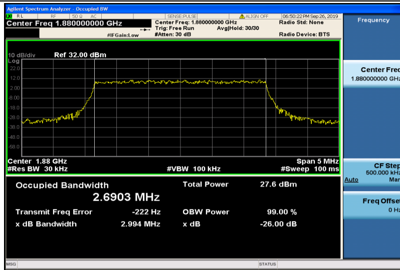
Band2-3MHz-QPSK-18900-15RB#0-2.6903
