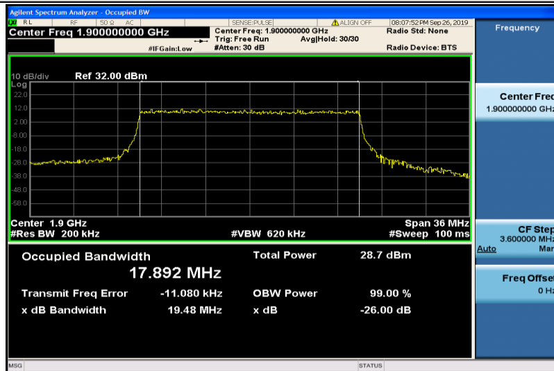
Band2-20MHz-QPSK-19100-100RB#0-17.892
