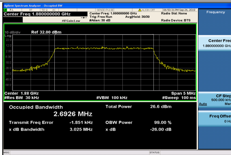
Band2-3MHz-16QAM-18900-15RB#0-2.6926
