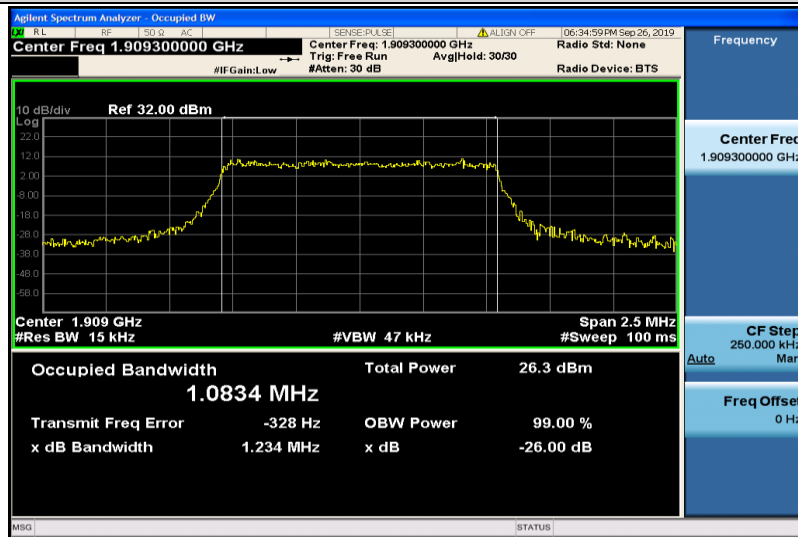
Band2-1.4MHz-16QAM-19193-6RB#0-1.0834
