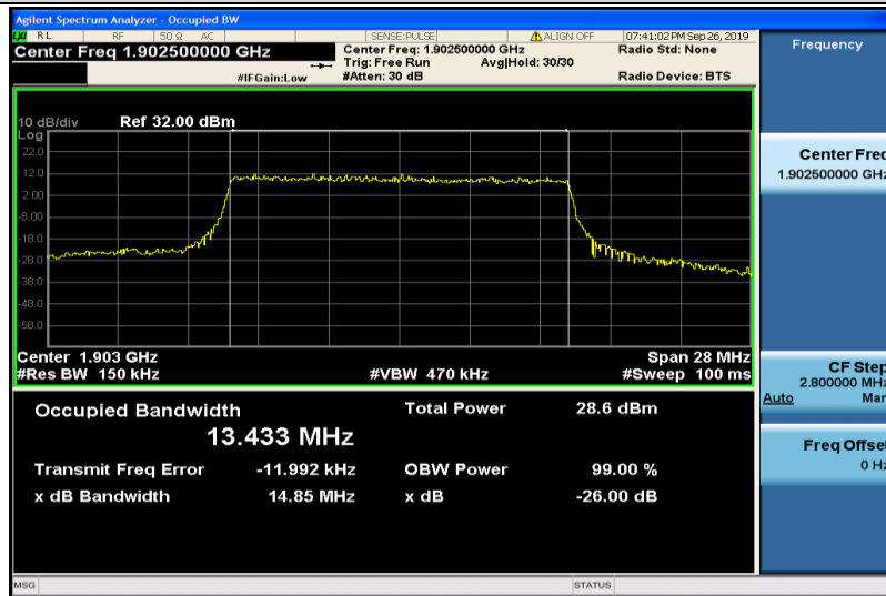
Band2-15MHz-QPSK-19125-75RB#0-13.433
