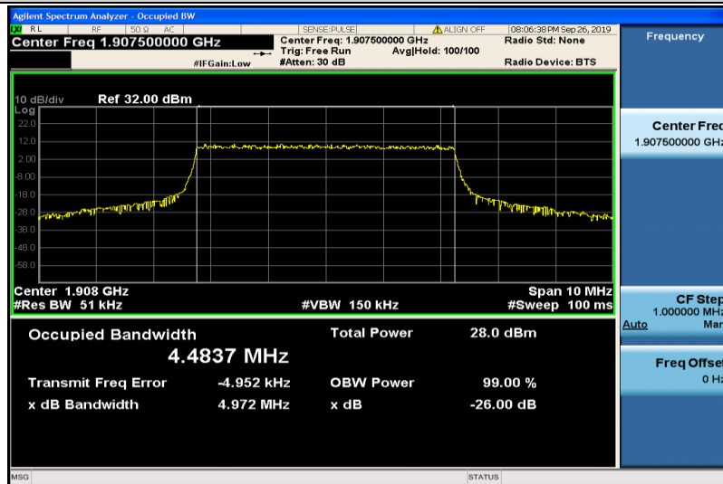
Band2-5MHz-QPSK-19175-25RB#0-4.4837
