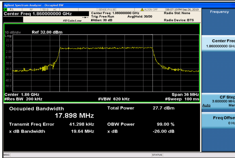
Band2-20MHz-16QAM-18700-100RB#0-17.898
