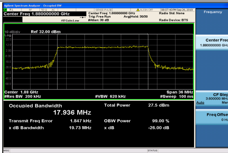
Band2-20MHz-16QAM-18900-100RB#0-17.936
