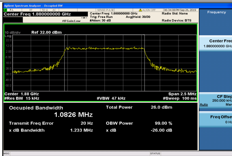
Band2-1.4MHz-16QAM-18900-6RB#0-1.0826
