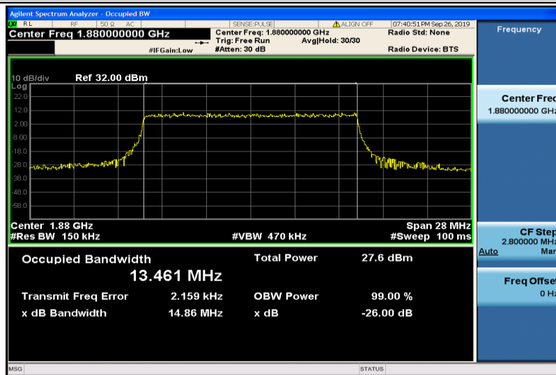
Band2-15MHz-16QAM-18900-75RB#0-13.461
