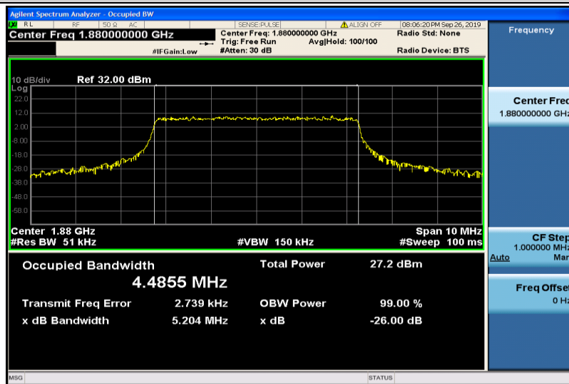
Band2-5MHz-16QAM-18900-25RB#0-4.4855
