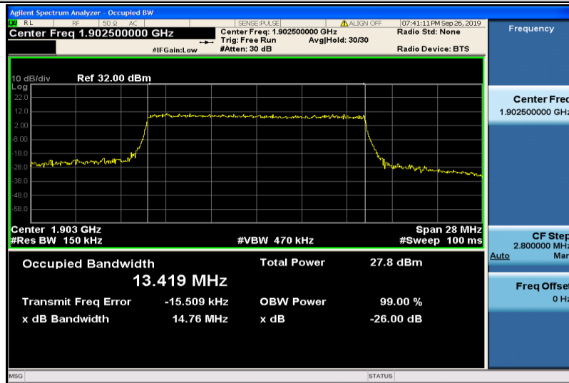
Band2-15MHz-16QAM-19125-75RB#0-13.419
