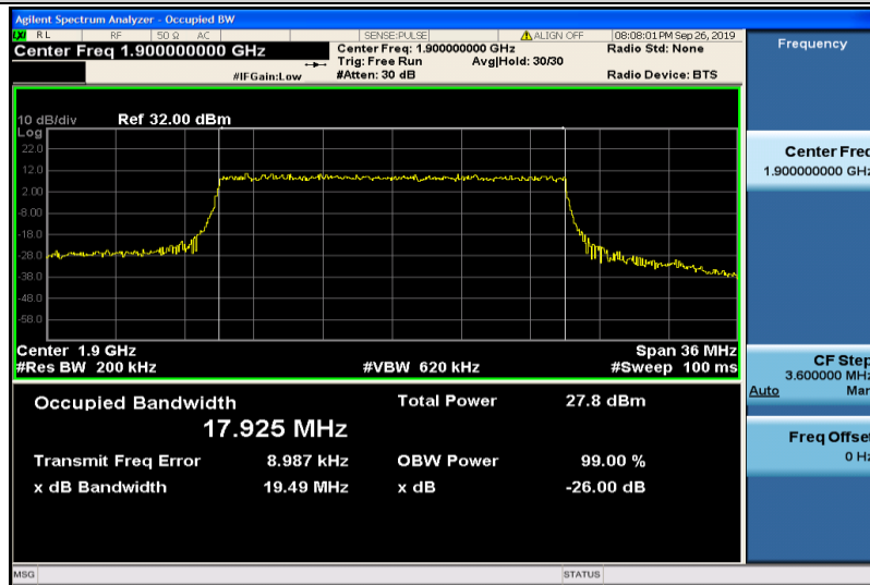
Band2-20MHz-16QAM-19100-100RB#0-17.925
