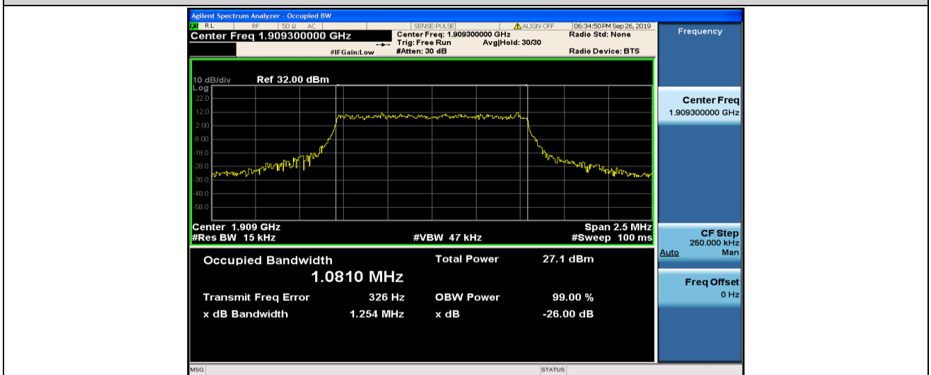
Band2-1.4MHz-QPSK-19193-6RB#0-1.0810
