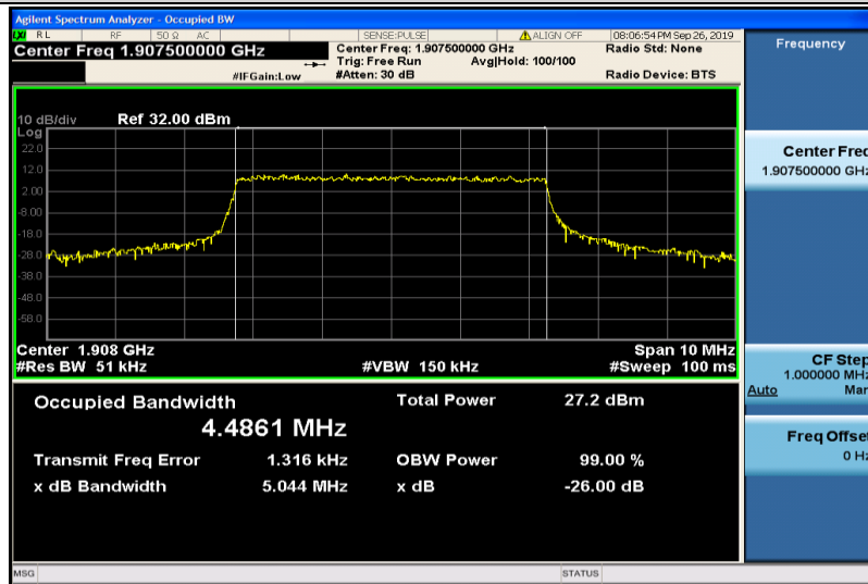
Band2-5MHz-16QAM-19175-25RB#0-4.4861
