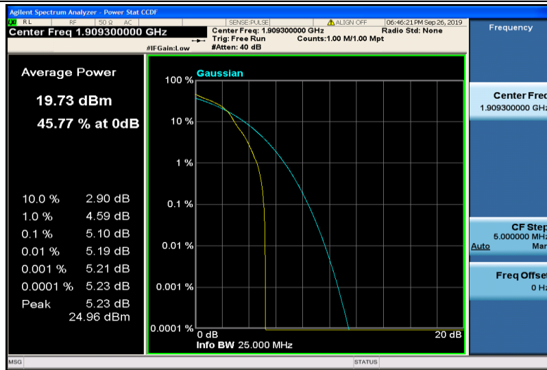
Band2-1.4MHz-16QAM-1913-1RB#0
