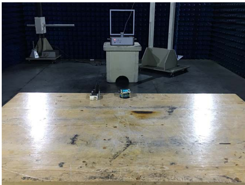
Photograph of set-up for Radiated Emission below 30MHz
