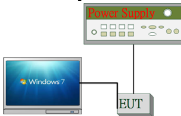
Fig. 2-2 Conducted (Antenna Port) Configuration
