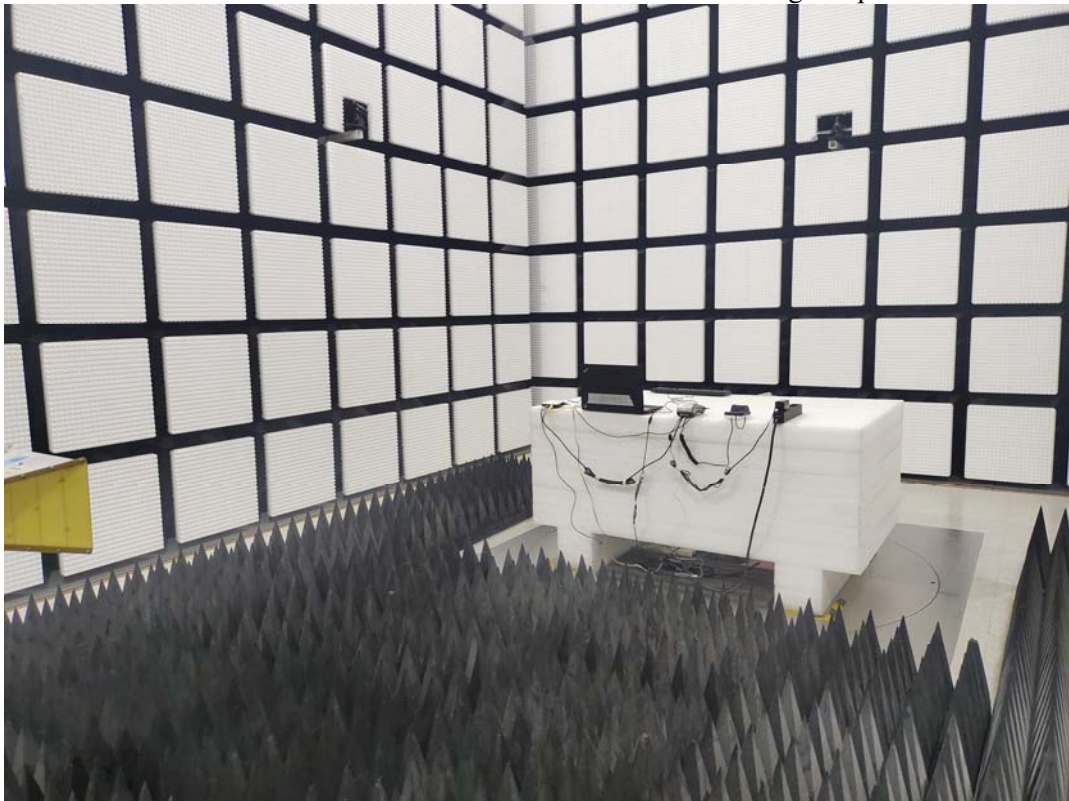
Radiated Emission Above 1GHz Rear View Downloading Adapter #1
