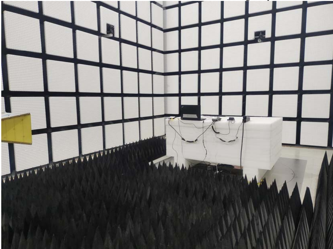
Radiated Emission Above 1GHz Rear View Downloading Adapter #2
