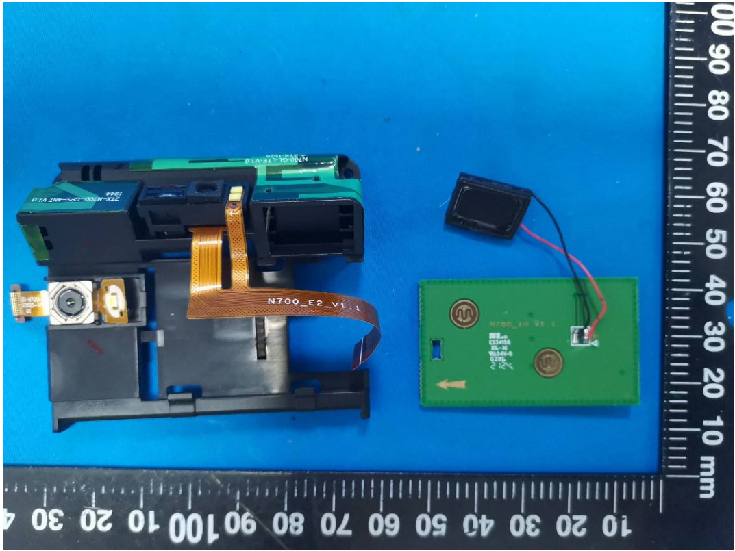
2G/3G/4G Antenna
