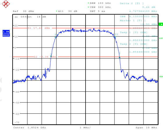
26dB&99% Occupied Bandwidth Plot on Channel 9262
