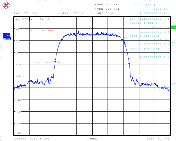
26dB&99% Occupied Bandwidth Plot on Channel 9538
