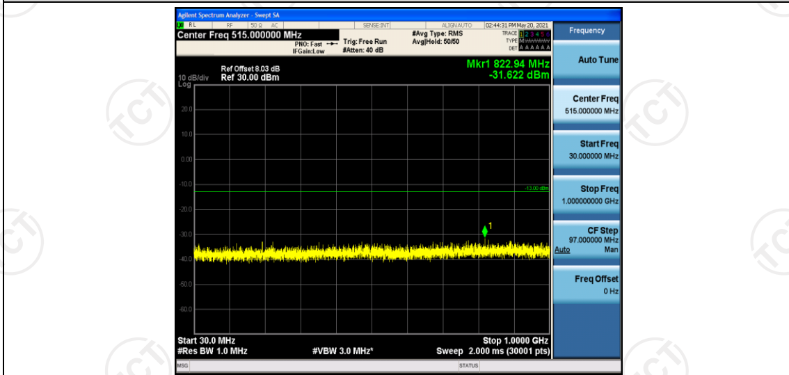
Band66-15MHz-QPSK-132047-1RB#0-Range4:1000~5000MHz
