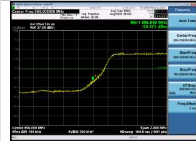
LCH_QPSK_25RB#0
