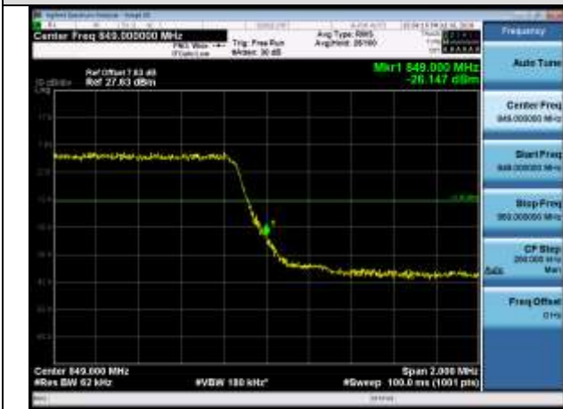
HCH_QPSK_15RB#0
