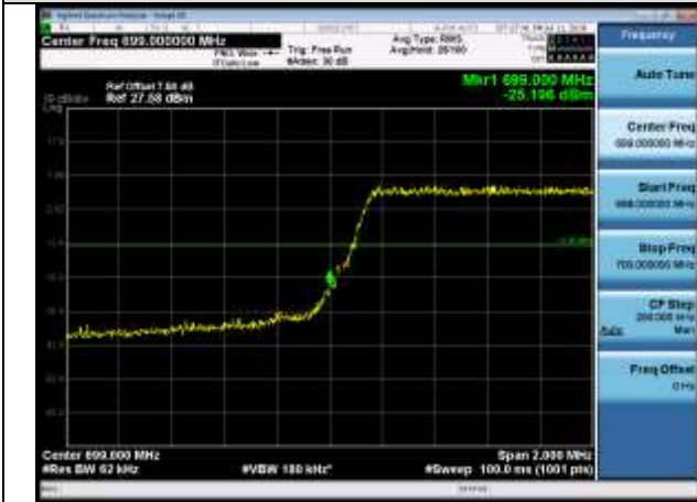
LCH_QPSK_15RB#0
