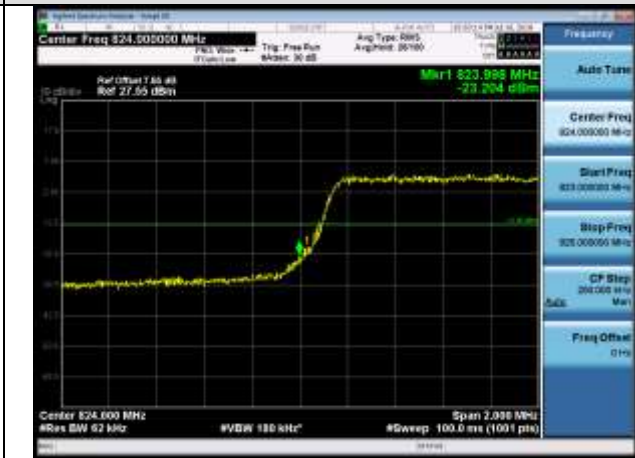
LCH_16QAM_15RB#0
