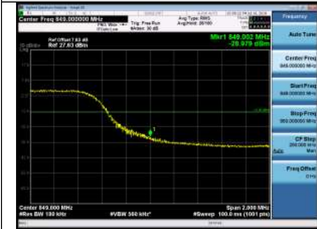
HCH_QPSK_50RB#0
