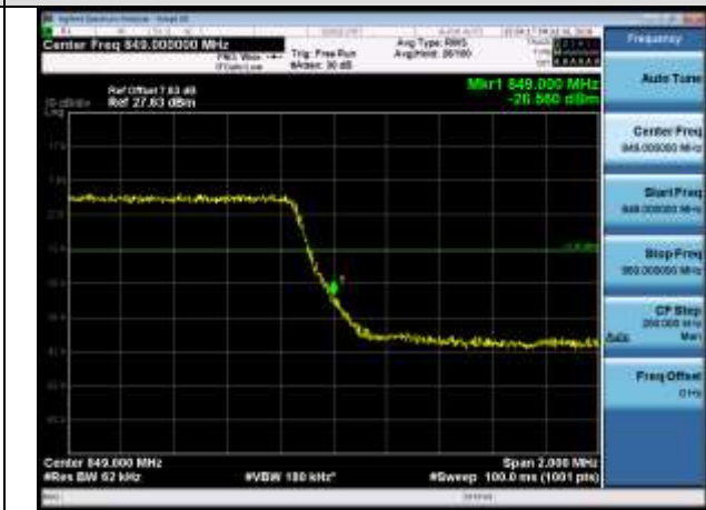
HCH_16QAM_15RB#0
