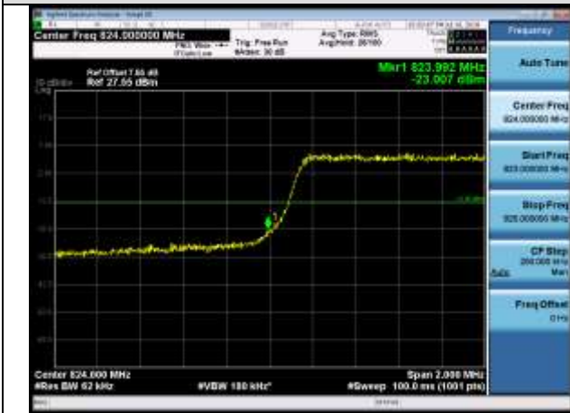
LCH_QPSK_15RB#0
