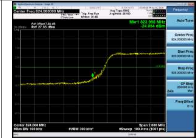
LCH_16QAM_25RB#0
