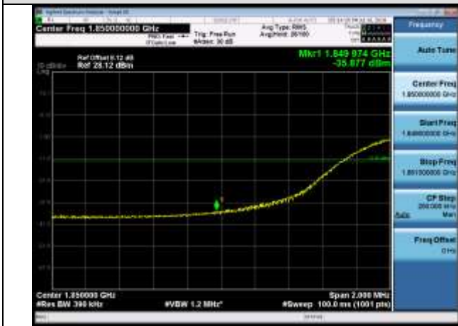
LCH_QPSK_100RB#0
