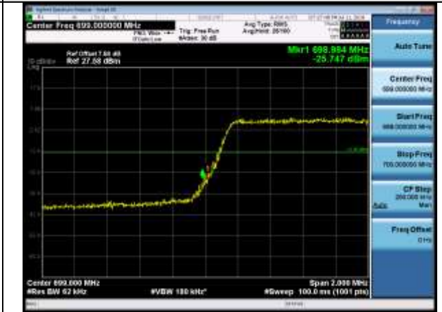
LCH_16QAM_15RB#0
