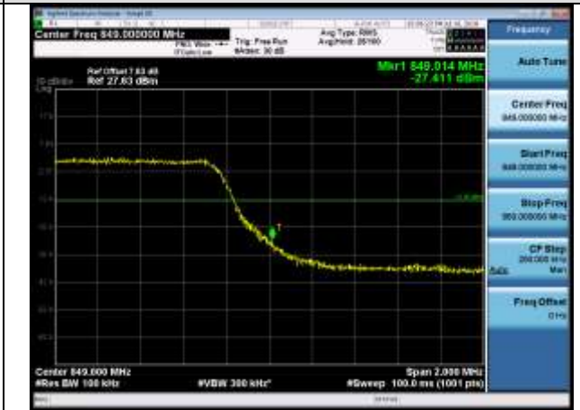
HCH_16QAM_25RB#0
