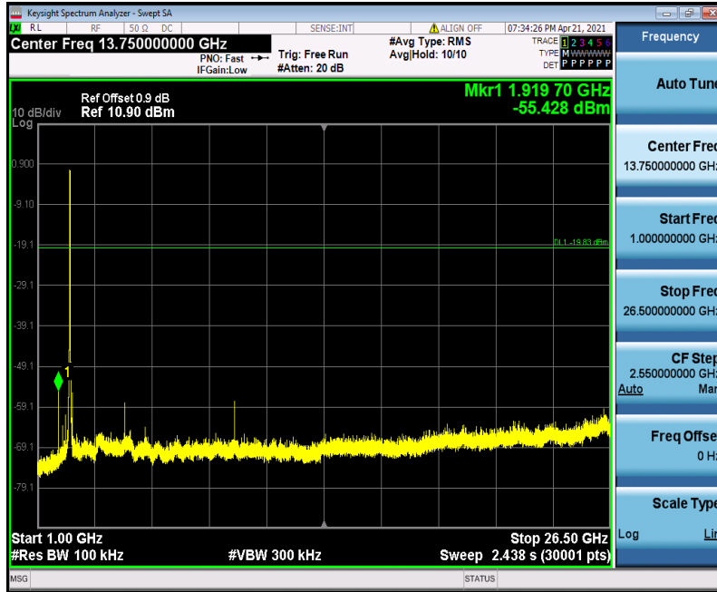
11G_Ant1_2462_0~Reference
