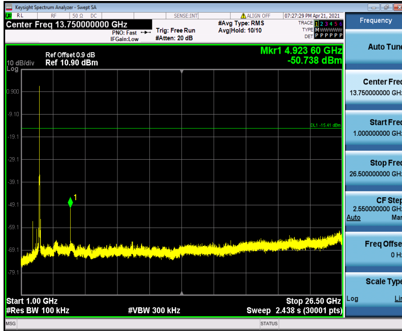
11G_Ant1_2412_0-Reference
