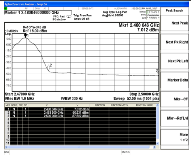
Channel 26 / 2480 MHz – Average
