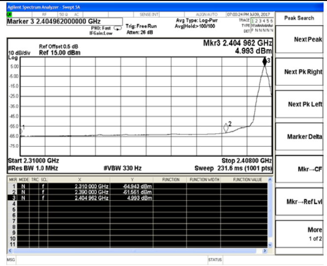
Channel 11 / 2405 MHz – Average
