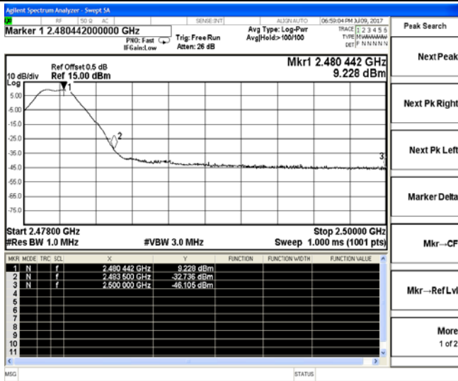
Channel 26 / 2480 MHz – Peak
