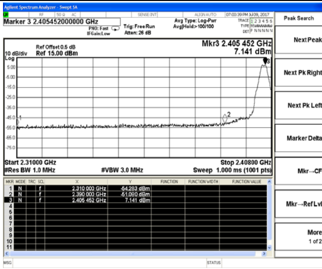
Channel 11 / 2405 MHz – Peak
