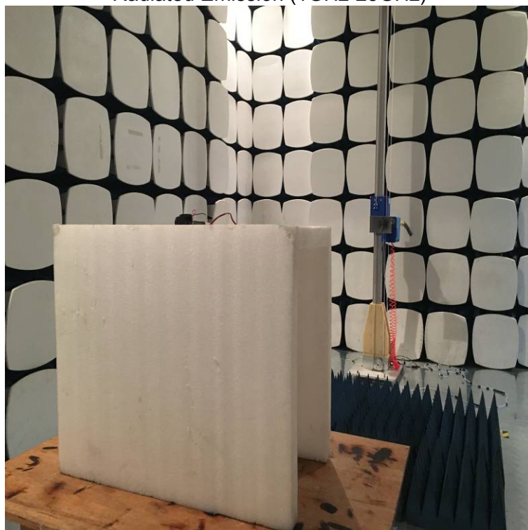
Radiated Emission (1GHz-25GHz)
