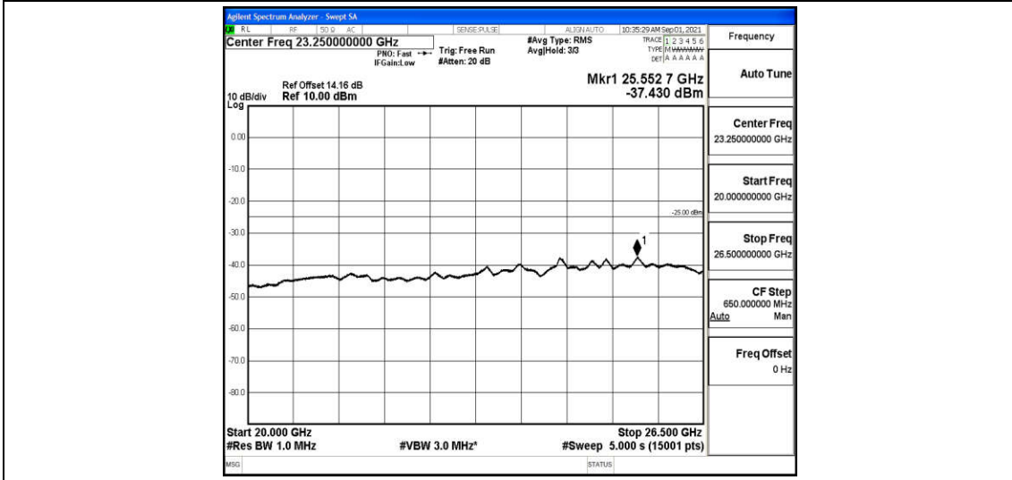
Band41-20MHz-16QAM-41490-1RB#0-Range6:20000~26500MHz
