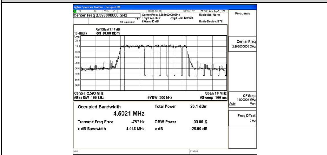
Band41-5MHz-16QAM-41565-25RB#0
