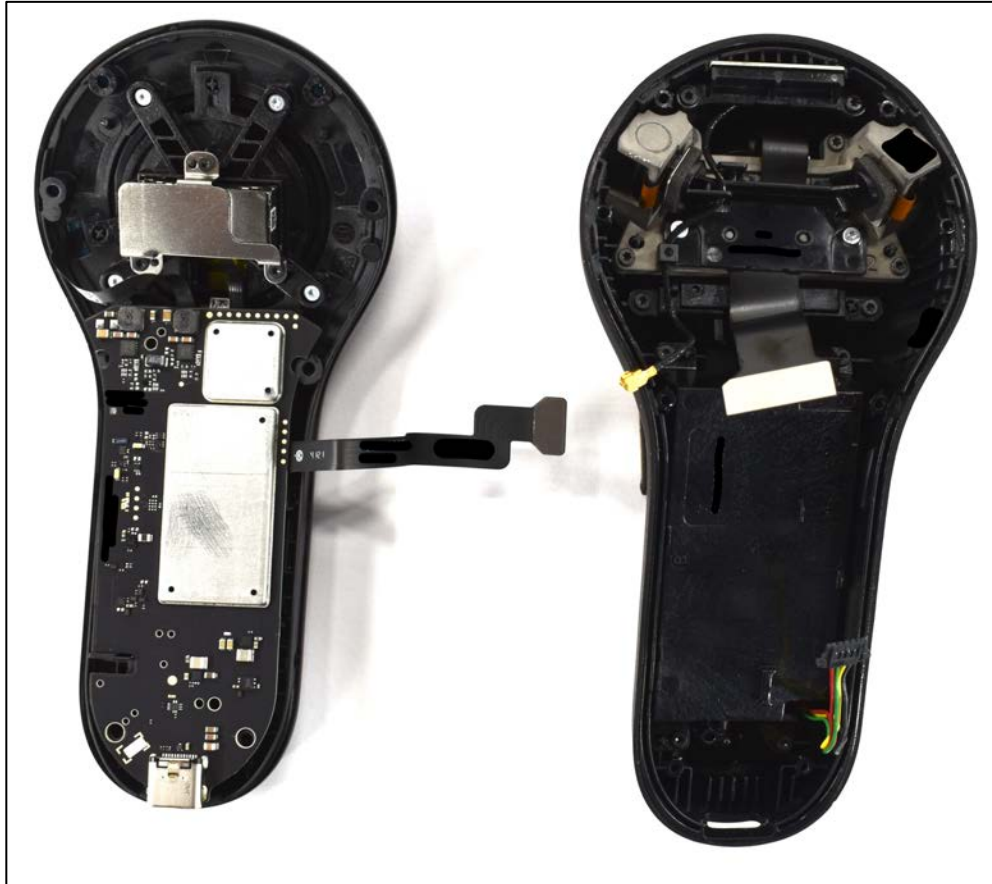
Figure 4: Controller – second layer before the battery compartment
