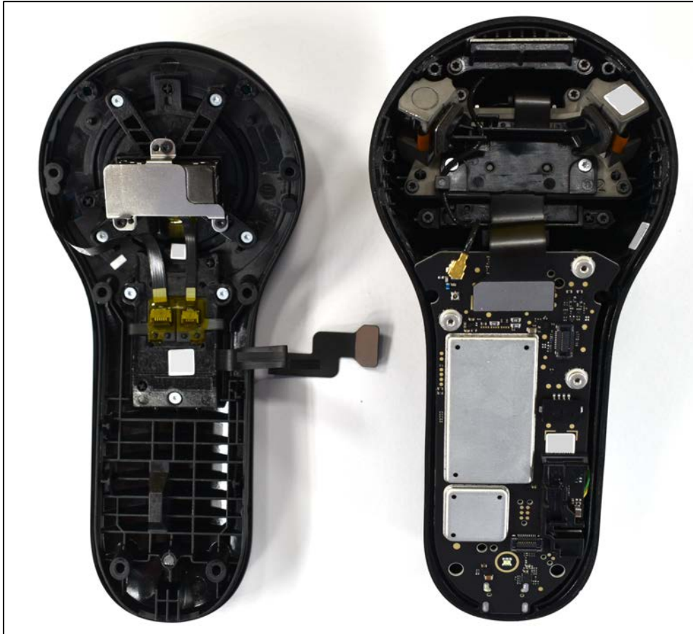
Figure 2: Controller – first layer below the top cover
