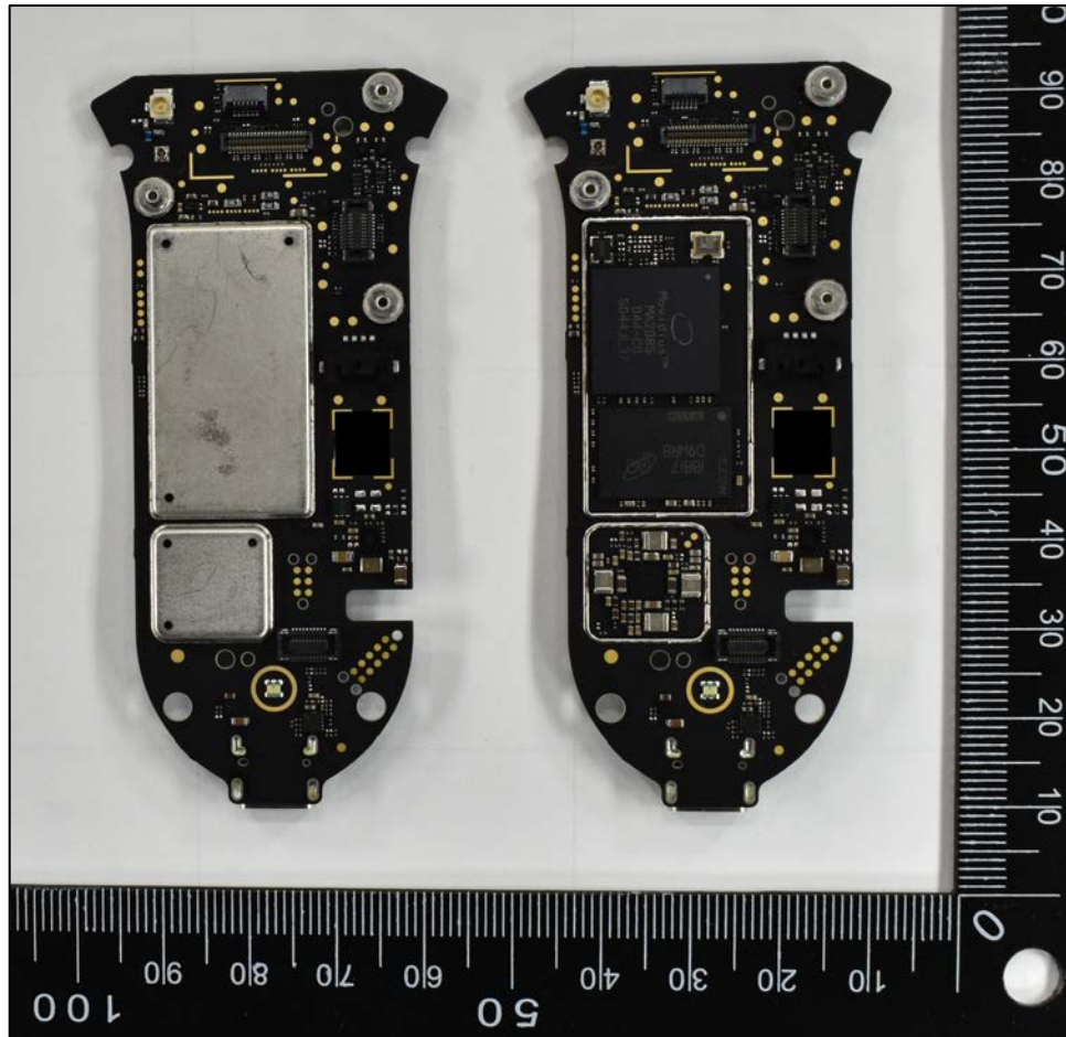
Figure 3: Controller – top PCB view, with and without shield
