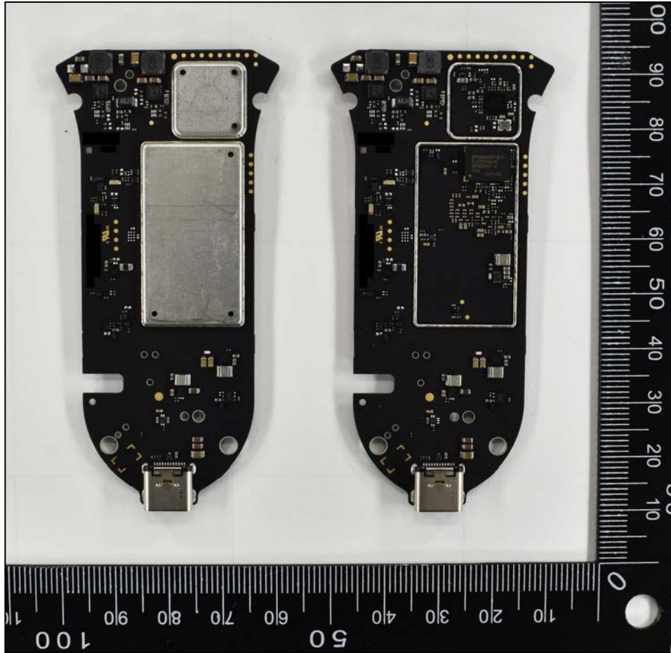
Figure 5: Controller – Bottom PCB view, with and without shield
