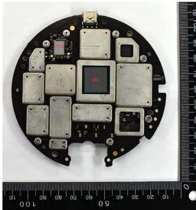
Figure 6: Compute Pack – Bottom PCB view w/o fan
