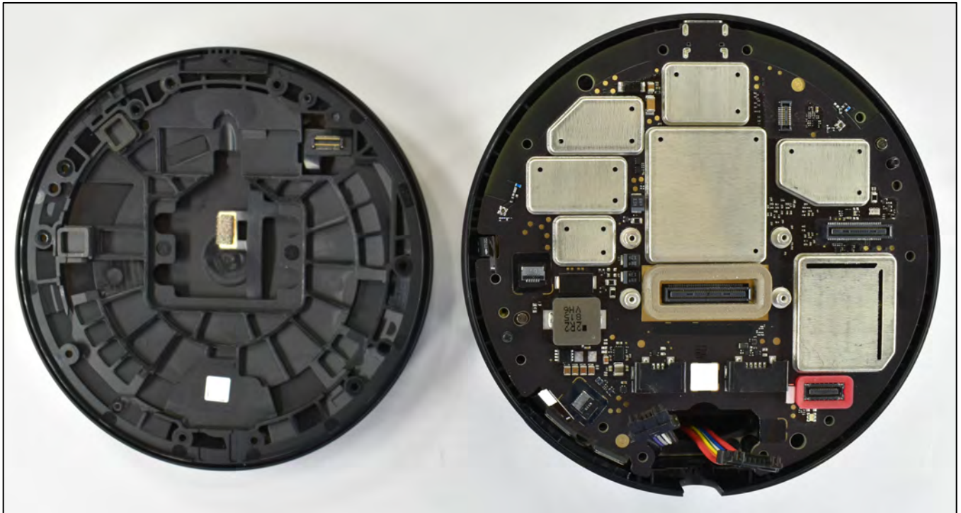
Figure 2: Compute Pack – Second layer below top cover
