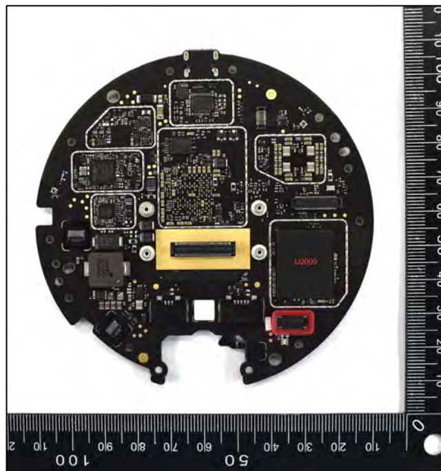
Figure 4: Compute Pack – Top PCB view w/o shield
