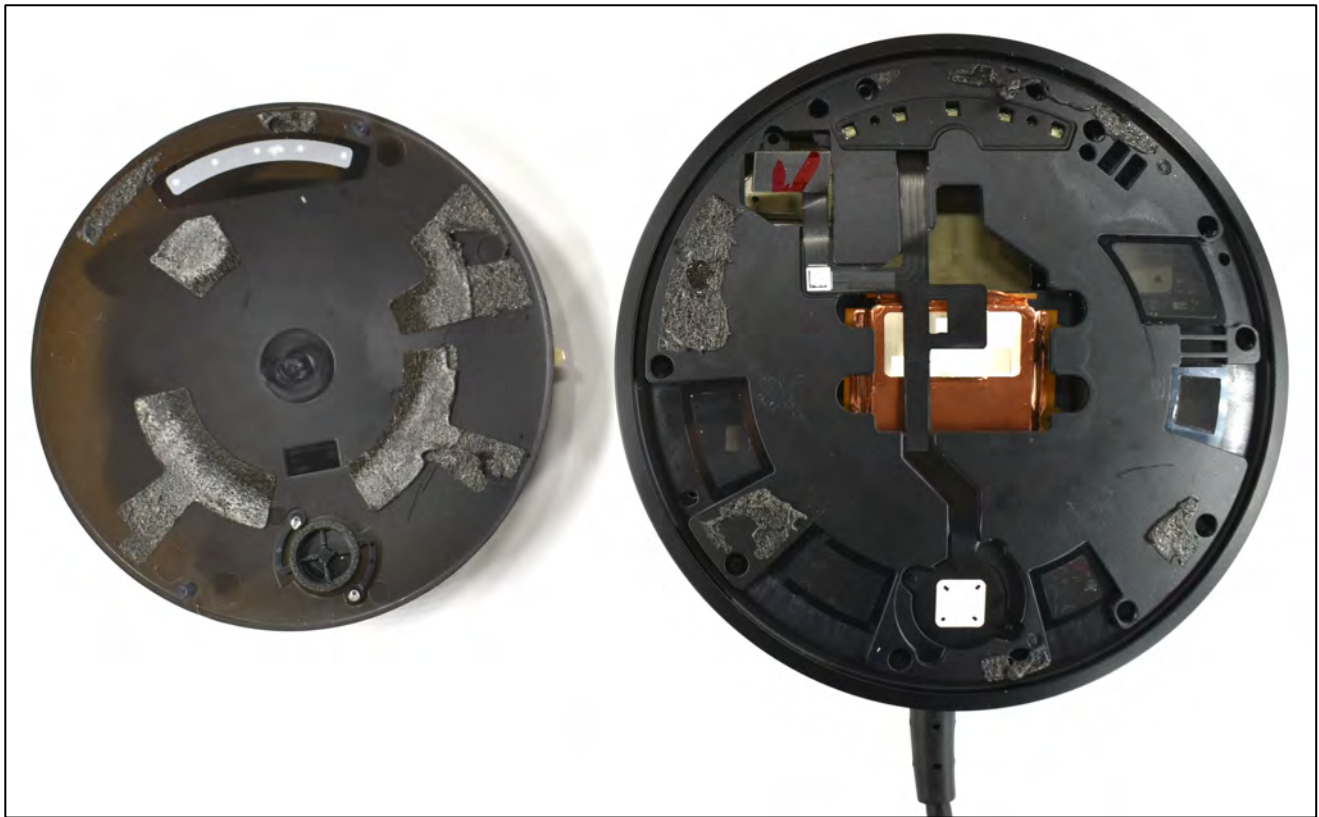
Figure 1: Compute Pack – First layer below top cover
