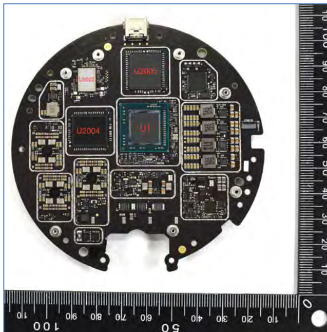
Figure 7: Compute Pack – Bottom PCB view w/o fan and shield
