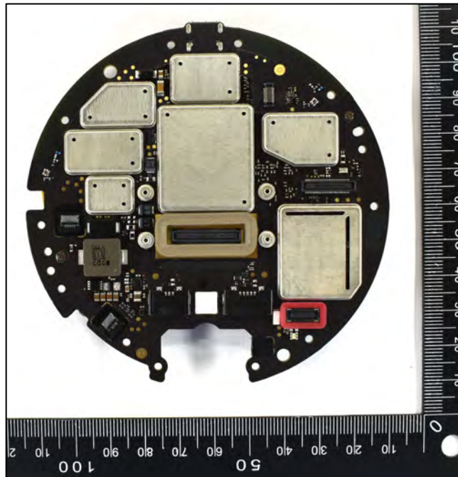
Figure 3: Compute Pack – Top PCB view w/ shield
