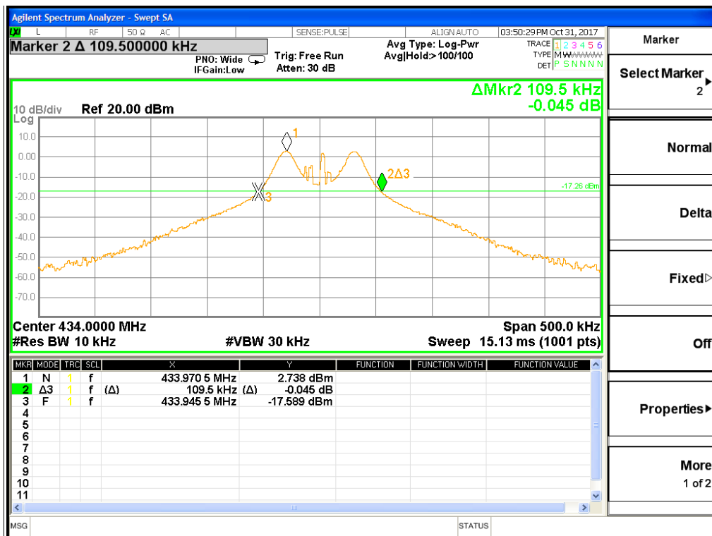
20dB Bandwidth
