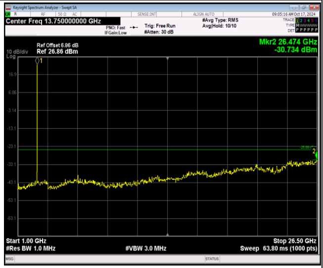
Band41-5MHz-64QAM-41215-1RB#0-Range2:1000~26500MHz
