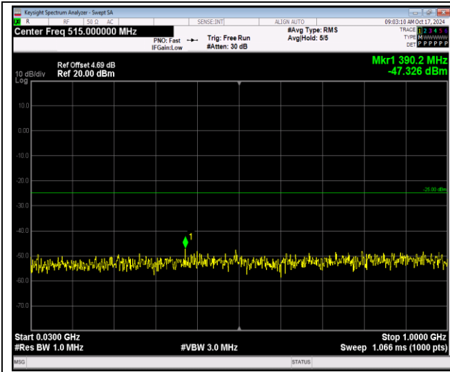
Band41-5MHz-64QAM-40740-1RB#0-Range1:30~1000MHz
