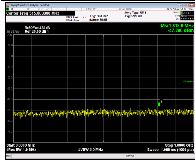
Band41-5MHz-16QAM-40265-1RB#0-Range1:30~10 00MHz
