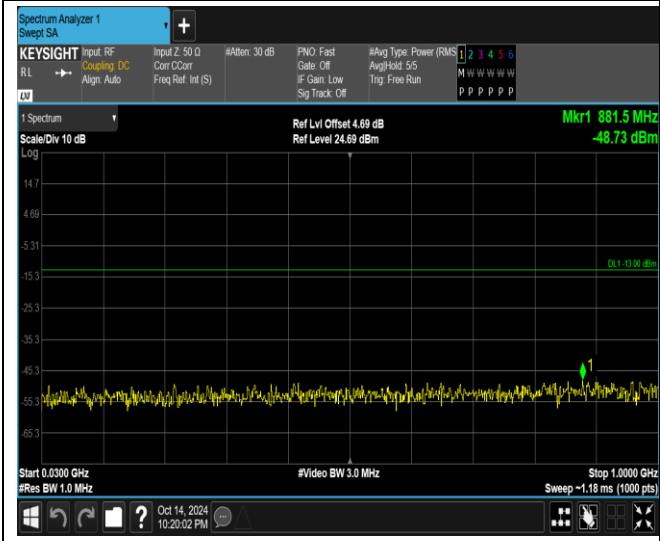
Band66-1.4MHz-16QAM-132665-1RB#0-Range1:30 ~1000MHz
