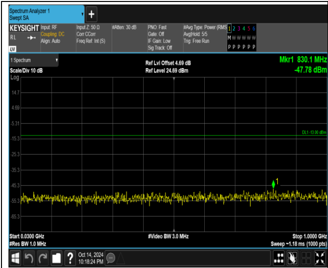
Band66-1.4MHz-16QAM-132322-1RB#0-Range1:30 ~1000MHz
