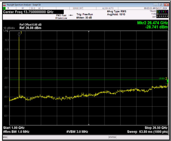
Band41-5MHz-64QAM-40740-1RB#0-Range2:1000~26500MHz
