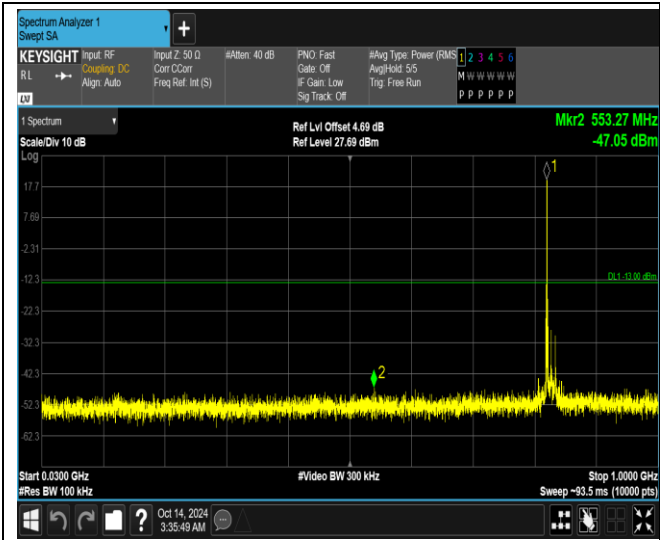
Band26-15MHz-QPSK-26915-1RB#0-Range1:30~1000MHz
