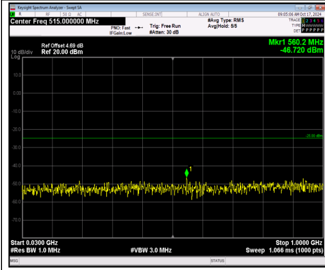
Band41-5MHz-64QAM-41215-1RB#0-Range1:30~1000MHz
