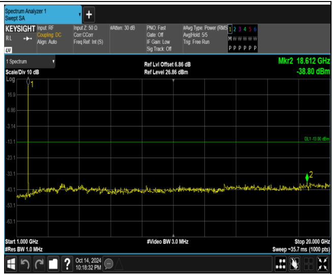
Band66-1.4MHz-16QAM-132322-1RB#0-Range2:10 00~20000MHz
