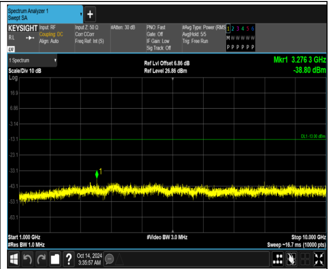
Band26-15MHz-QPSK-26915-1RB#0-Range2:1000~10000MHz
