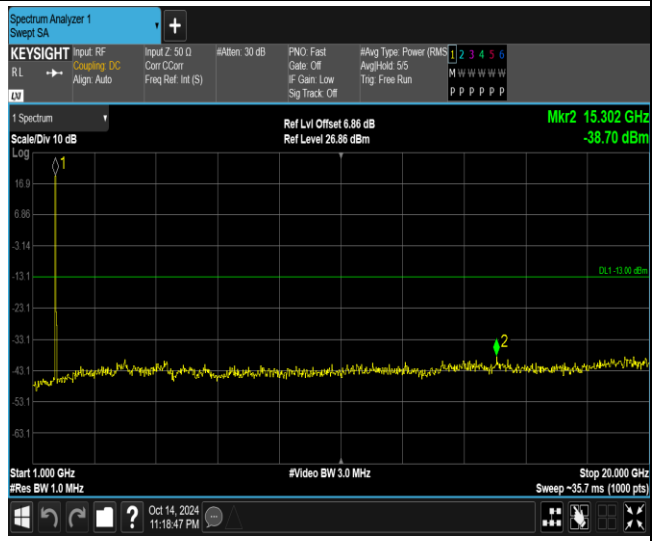
Band66-20MHz-64QAM-132072-1RB#0-Range2:1000~20000MHz
