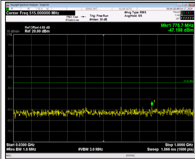
Band41-5MHz-16QAM-40265-1RB#0-Range1:30~10 00MHz
