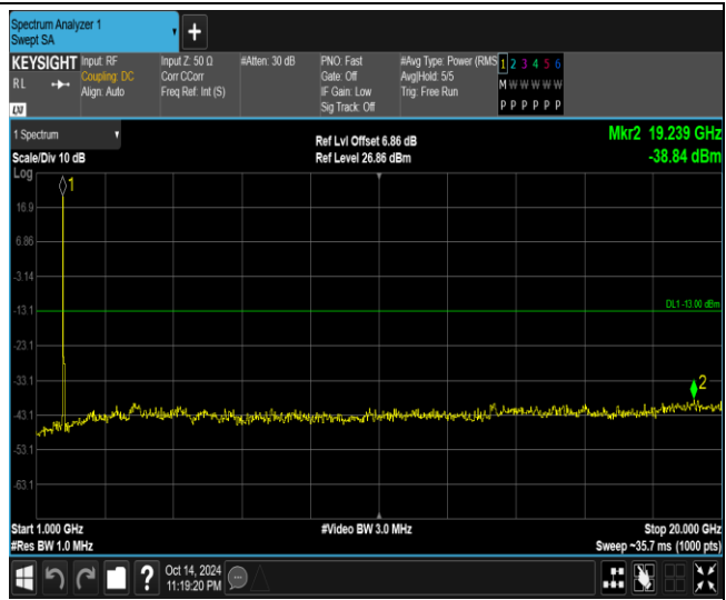
Band66-20MHz-16QAM-132572-1RB#0-Range2:1000~20000MHz
