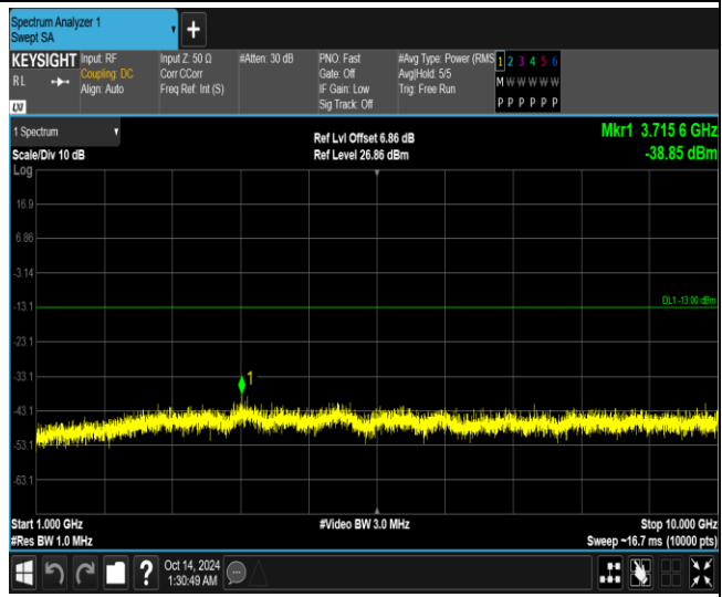
Band13-10MHz-16QAM-23230-1RB#0-Range2:1000~10000MHz
