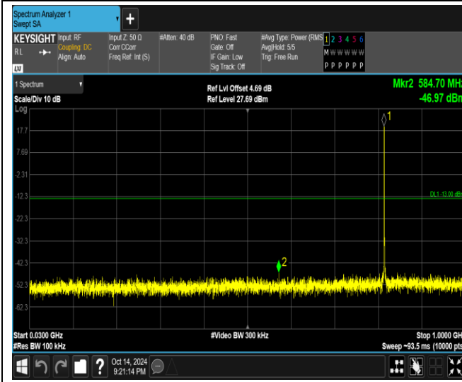
Band26-1.4MHz-16QAM-26783-1RB#0-Range1:30~1000MHz
