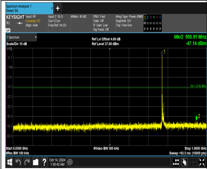
Band13-10MHz-16QAM-23230-1RB#0-Range1:30~1000MHz
