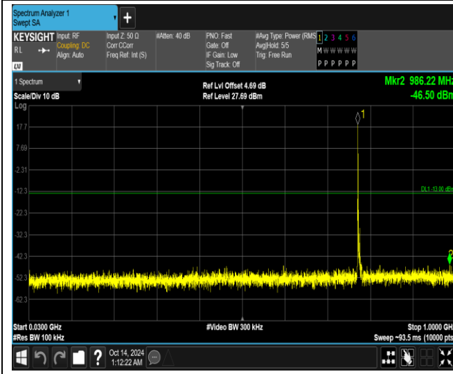
Band13-5MHz-QPSK-23205-1RB#0-Range1:30~1000MHz
