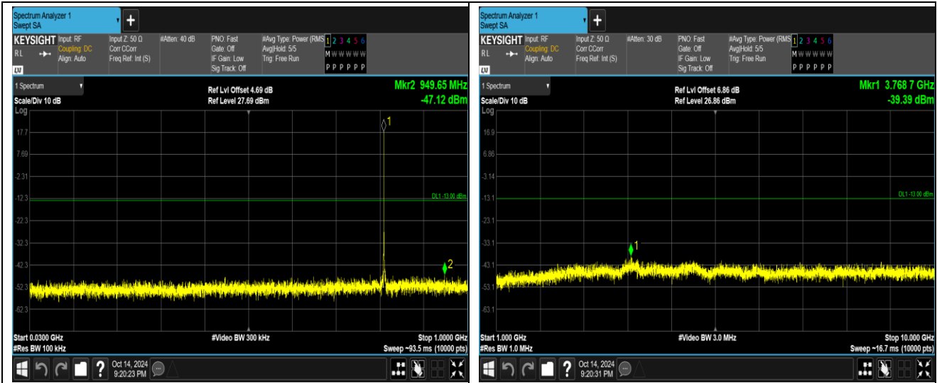
Band26-1.4MHz-16QAM-26740-1RB#0-Range1:30~1000MHz
