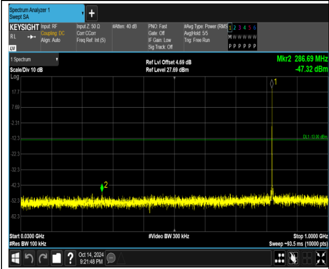
Band26-1.4MHz-QPSK-26797-1RB#0-Range1:30~1000MHz
