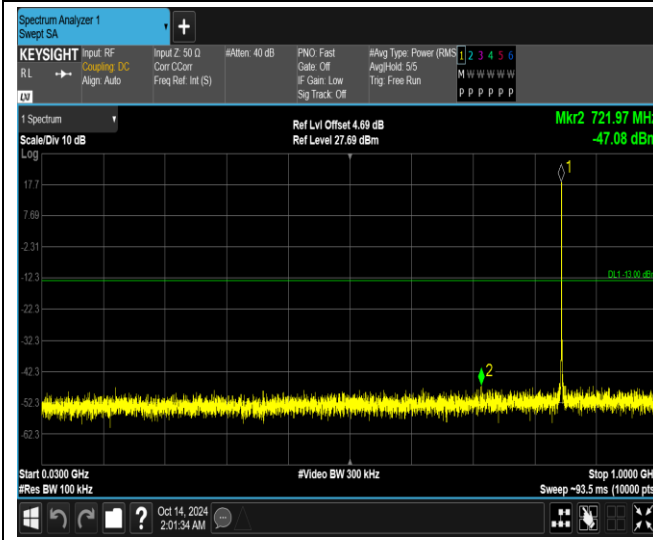
Band26-10MHz-QPSK-26740-1RB#0-Range1:30~1000MHz
