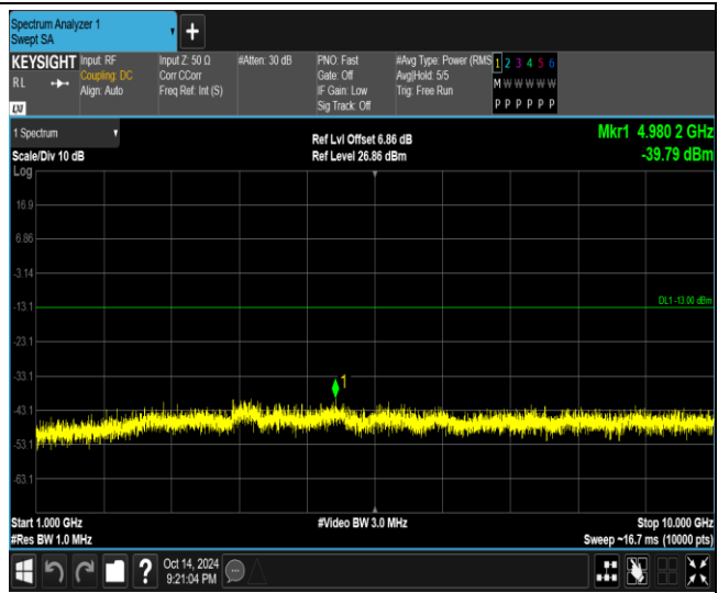
Band26-1.4MHz-QPSK-26783-1RB#0-Range2:1000~10000MHz
