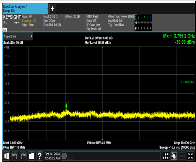
Band12-10MHz-16QAM-23060-1RB#0-Range2:1000~10000MHz
