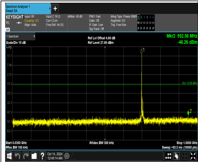
Band12-10MHz-16QAM-23060-1RB#0-Range1:30~1000MHz
