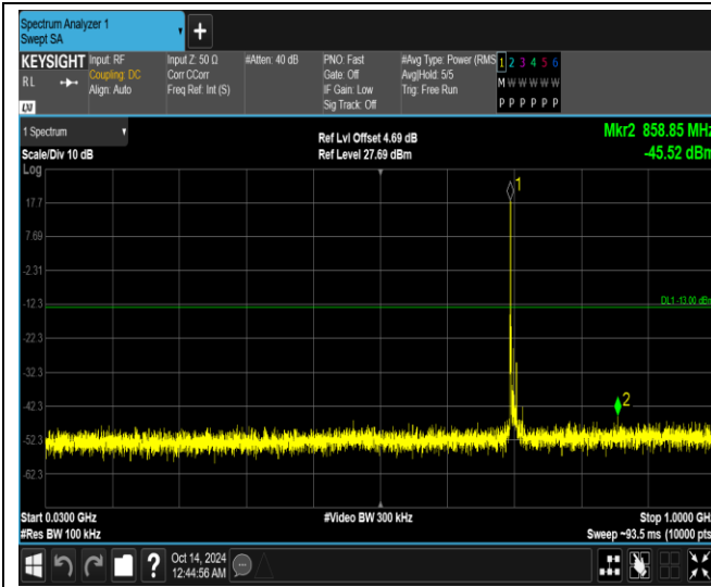
Band12-10MHz-64QAM-23130-1RB#0-Range1:30~1000MHz
