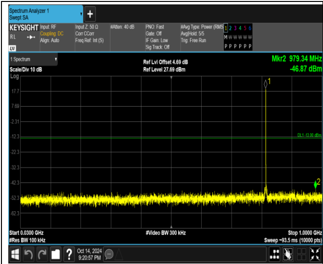
Band26-1.4MHz-QPSK-26783-1RB#0-Range1:30~1000MHz
