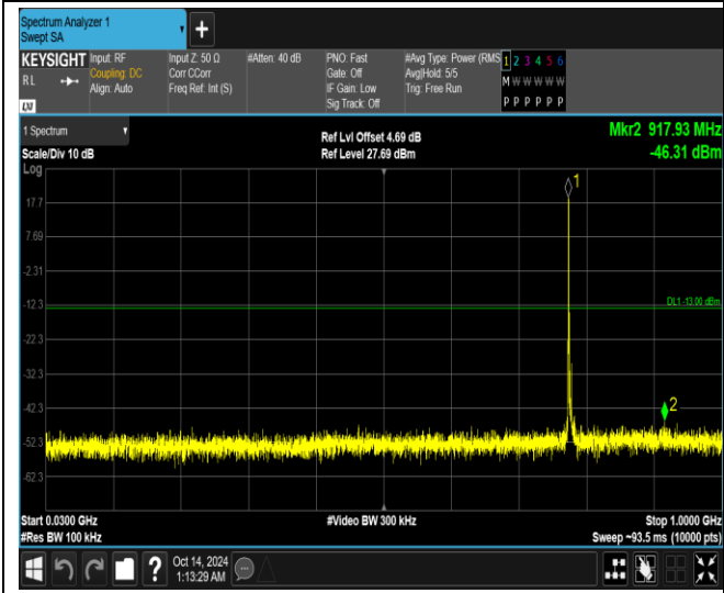
Band13-5MHz-16QAM-23255-1RB#0-Range1:30~1000MHz
