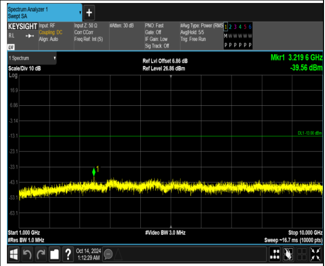
Band13-5MHz-QPSK-23205-1RB#0-Range2:1000~10000MHz
