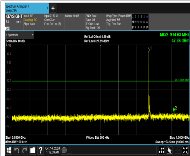
Band13-5MHz-16QAM-23230-1RB#0-Range1:30~1000MHz
