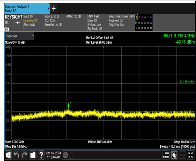
Band13-5MHz-16QAM-23230-1RB#0-Range2:1000~10000MHz
