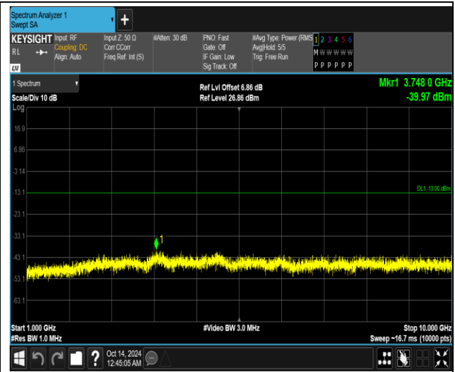
Band12-10MHz-64QAM-23130-1RB#0-Range2:1000~10000MHz
