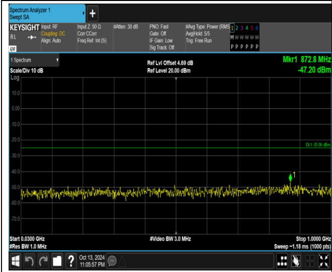
Band7-5MHz-QPSK-21100-1RB#0-Range1:30~1000 MHz
