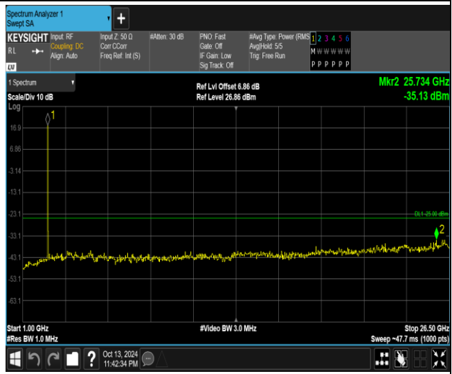
Band7-20MHz-64QAM-21100-1RB#0-Range2:1000~26500MHz
