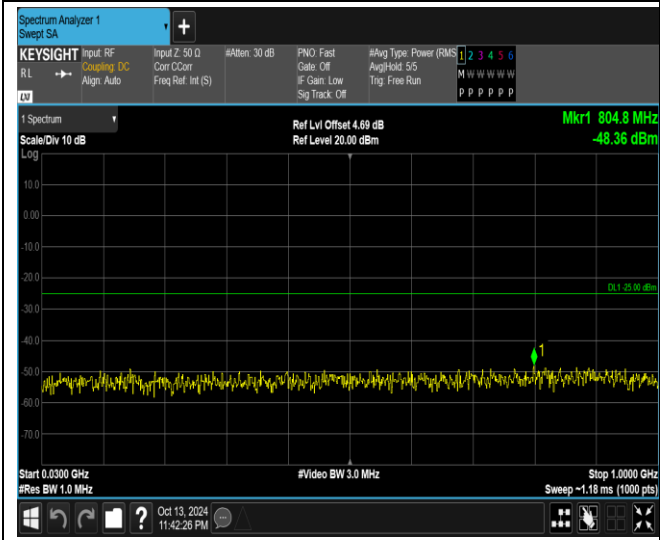
Band7-20MHz-64QAM-21100-1RB#0-Range1:30~1000MHz
