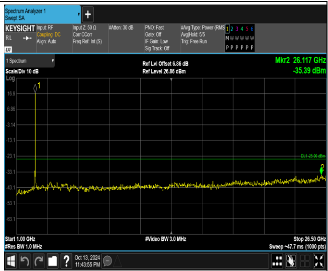
Band7-20MHz-64QAM-20850-1RB#0-Range2:1000~26500MHz
