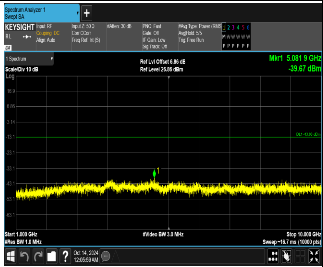
Band12-1.4MHz-64QAM-23173-1RB#0-Range2:1000~10000MHz
