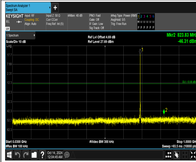
Band12-1.4MHz-16QAM-23017-1RB#0-Range1:30~1000MHz
