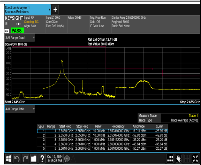
Band41-5MHz-64QAM-41215-25RB#0
