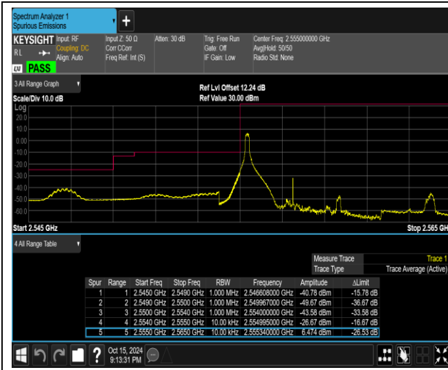
Band41-5MHz-64QAM-40265-25RB#0
