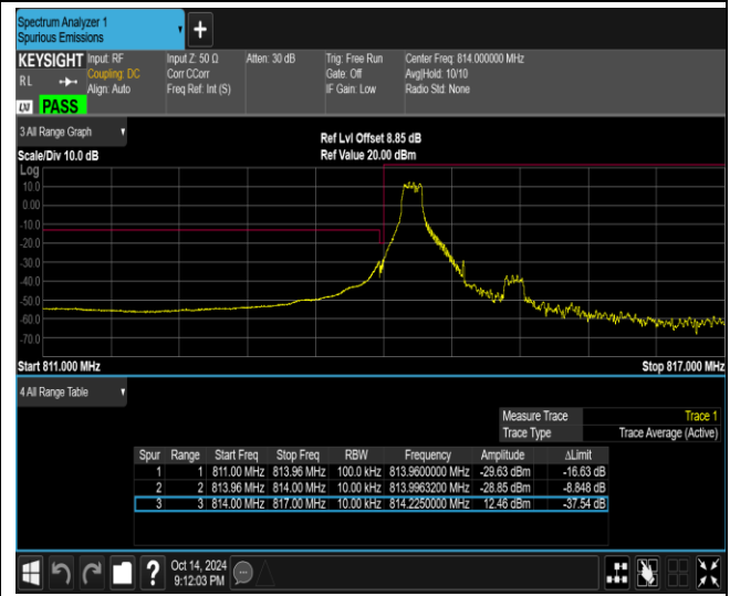
Band26-1.4MHz-QPSK-26697-6RB#0
