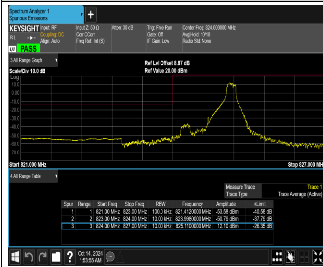
Band26-1.4MHz-QPSK-27033-1RB#0
