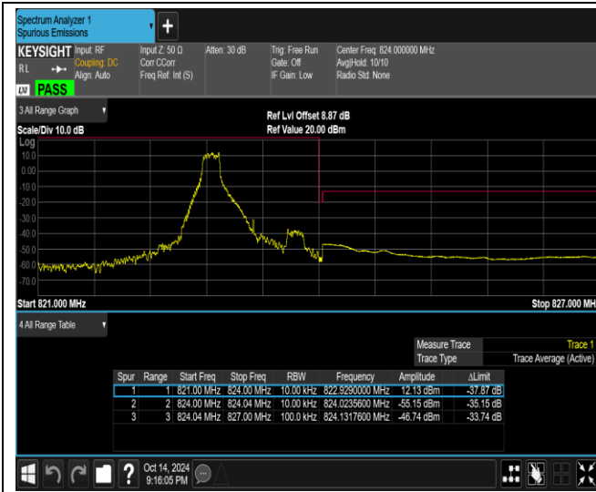
Band26-1.4MHz-QPSK-26783-6RB#0
