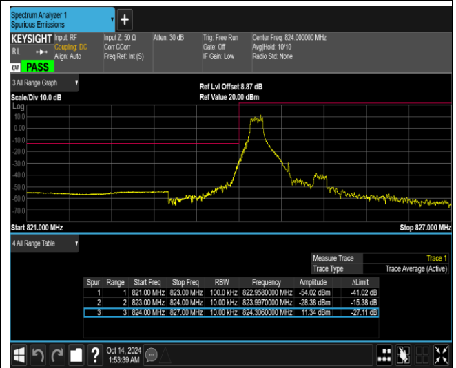
Band26-1.4MHz-64QAM-26797-6RB#0
