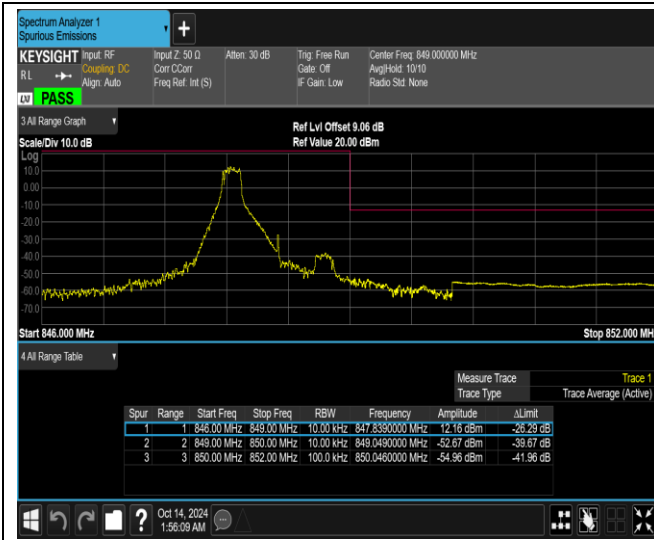
Band26-1.4MHz-QPSK-27033-6RB#0
