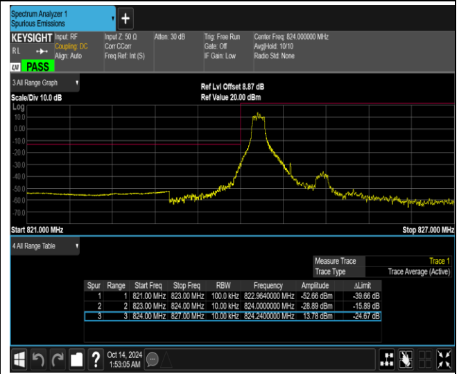
Band26-1.4MHz-QPSK-26797-6RB#0
