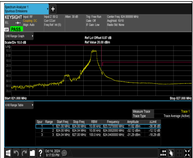
Band26-1.4MHz-16QAM-26797-1RB#0
