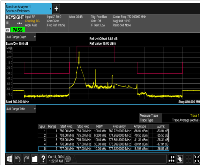
Band13-10MHz-64QAM-23230-50RB#0
