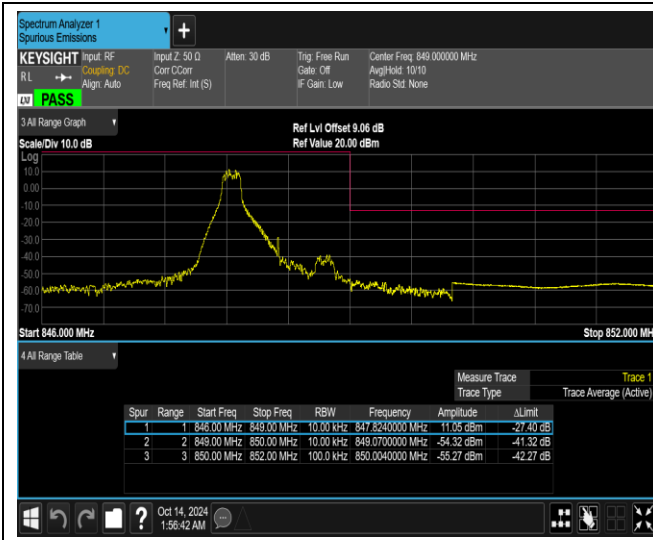
Band26-1.4MHz-64QAM-27033-6RB#0
