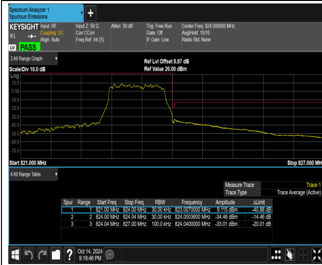
Band26-1.4MHz-QPSK-26797-1RB#5
