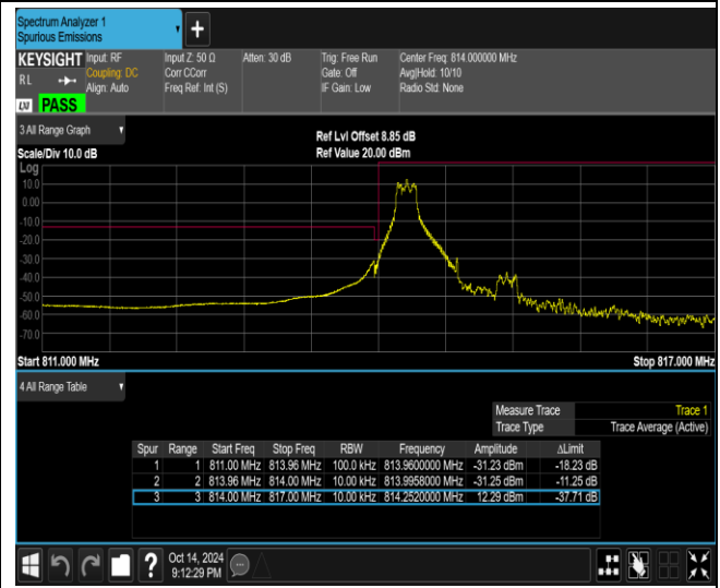
Band26-1.4MHz-16QAM-26697-6RB#0
