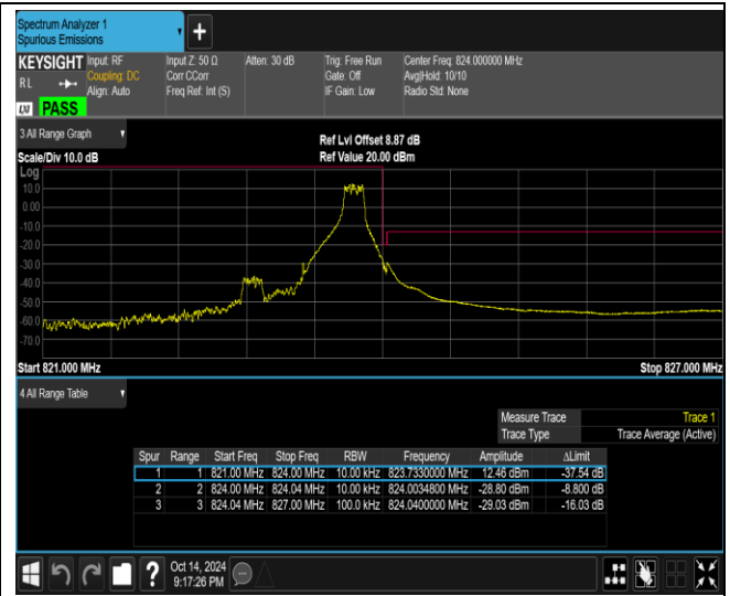
Band26-1.4MHz-QPSK-26797-1RB#0
