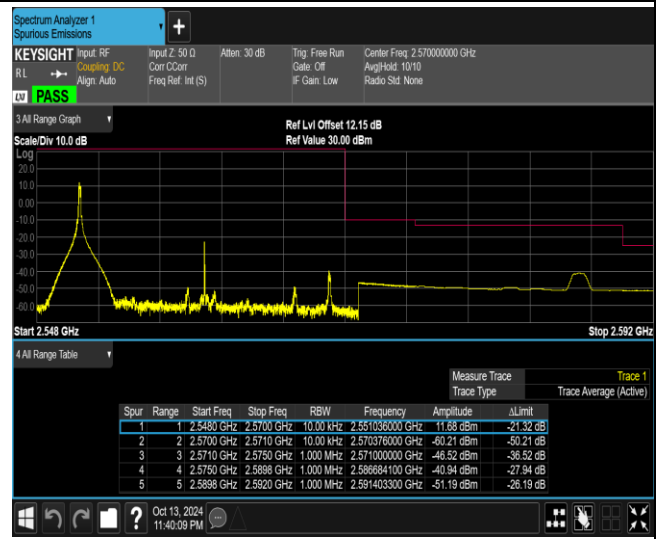
Band7-20MHz-64QAM-21350-100RB#0
