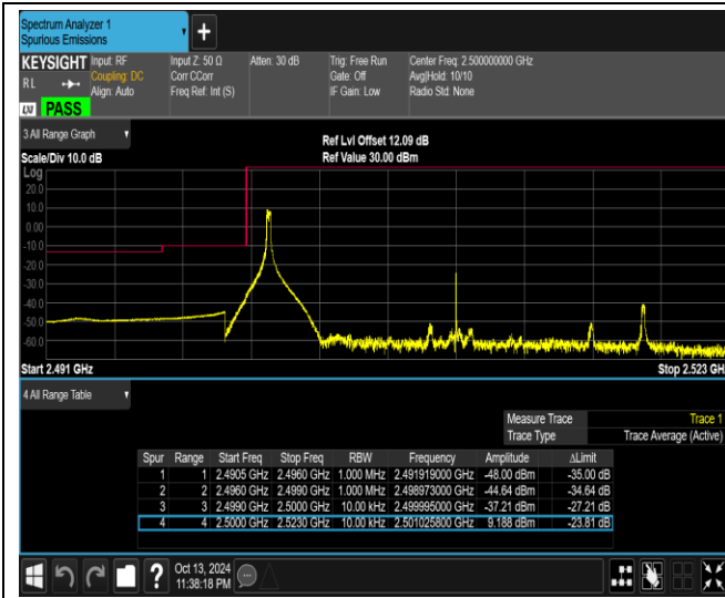
Band7-20MHz-64QAM-20850-100RB#0
