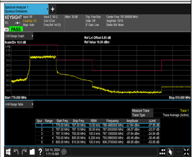
Band13-5MHz-64QAM-23205-1RB#24
