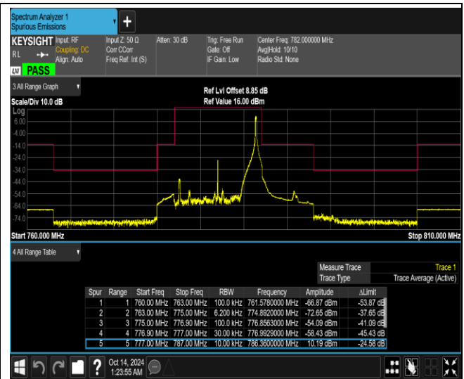
Band13-10MHz-16QAM-23230-1RB#0
