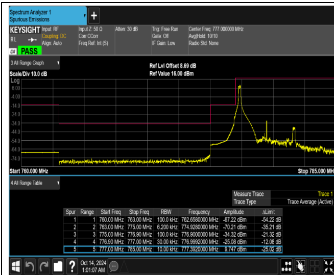
Band13-5MHz-16QAM-23205-25RB#0
