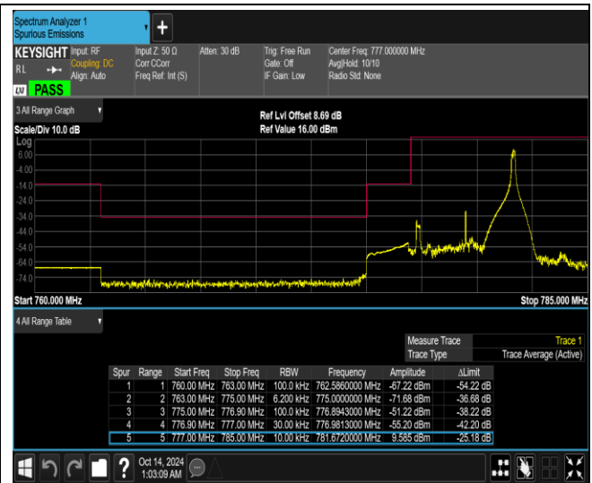
Band13-5MHz-16QAM-23255-1RB#0
