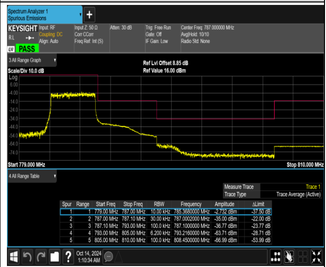
Band13-5MHz-16QAM-23205-1RB#24
