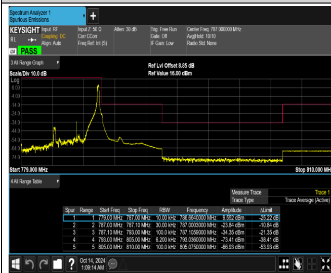
Band13-5MHz-64QAM-23205-1RB#0
