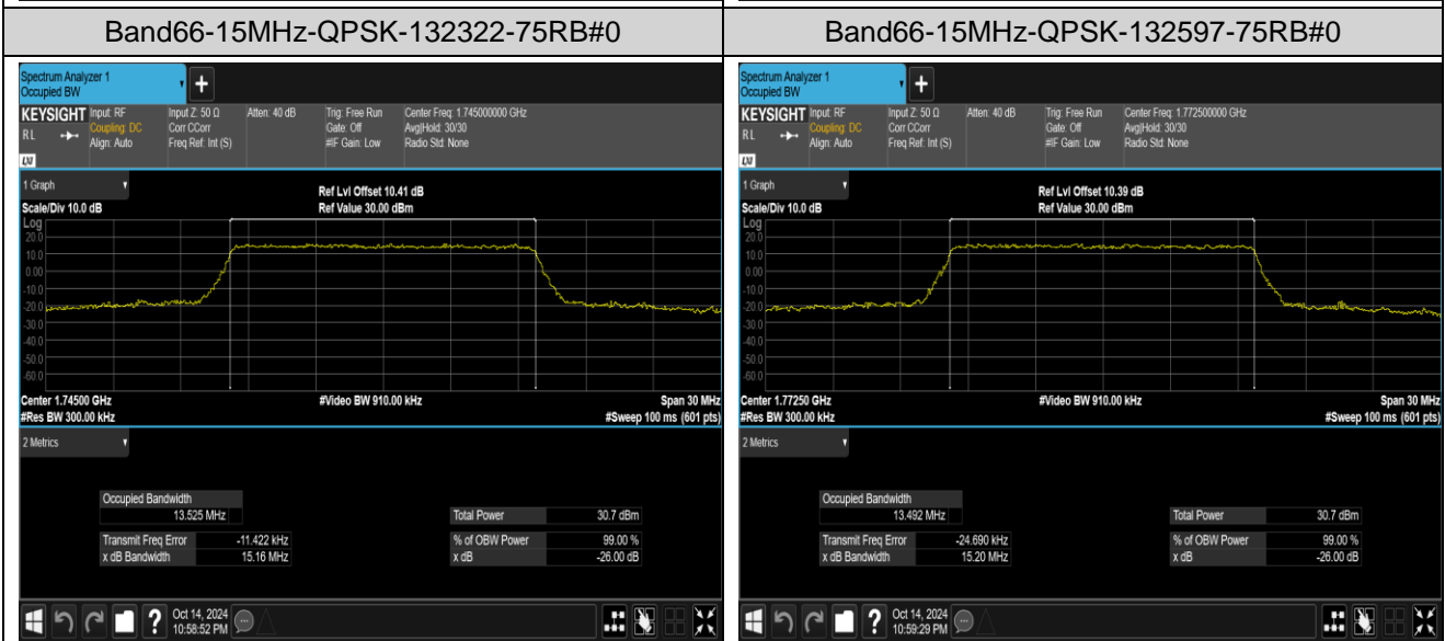
Band66-15MHz-16QAM-132047-75RB#0 Band66-15MHz-16QAM-132322-75RB#0
