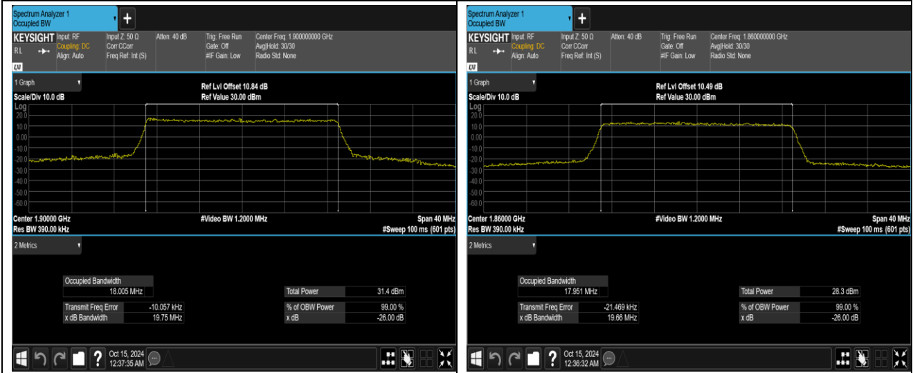
Band2-20MHz-64QAM-18900-100RB#0
