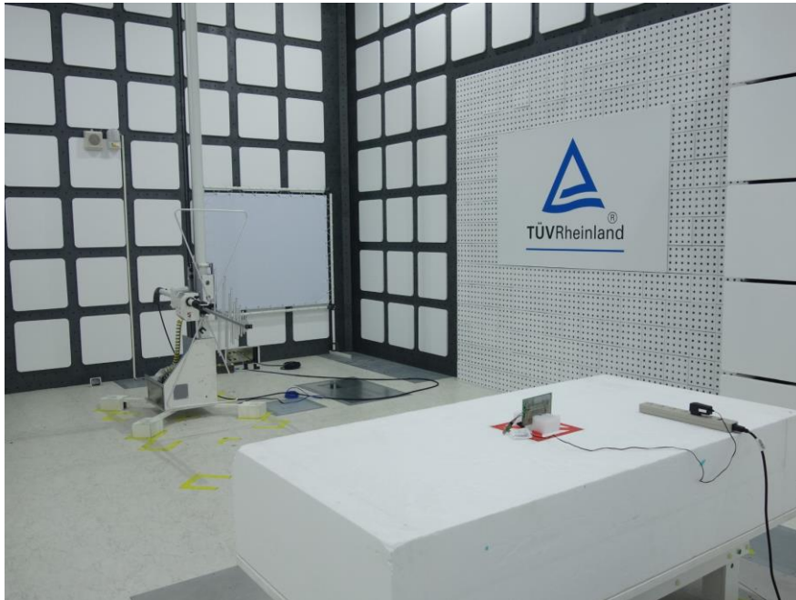
Photograph 11: Set-up for Spurious Emissions (Back View 1, 37130-AKD3)
