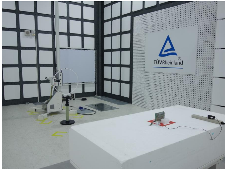
Photograph 4: Set-up for Spurious Emissions (Back View 2, 37130-AGJ5)
