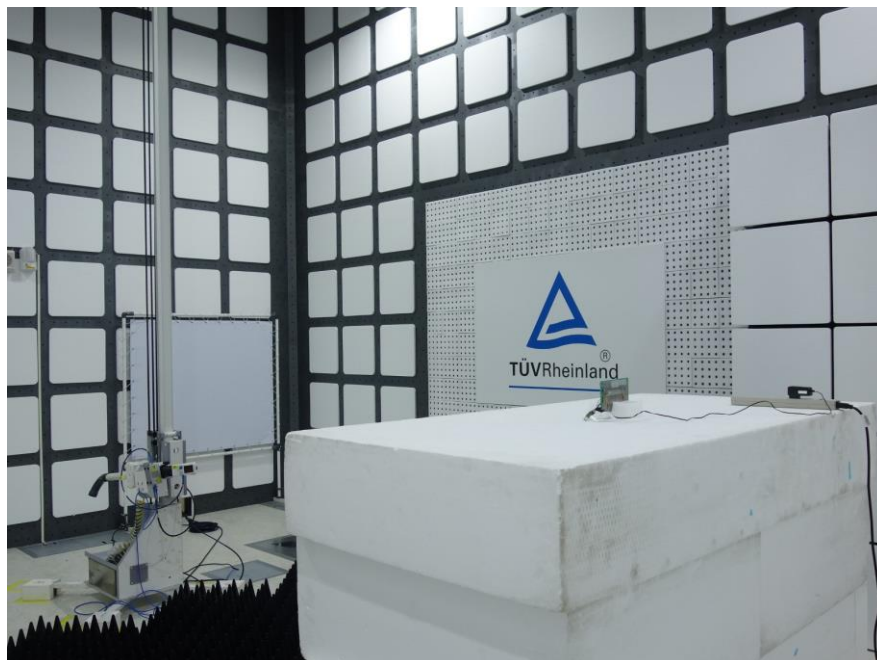
Photograph 14: Set-up for Spurious Emissions (Back View 4, 37130-AKD3)
