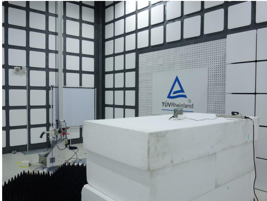
Photograph 13: Set-up for Spurious Emissions (Back View 3, 37130-AKD3)
