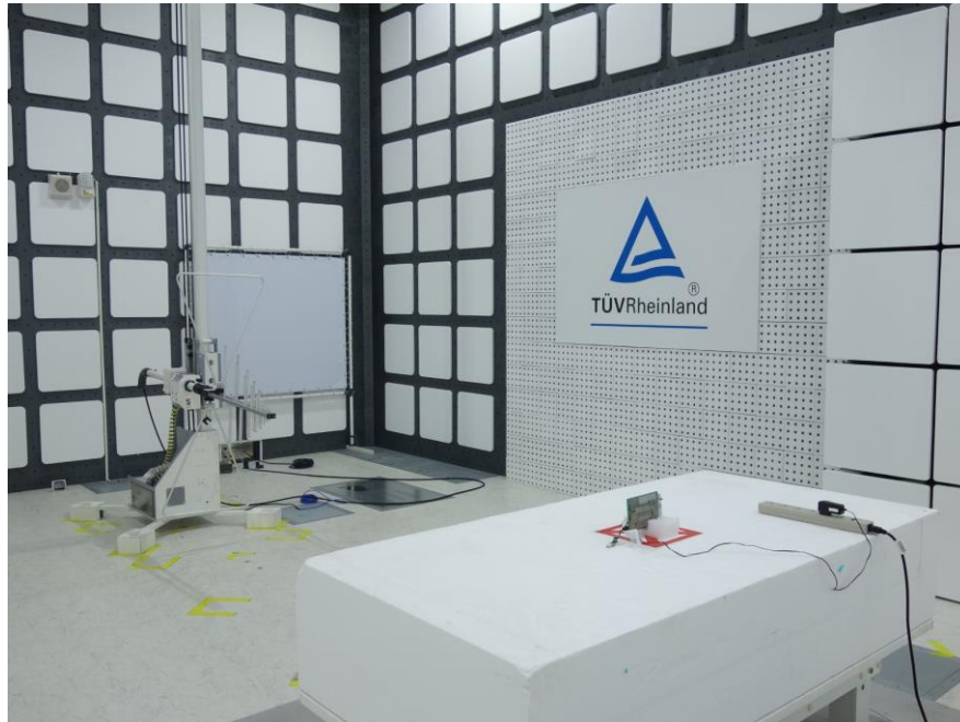
Photograph 3: Set-up for Spurious Emissions (Back View 1, 37130-AGJ5)
