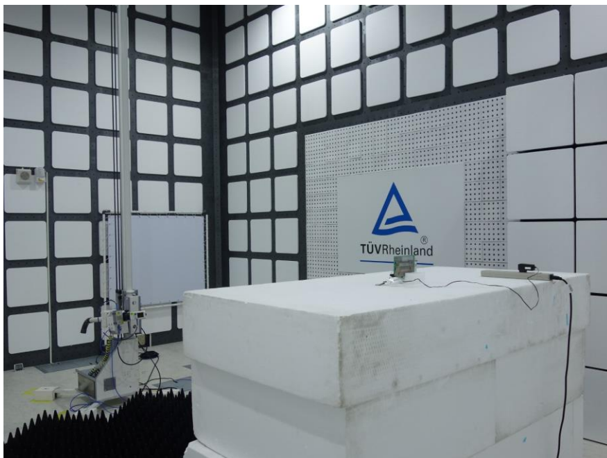
Photograph 6: Set-up for Spurious Emissions (Back View 4, 37130-AGJ5)
