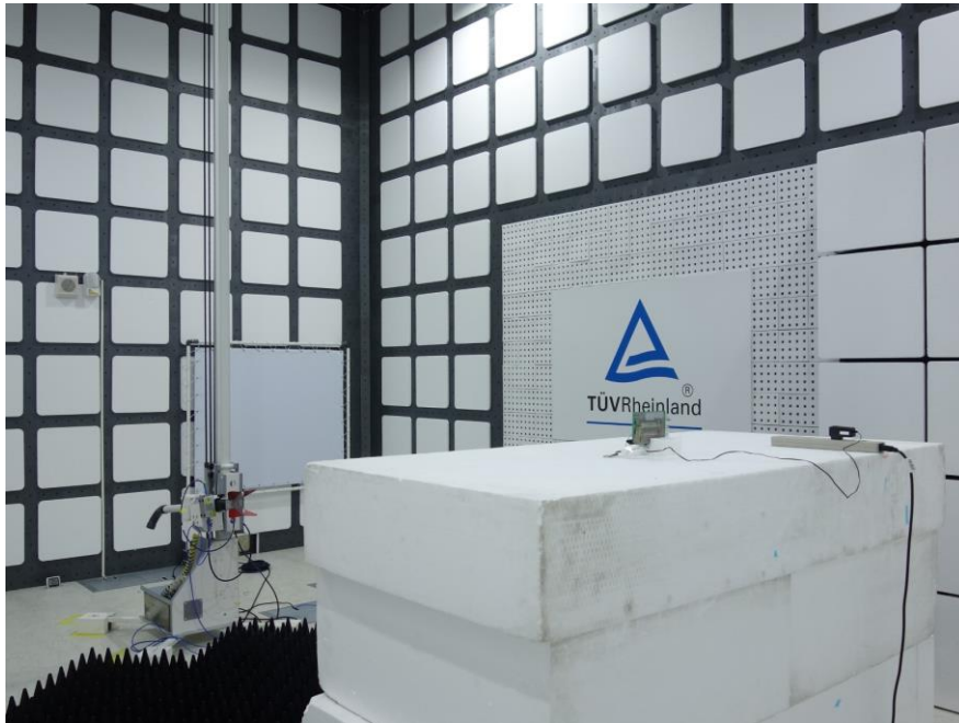
Photograph 5: Set-up for Spurious Emissions (Back View 3, 37130-AGJ5)
