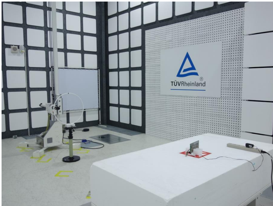
Photograph 12: Set-up for Spurious Emissions (Back View 2, 37130-AKD3)
