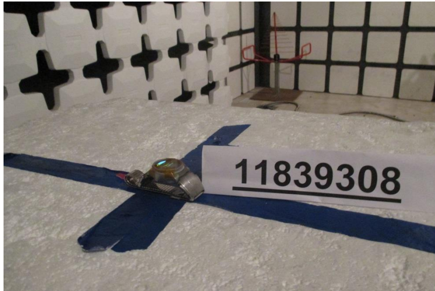
X-AXIS PHOTO
