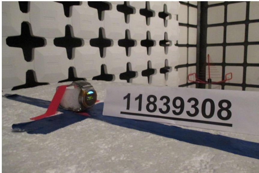
Y-AXIS PHOTO
