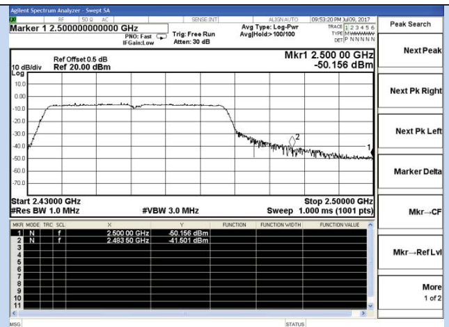
Channel 11 / 2452 MHz – Peak
