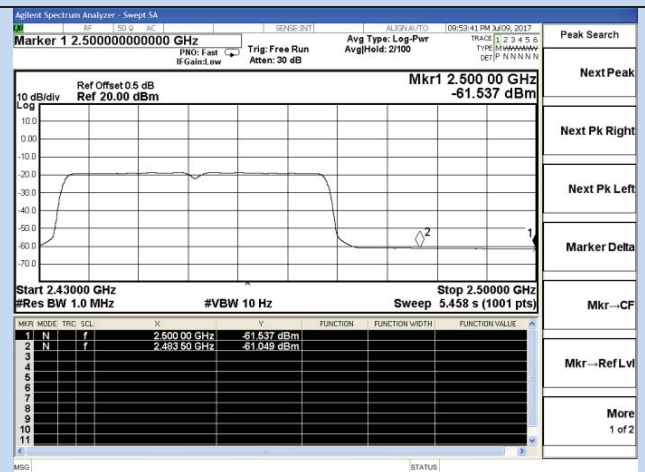
Channel 11 / 2452 MHz – Average
