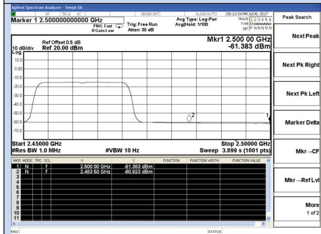
Channel 1 / 2462 MHz – Average
