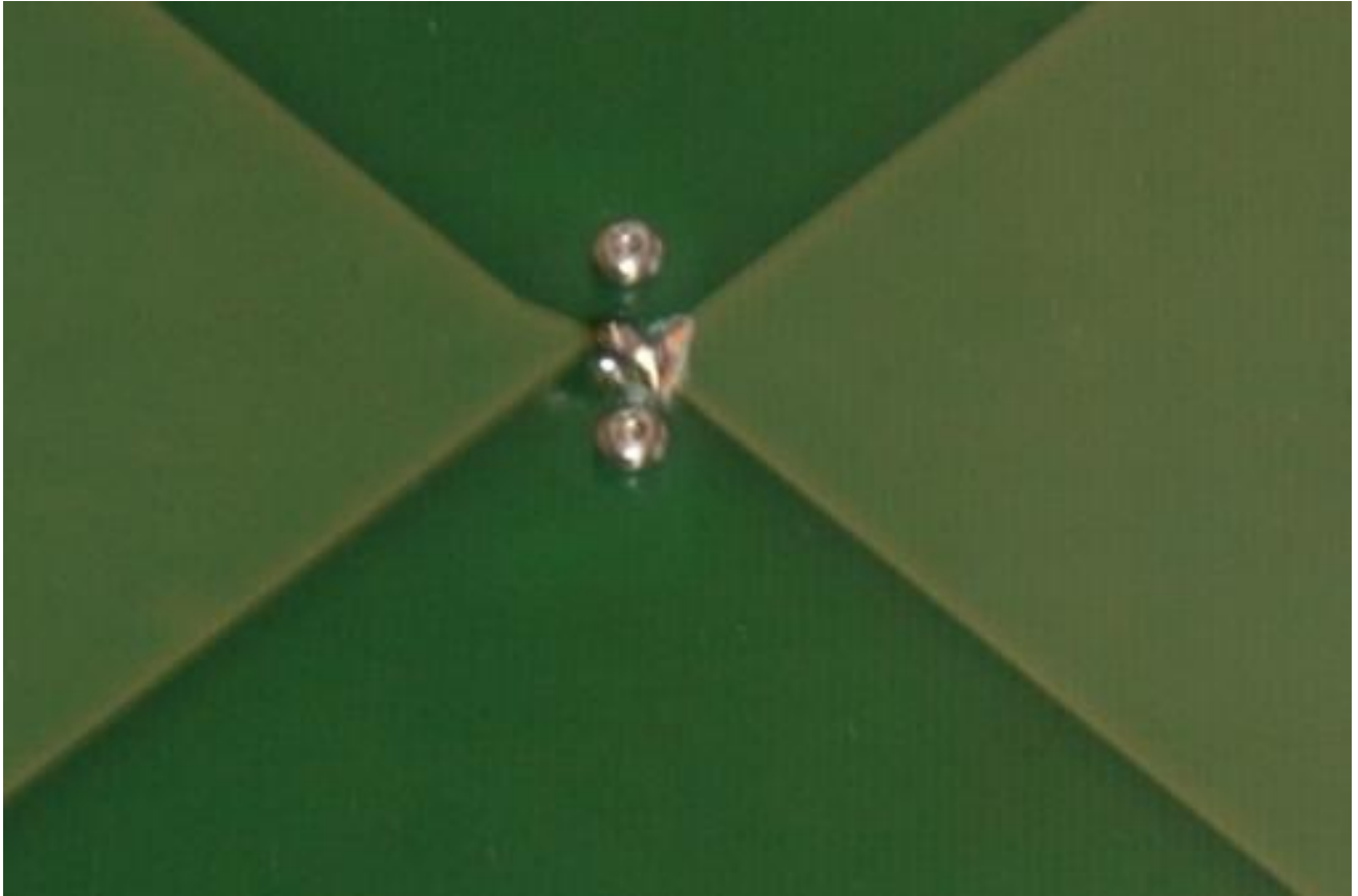
Modification with capacitor across antenna flares
