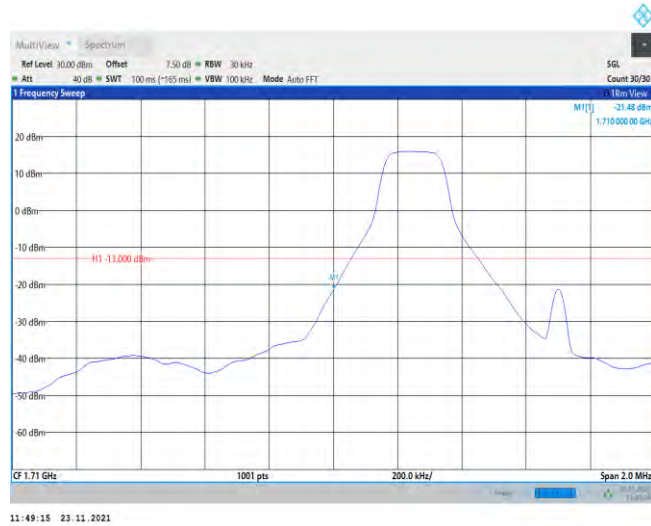
Band66-1.4MHz-QPSK-131979-6RB#0
