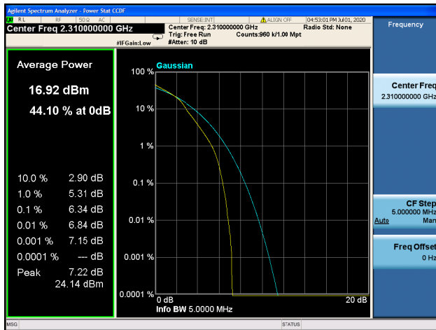
Band30 / 5MHz / Mid CH / 64QAM
