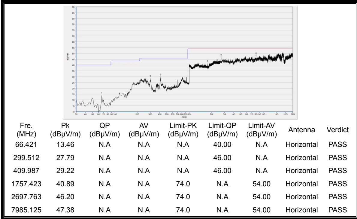
(30MHz to 25GHz, Antenna Horizontal @ GFSK, channel 0)
