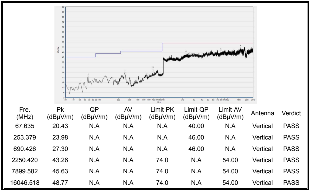
(30MHz to 25GHz, Antenna Vertical @ π/4-DQPSK, channel 78)
