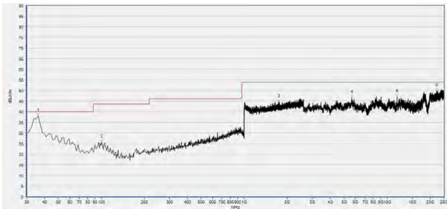
(30MHz to 25GHz, Antenna Horizontal, 8-DPSK, channel 0)
